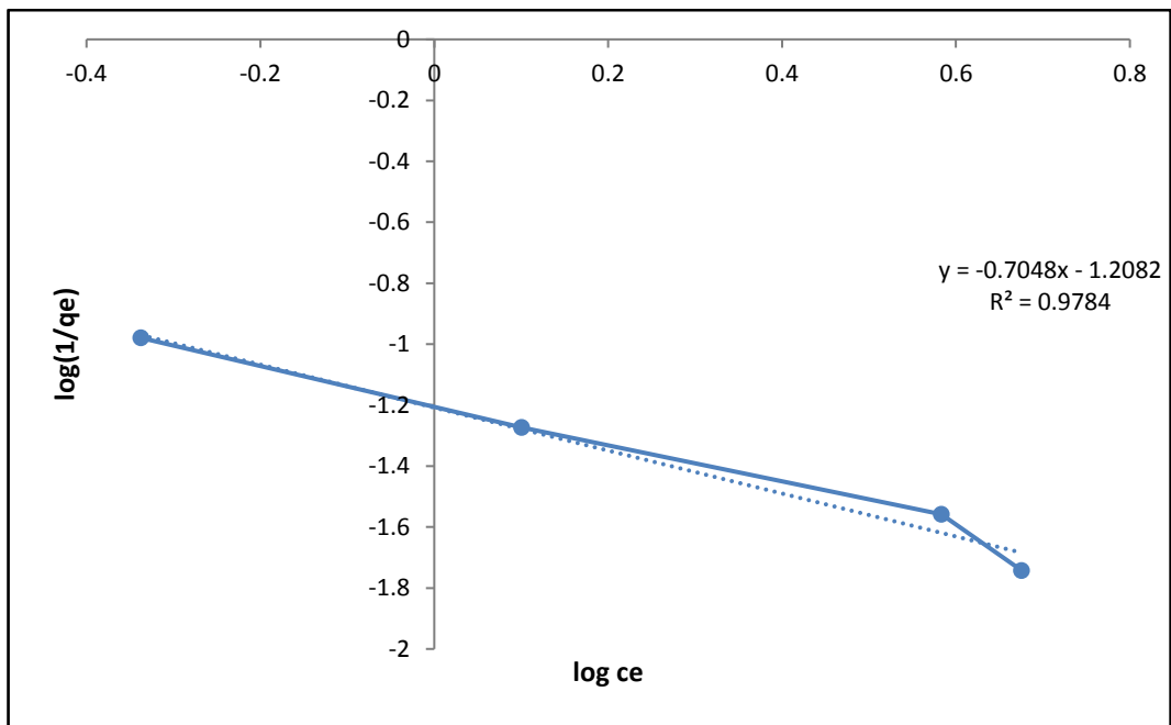
Figure 26: Sips Adsorption Isotherm with Plot of \log(1/q_e) vs \log c_e and R^2 0.9784
