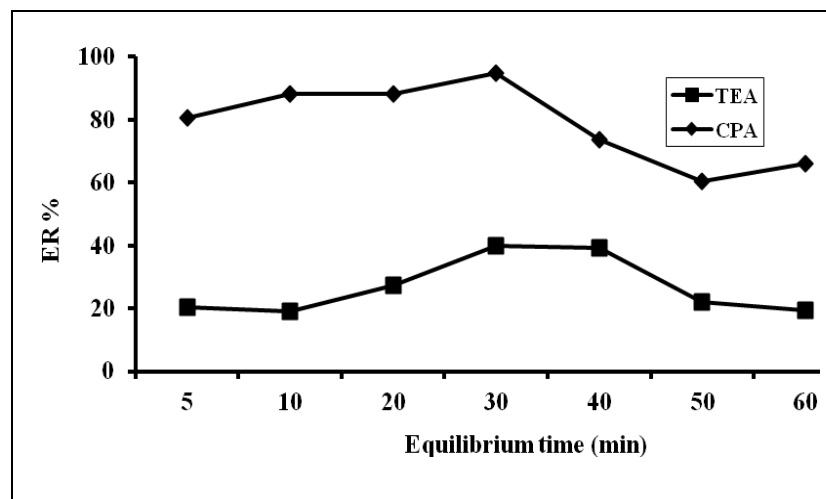
Figure 3.18 Effect of equilibration time on CPA and TEA extraction. Extraction conditions: synthetic sample solution, 2 mL; pH 2; volume of 4%w/v Triton X-114, 2 mL; volume of 1%w/v \text{KNO}_3 , 2 mL; T_{\text{eq}} 50 °C
