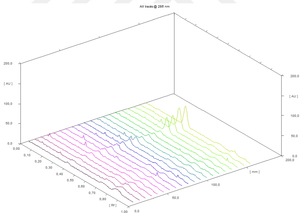
Figure 2.2 The HPTLC densitogram of standard HMF
