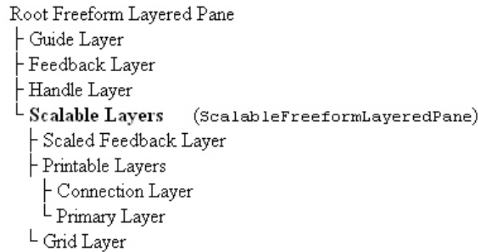
Figure 3.7: Layers in GEF
