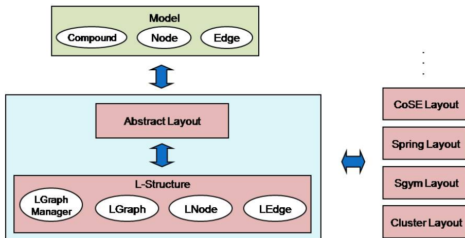
Figure 5.3: CHISIO Layout Architecture
