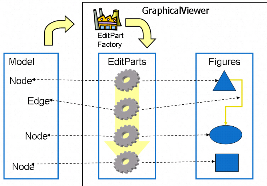
Figure 3.3: Chisio system architecture
