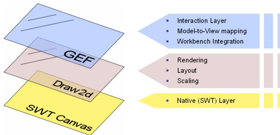
Figure 1.8: GEF is on top of Draw2d and SWT
