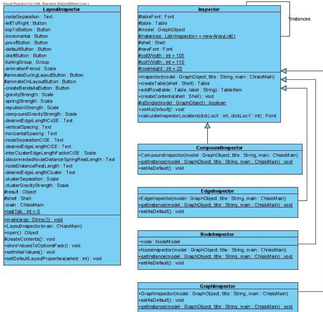
Figure 3.6: A UML Class Diagram illustrating the inspector dialogs in CHISIO
