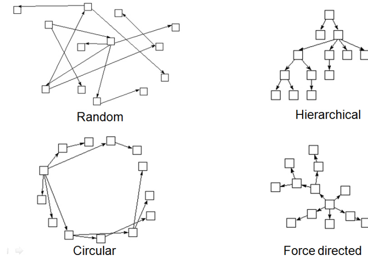
Figure 1.4: Different layouts for the same graph
