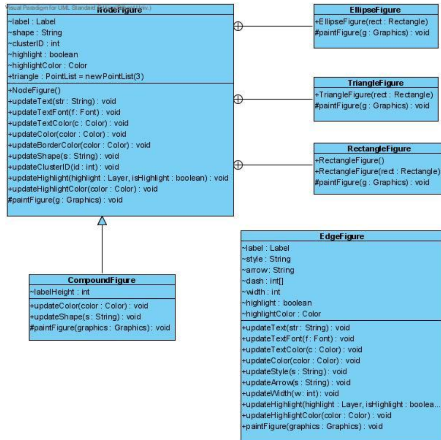
Figure 3.2: A UML Class Diagram illustrating the figure relations in CHISIO
