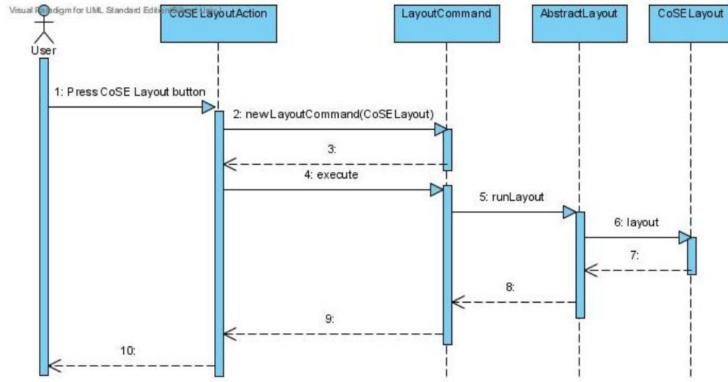
Figure 3.5: A UML Sequence Diagram for running CoSE layout in CHISIO
