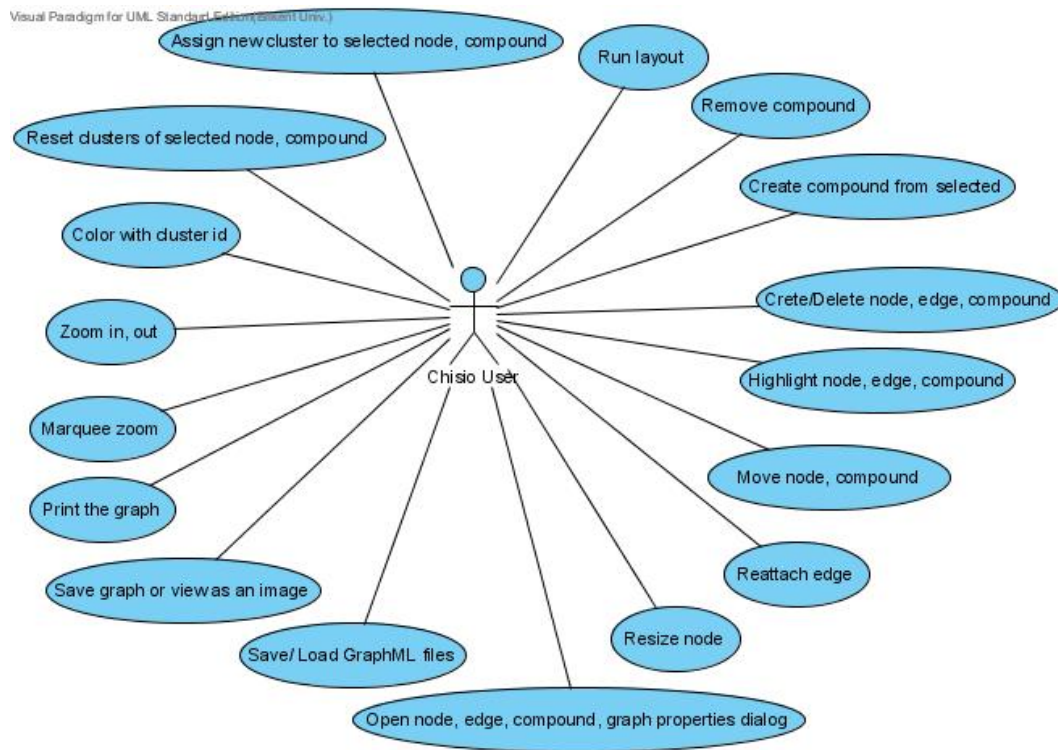
Figure 3.9: A UML Use Case Diagram for CHISIO as an editor
