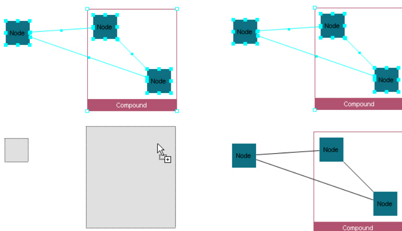
Figure 4.17: Clone operation; drag selected nodes pressing the CTRL key in the transfer mode and click to clone
