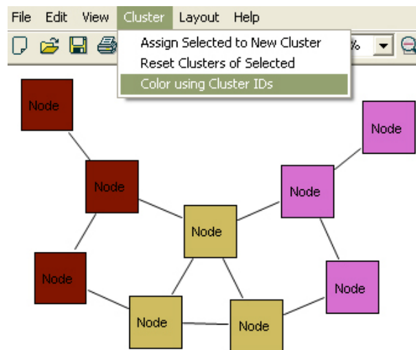
Figure 4.28: Coloring with cluster IDs results in three clusters, each with a unique color
