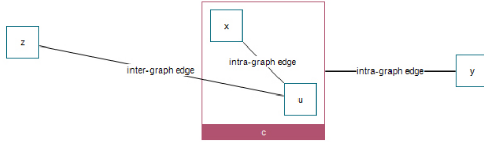
Figure 1.5: Compound graph with inter-graph and intra-graph edges
