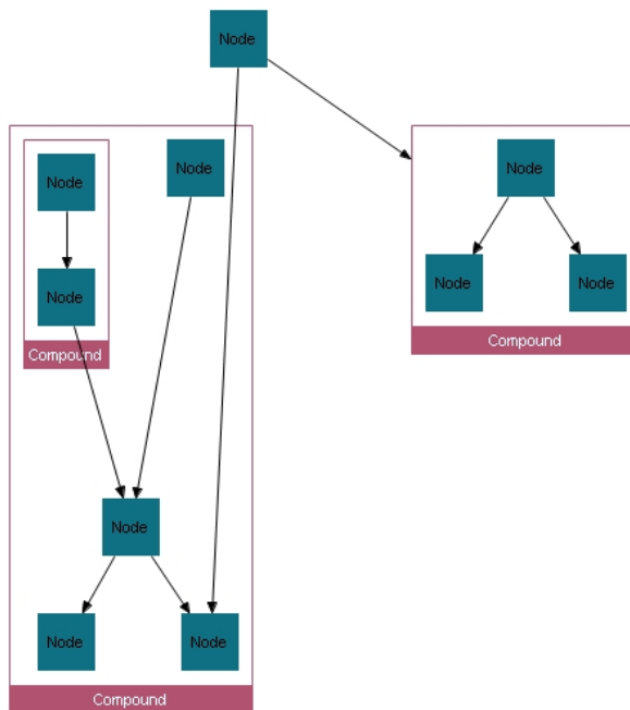
Figure 6.15: Hierarchical layout with compound support
