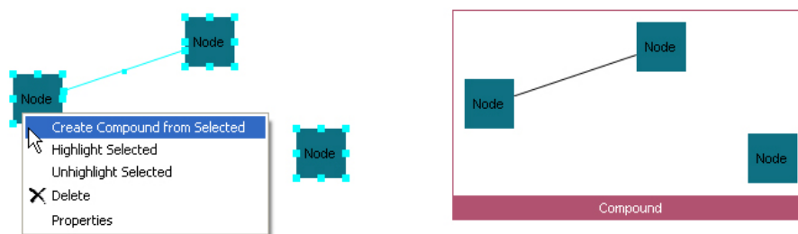
Figure 4.18: Create compound (right) from selected nodes (left)
