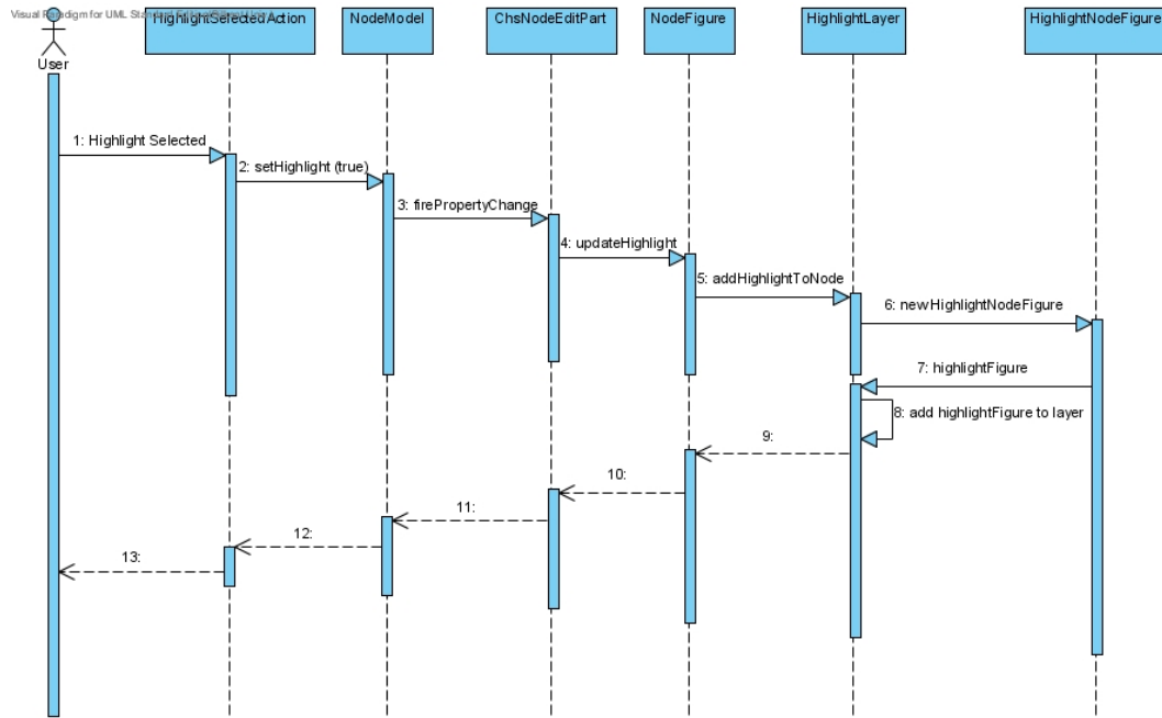
Figure 3.8: A UML Sequence Diagram for highlighting a node in CHISIO
