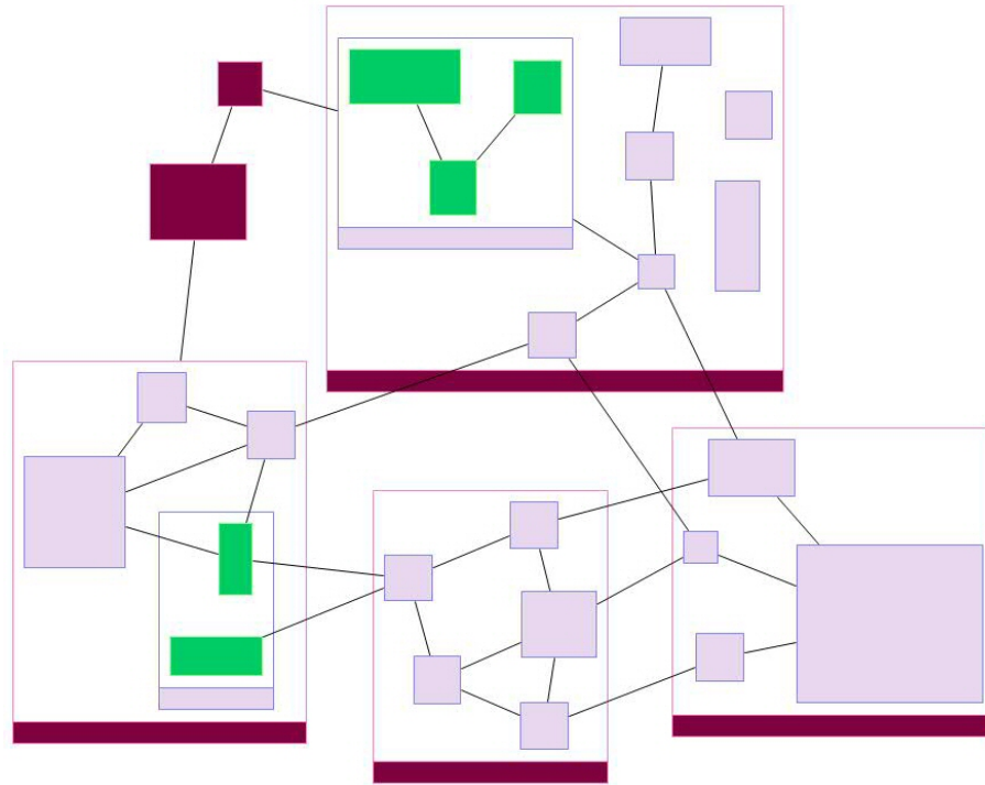
Figure 6.1: Sample CoSE layout produced by CHISIO
