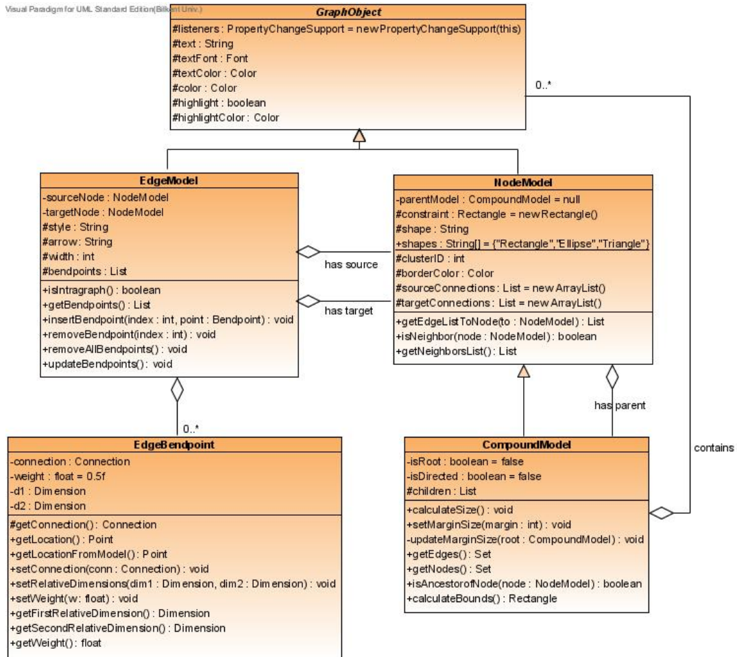
Figure 3.1: A UML Class Diagram illustrating the compound graph model used in CHISIO
