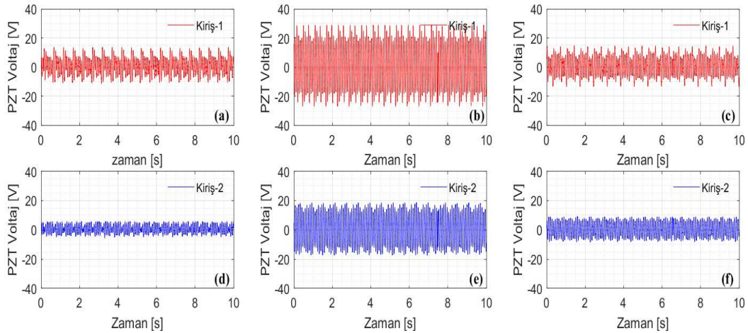
Şekil 6.5. Sistemin piezoelektrik voltaj üretimi: (a) Beam-1: T_p = 0.3 s, T_s = 0.2 s (b) Beam-1: T_p = 0.3 s, T_s = 0.3 s (c) Beam-1: T_p = 0.3 s, T_s = 0.4 s (d) Beam-2: T_p = 0.3 s, T_s = 0.2 s (e) Beam-2: T_p = 0.3 s, T_s = 0.3 s (f) Beam-2: T_p = 0.3 s, T_s = 0.4 s.
