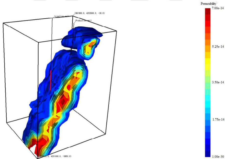
Figure 4.4 Permeability distribution
