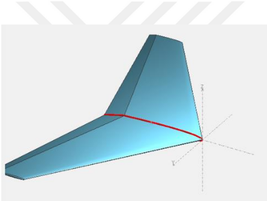
Figure 2.13. Negative elevator deflection
