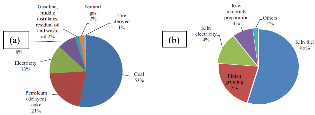
Figure 2.1 (a) Total Energy for Cement Manufacturing Sector by Energy Source, 2006 [37]; (b) Total Energy for Cement Manufacturing Sector by Process Step, 2006 [37]
