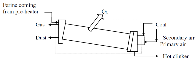
Figure 2.2 Rotary kiln and the materials going into and leaving
