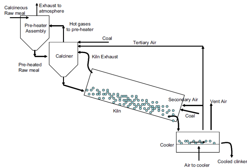
Figure 2.3 Schematic of cement clinker process [65].
