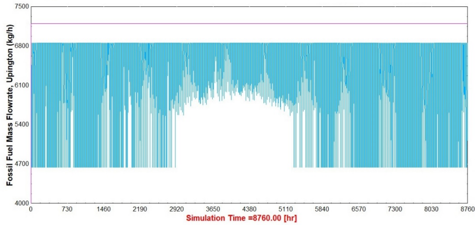
Figure 7.18 Fuel mass flowrate (kg/h) in a conventional vs. solar cement plant, Upington-South Africa
