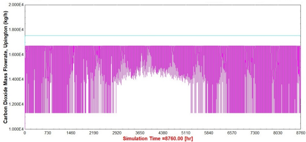
Figure 7.20 CO 2 emission flow rate in a conventional vs. a solar-hybridized cement plant, Upington-South Africa
