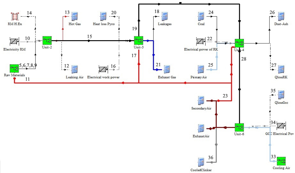
Figure 7.4 The schematic of the TRNSYS model of a cement manufacturing plant
