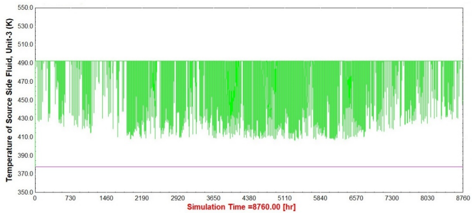
Figure 7.21 Temperature (K) profile of preheated farine, Model-3
