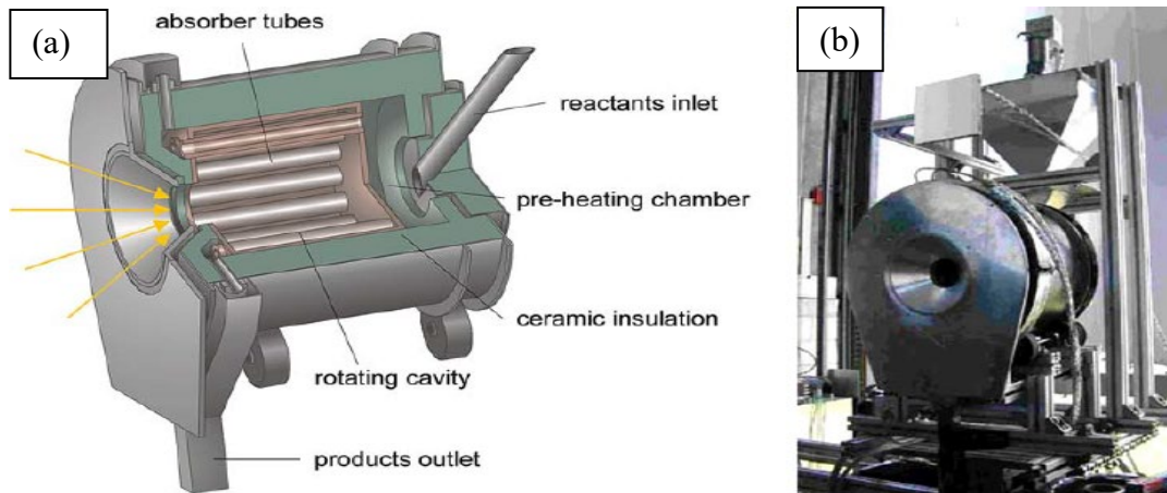
Figure 2.4 (a) Schematic of the multi-tube rotary kiln prototype [74]; (b) A solar kiln prototype [74].
