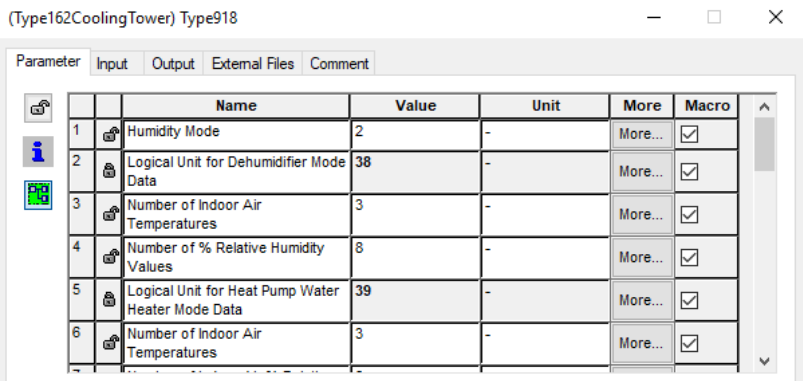
Figure 6.2 Cooling tower Variable Table
