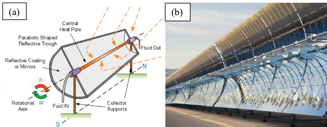
Figure 4.9 (a) General conceptual form of a PTC [118]; (b) A parabolic trough collector [35].
