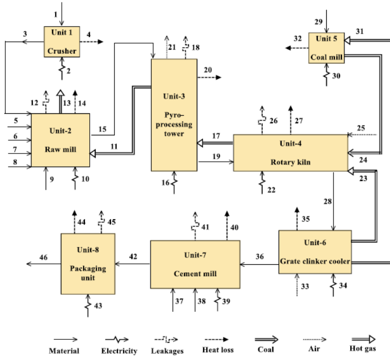
Figure 7.3 The schematic of an actual cement manufacturing plant [30].
