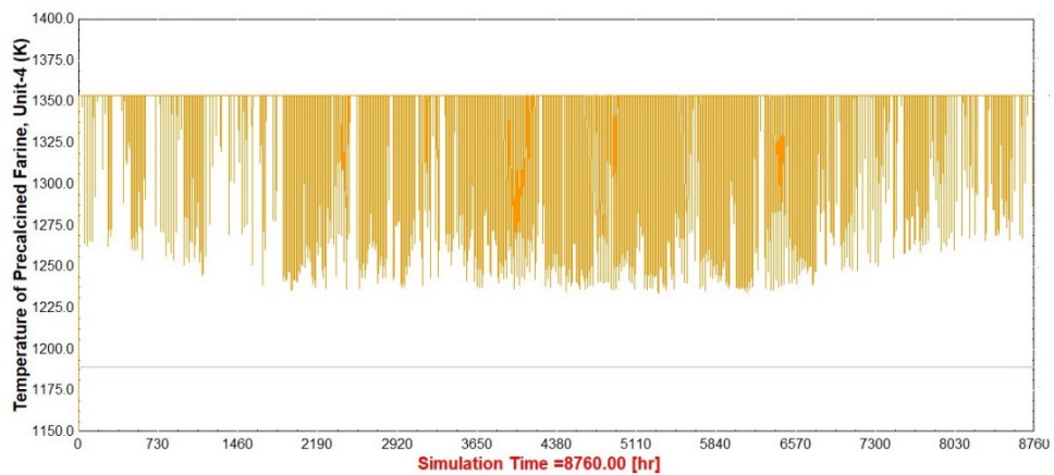
Figure 7.22 Temperature (K) profile of the precalcined farine, Model-3
