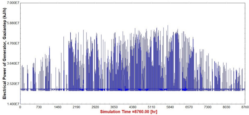
Figure 7.13 Electric power of generator (kJ/h), Gaziantep-Turkey
