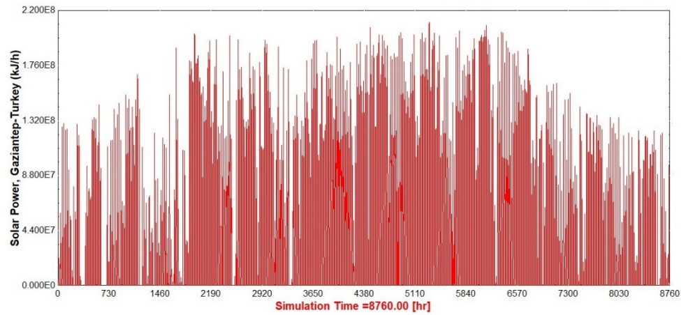
Figure 7.11 Generated power by heliostat solar field (kJ/h), Gaziantep-Turkey
