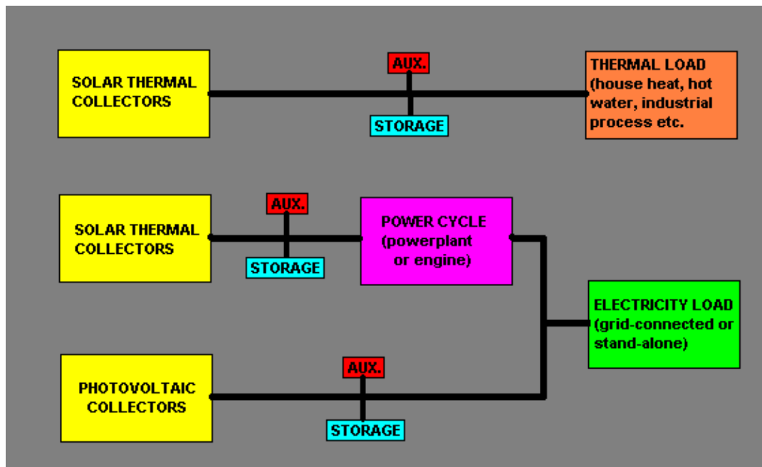
Figure 4.1 Diagram of a basic solar energy conversion system. The AUX. box represents some auxiliary source of thermal or electrical energy [35].
