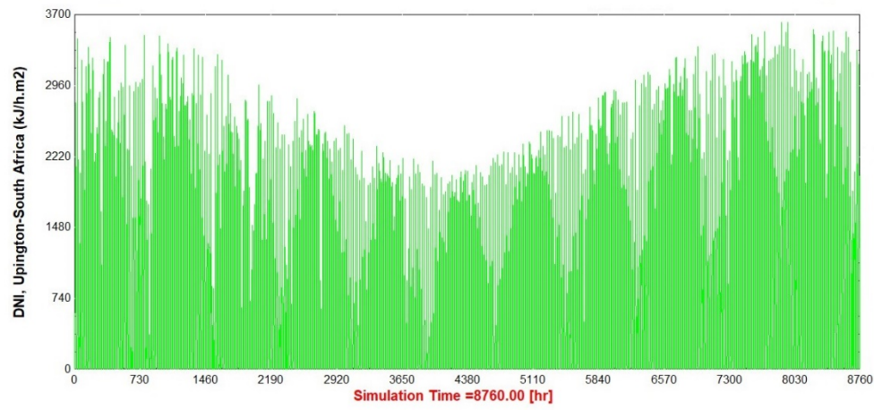
Figure 7.8 Annual DNI (kJ/h.m 2 ) profile, Upington-South Africa
