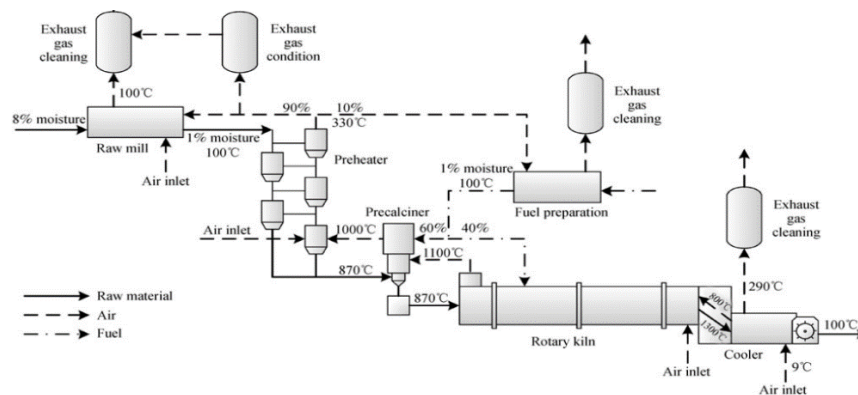
Figure 6.4 General flow diagram for a cement plant [68],
