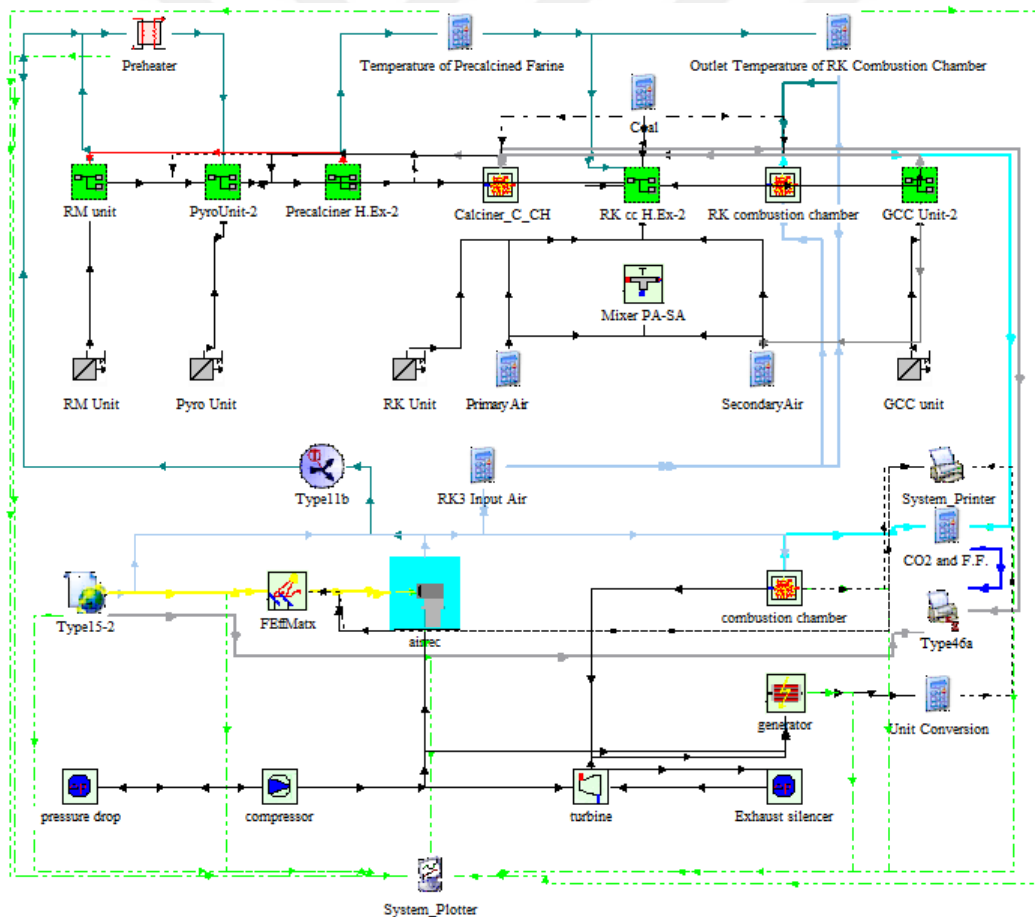
Figure 6.41 TRNSYS Layout of the Solar-integrated Cement Plant with a solar-based preheater
