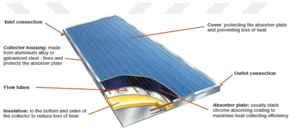
Figure 4.3 Flat-plate solar collector [110].
