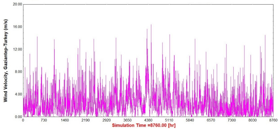
Figure 7.6 Wind velocity (m/s) profile, Gaziantep-Turkey
