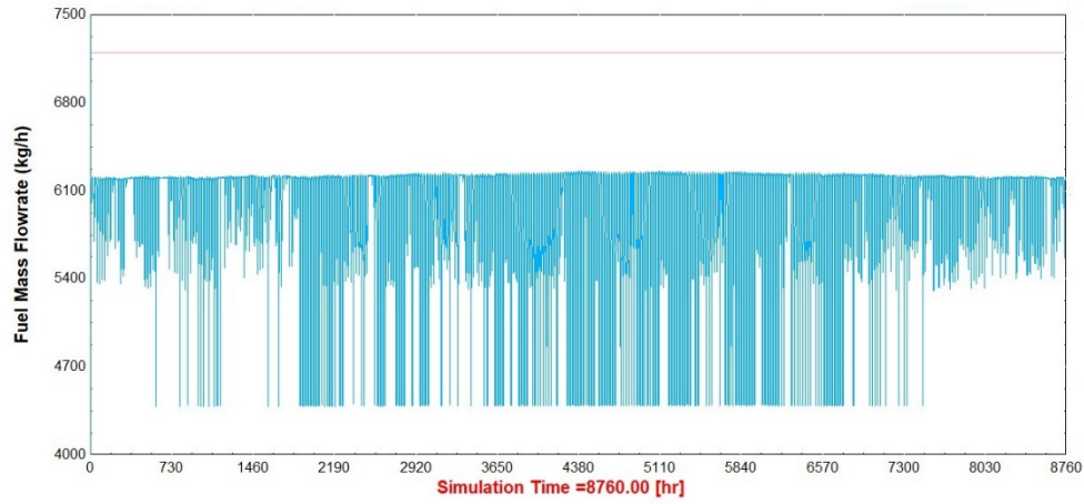
Figure 7.24 Fuel mass flowrate (kg/h), Model-3
