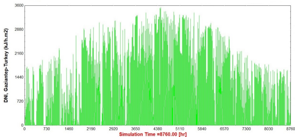
Figure 7.5 Annual DNI (kJ/h.m 2 ) profile, Gaziantep-Turkey
