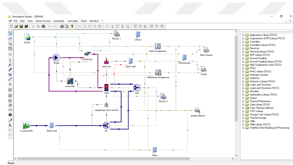
Figure 6.1 The TRNSYS Simulation Studio: Model of a solar domestic hot water system
