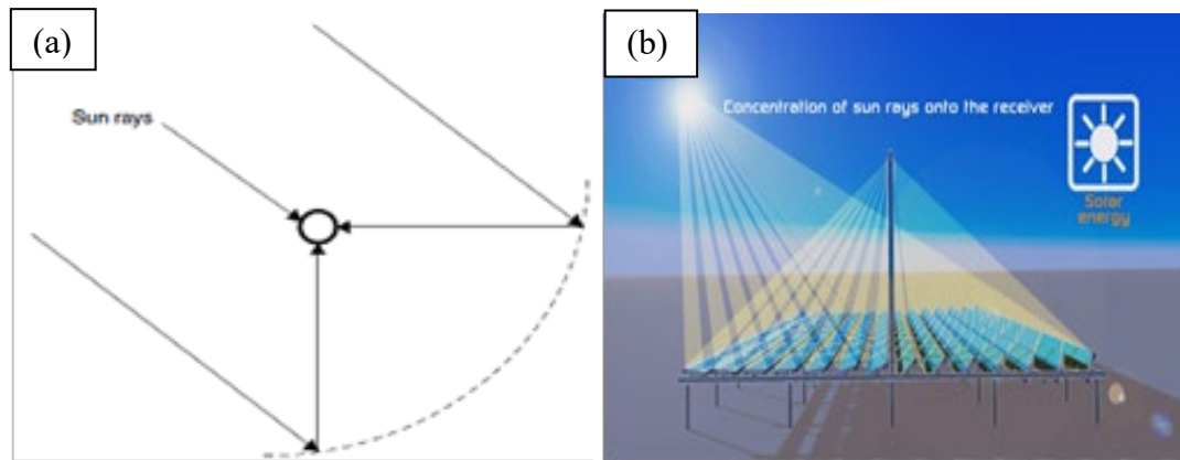
Figure 4.7 (a) Linear Fresnel-type parabolic trough collector [109]; (b) a downward-facing receiver illuminated from an LFR field [115].
