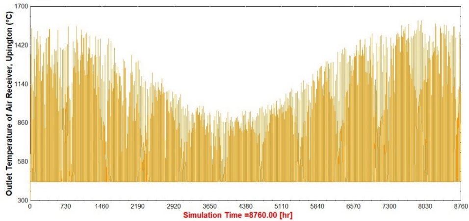
Figure 7.16 T_{out} Air Receiver (°C) Profile, Upington-South Africa
