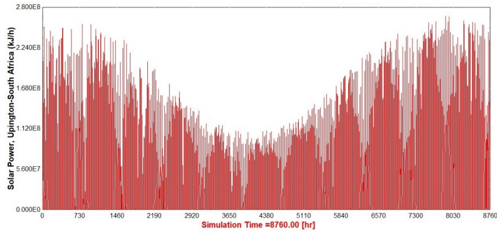
Figure 7.12 Generated power by heliostat solar field (kJ/h), Upington-South Africa
