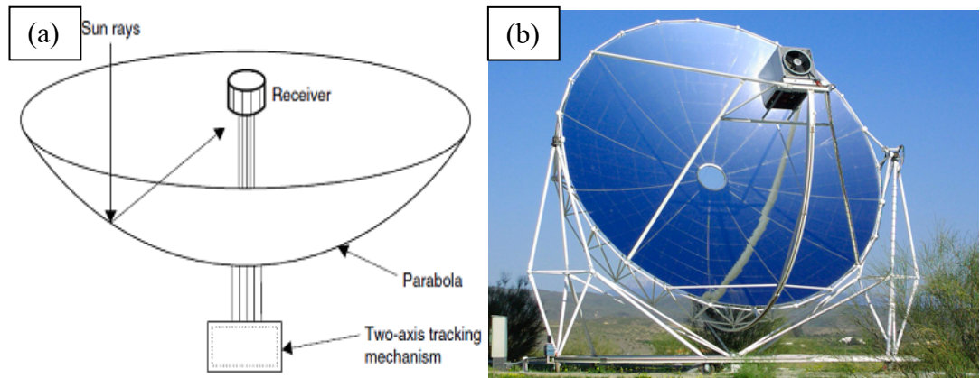
Figure 4.10 (a) Schematic diagram of a PDR [110]; (b) a PDR [120].
