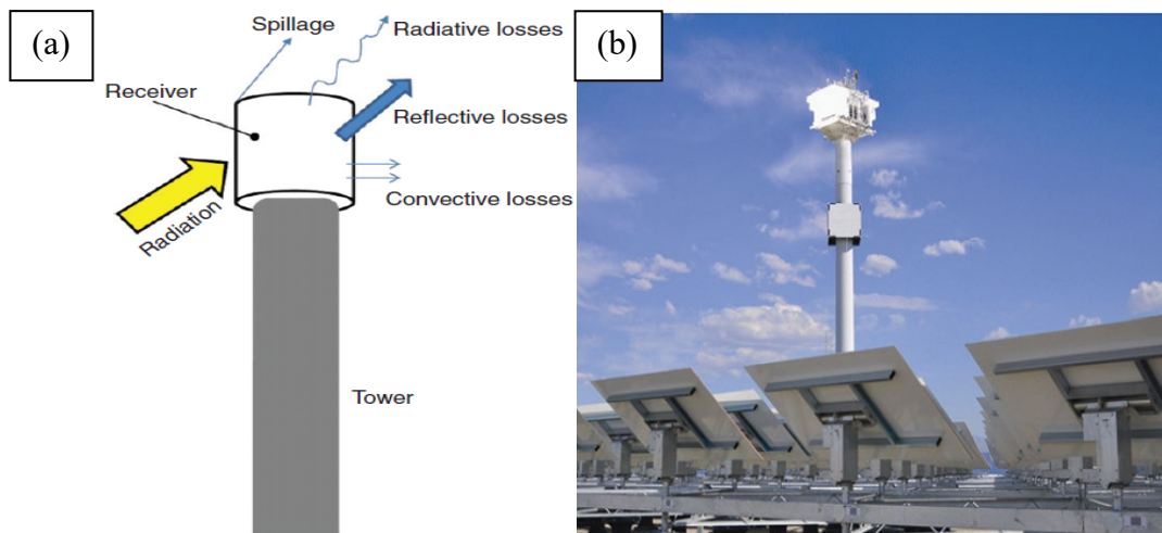
Figure 4.16 (a) Energy balance of a solar receiver [124]; (b) Solar receiver system of eSolar [124].
