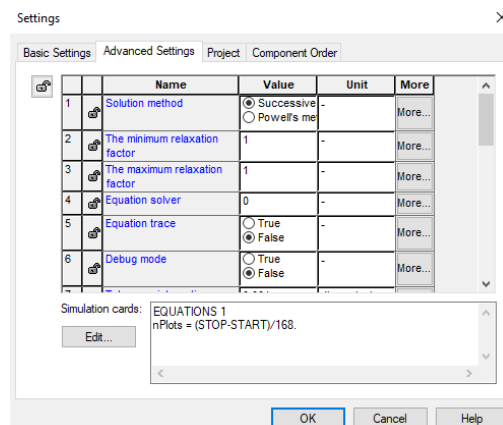
Figure 7.2 TRNSYS settings window
