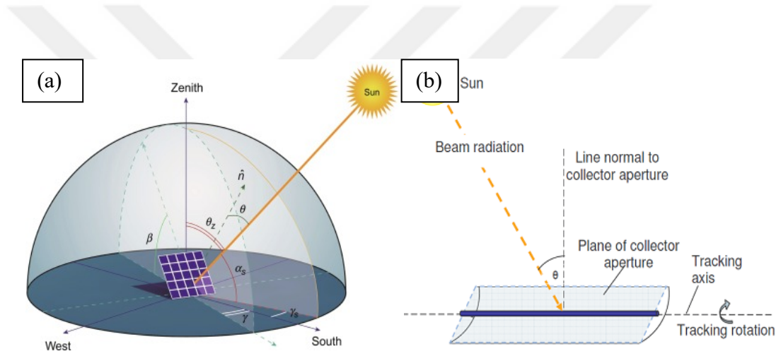
Figure 4.12 (a) Solar and PV module characteristic angles [129]; (b) Angle of incidence on a parabolic trough collector [127].
