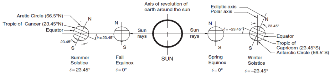
Figure 4.13 Yearly variation of solar declination [124].
