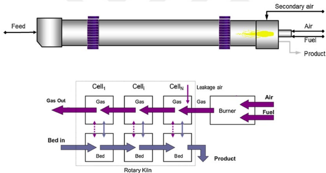
Figure 6.7 Model scheme of the counter current rotary kiln [144].
