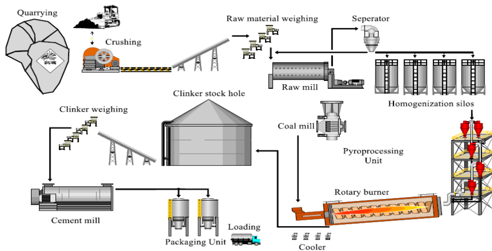
Figure 3.1 Process flow diagram of the cement manufacturing process [79].
