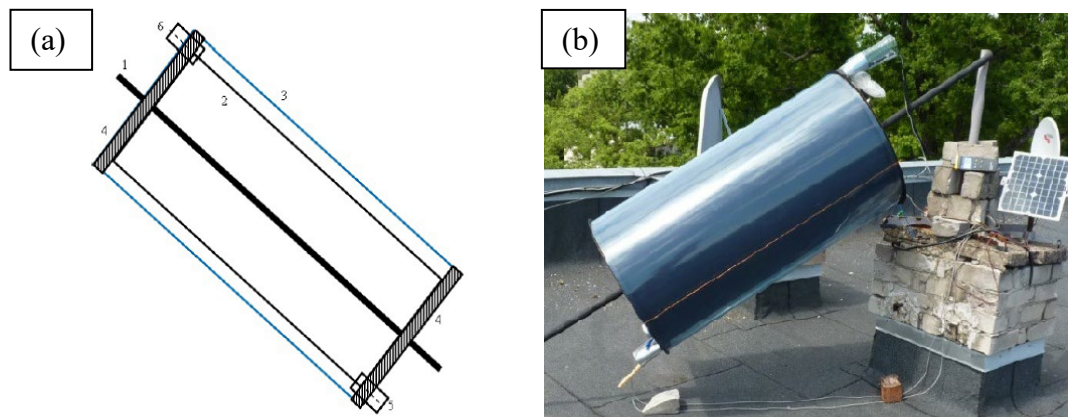
Figure 4.8 (a) Structure of cylindrical solar collector: 1. Axis, 2. Inner cylinder-absorber, 3. Outer transparent cylinder, 4. Thermoinsulation at ends, 5. Inflow opening, 6. Outflow opening [116]; (b) Cylindrical solar collector [116].
