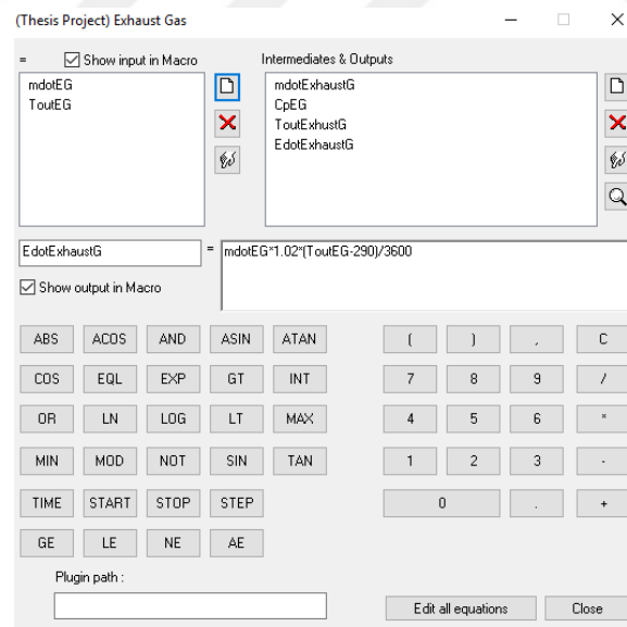
Figure 6.16 Exhaust Gas equation window
