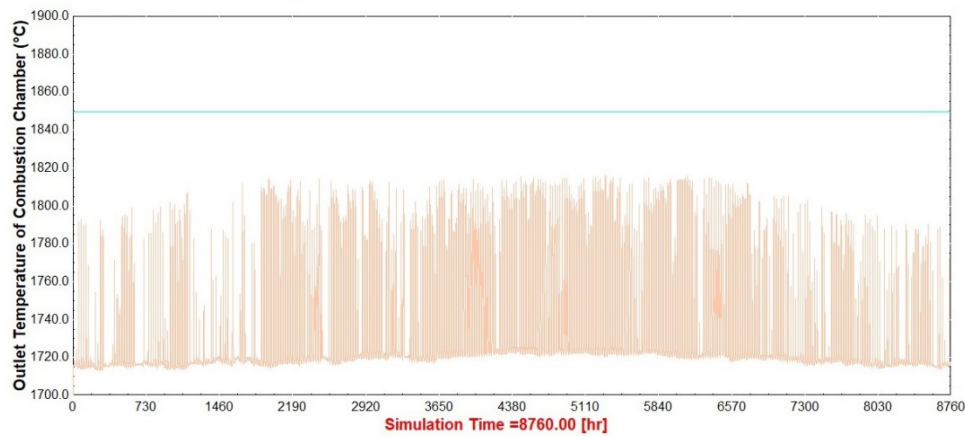
Figure 7.23 Outlet temperature of the combustion chamber (°C), Model-3
