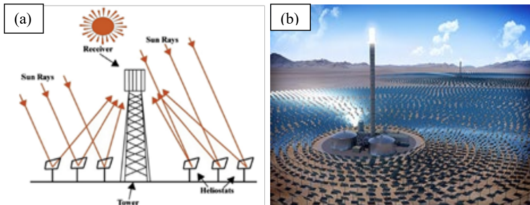
Figure 4.11 (a) Schematic diagram of a HFC [121]; (b) A heliostat solar field [122].
