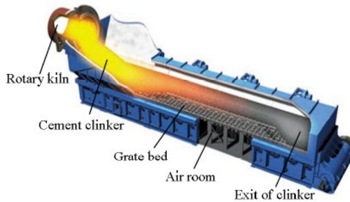
Figure 3.3 The schematic diagram of grate cooler [102].
