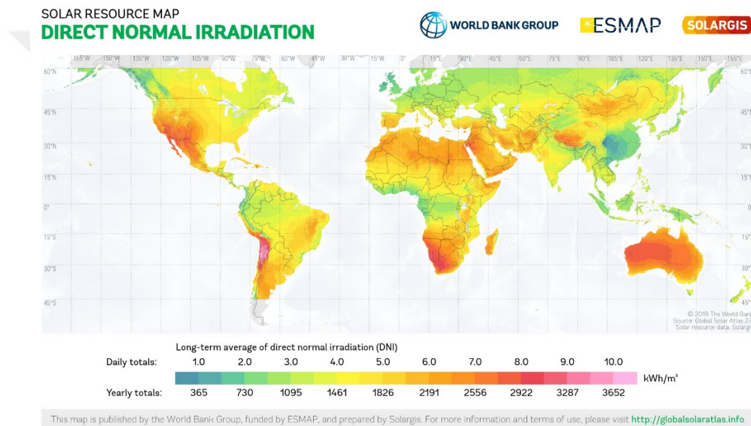
Figure 4.2 Global map of direct normal irradiation [94].
