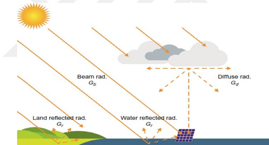
Figure 4.14 Solar radiation components striking the ground and the PV panel [129].
