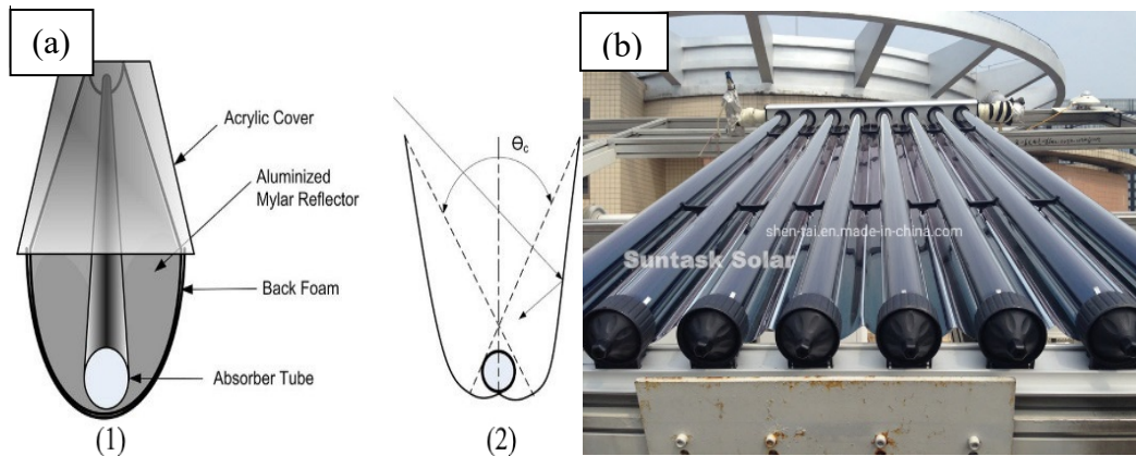
Figure 4.4 (a) Schematic of: (1) one compound parabolic collector, (2) The value of acceptance angle \theta_c ; (b) Poland CPC solar collector.
