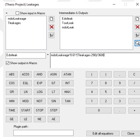
Figure 6.26 Leakages equation window
