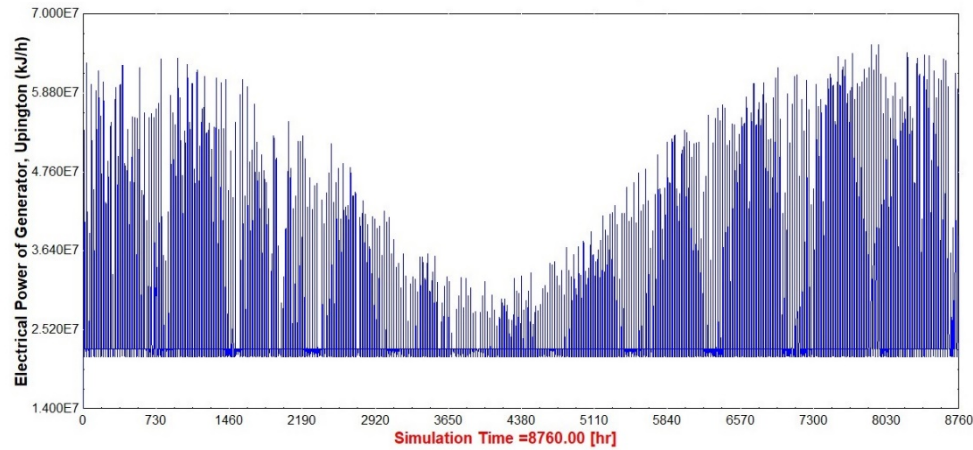
Figure 7.14 Electric power of generator (kJ/h), Upington-South Africa
