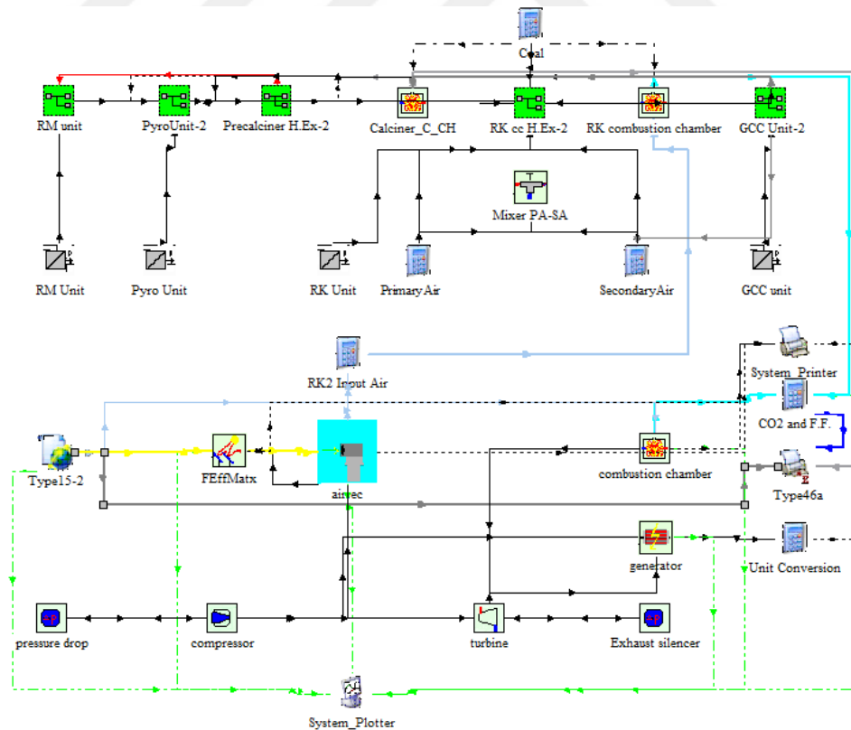
Figure 6.38 TRNSYS Layout of the Solar-integrated Cement Plant
