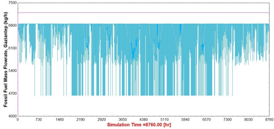
Figure 7.17 Fuel mass flowrate (kg/h) in a conventional vs. solar cement plant, Gaziantep-Turkey
