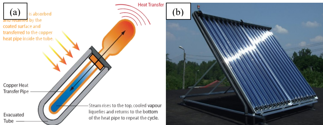
Figure 4.5 Diagram of an ETC [113]; (b) ET solar collector [114].
