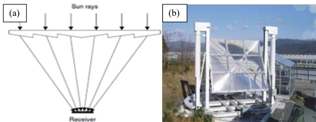
Figure 4.6 (a) Fresnel lens collector (FLC) [109]; (b) FLC solar furnace [114].
