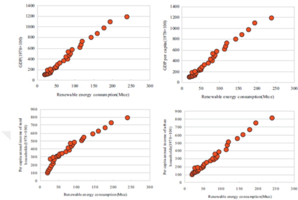
Figure 34: Renewable Energy Consumption in China and its Relation with Chinese GDP, (Mtce)
