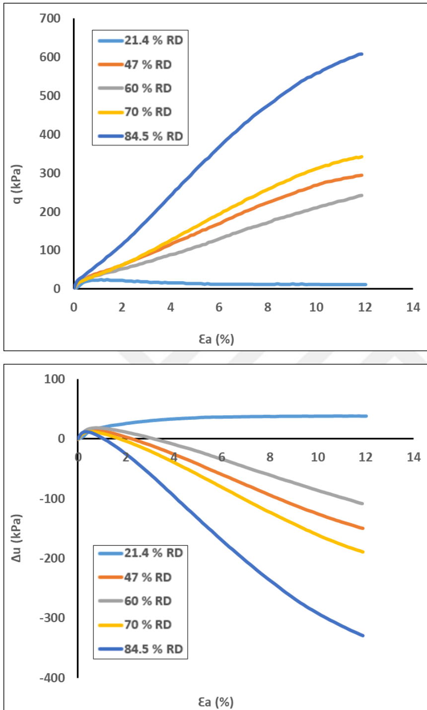
Figure 4.21. Effect of void ratio on the behavior of Çine sand under 50 kPa consolidation pressure
