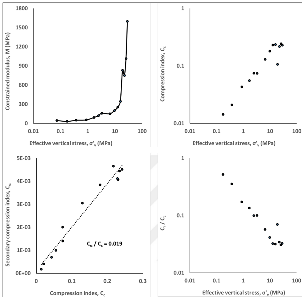
Figure 4.51. Results of 50% relative density sample
