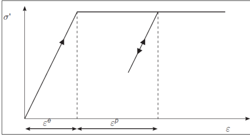
Figure 5.1. Linear elastic perfectly plastic model
