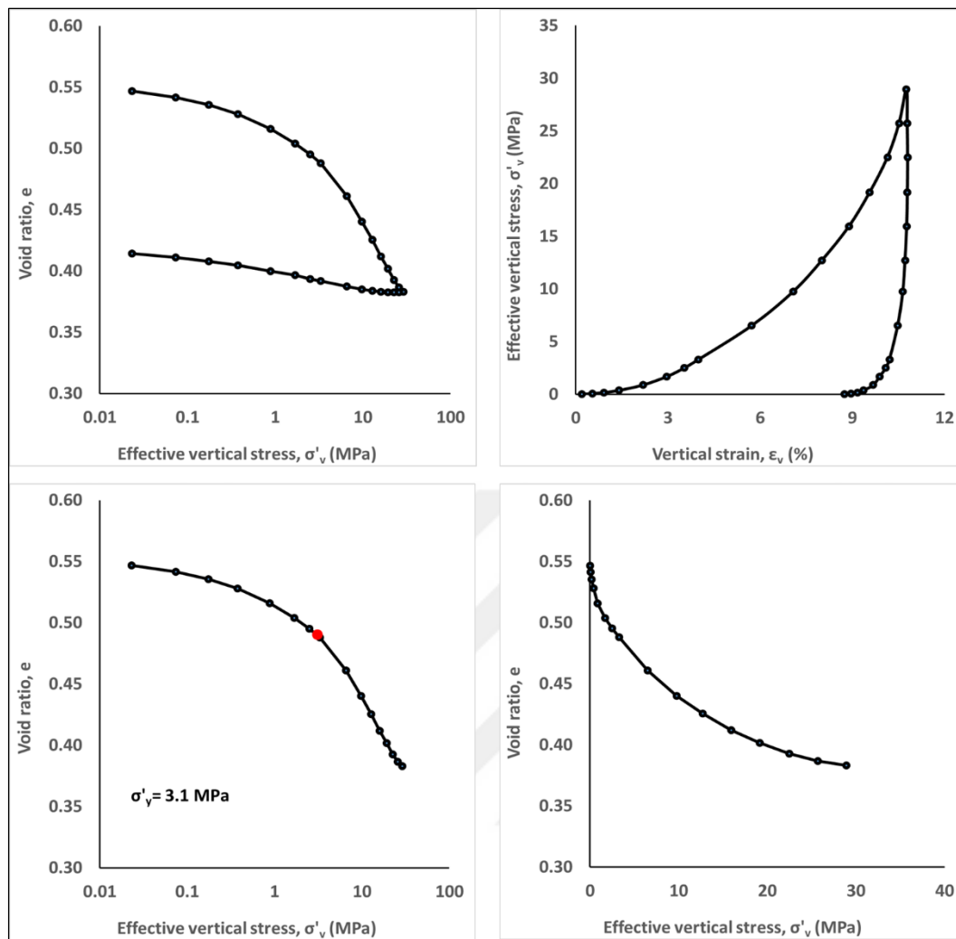
Figure 4.47. Oedometer test results of 85 % relative density sample
