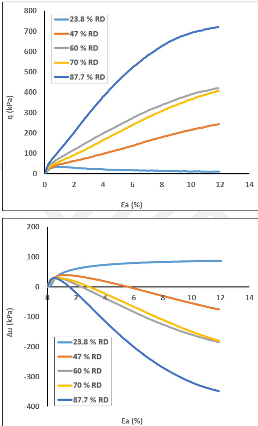
Figure 4.22. Effect of void ratio on the behavior of Çine sand under 100 kPa consolidation pressure
