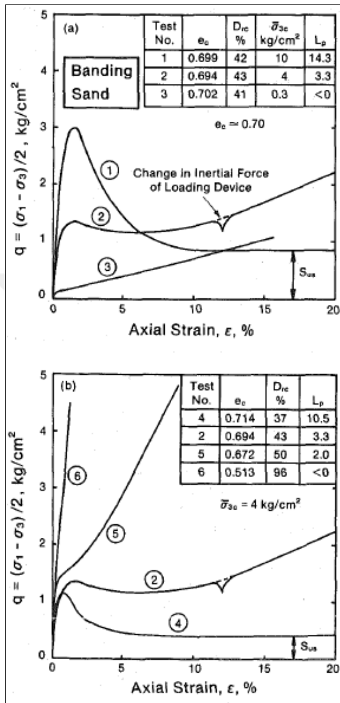
Figure 2.9. Effects of void ratio and confining stress on the undrained behavior of Banding Sand (Castro, 1969)
