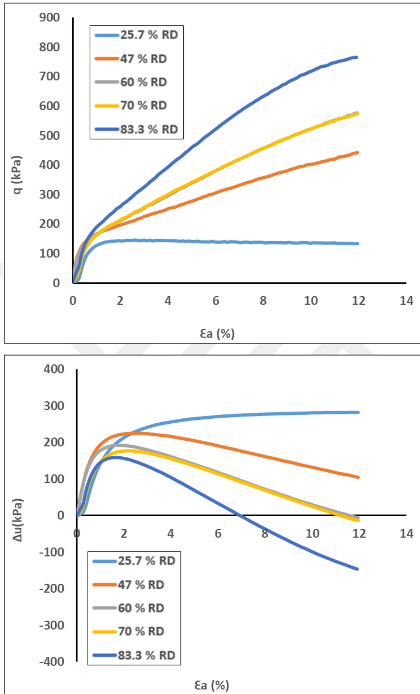
Figure 4.24. Effect of void ratio on the behavior of Çine sand under 400 kPa consolidation pressure
