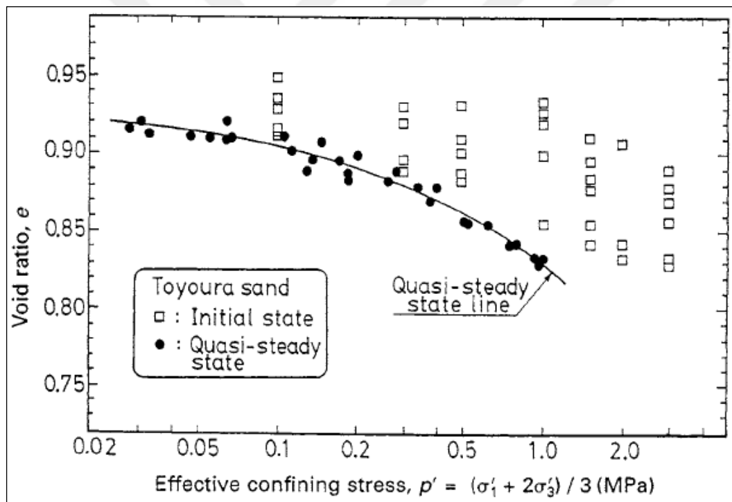
Figure 2.13. Quasi steady state line of Toyoura sand (Ishihara, 1996)
