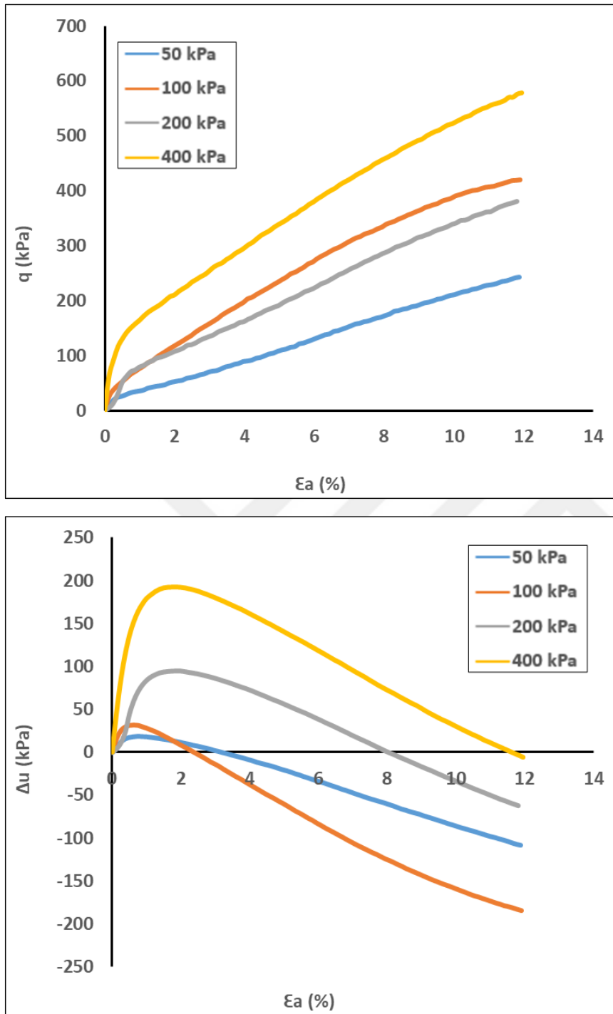
Figure 4.31. Effect of stress state on the behavior of Çine sand with 60 % relative density
