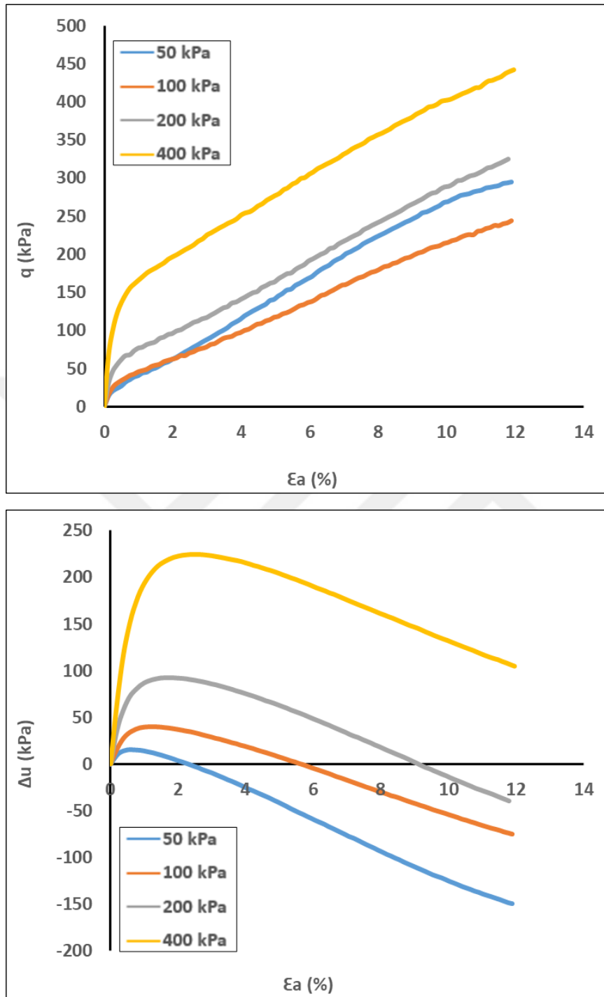
Figure 4.30. Effect of stress state on the behavior of Çine sand with 47 % relative density
