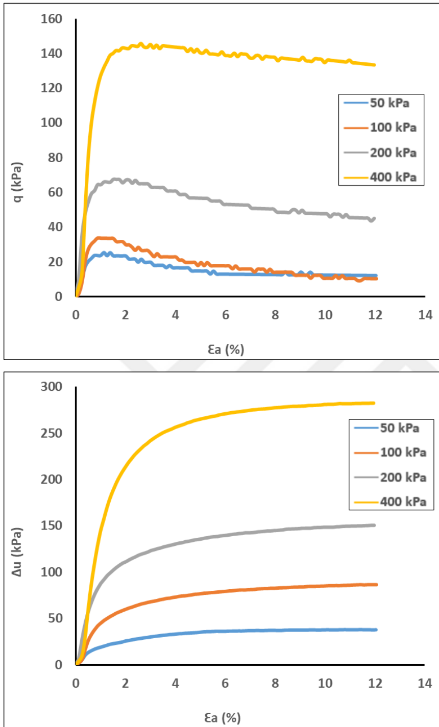
Figure 4.29. Effect of stress state on the behavior of Çine sand with 21 – 26 % relative density
