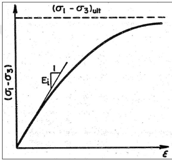
Figure 5.8. Hyperbolic stress-strain relationship of soils
