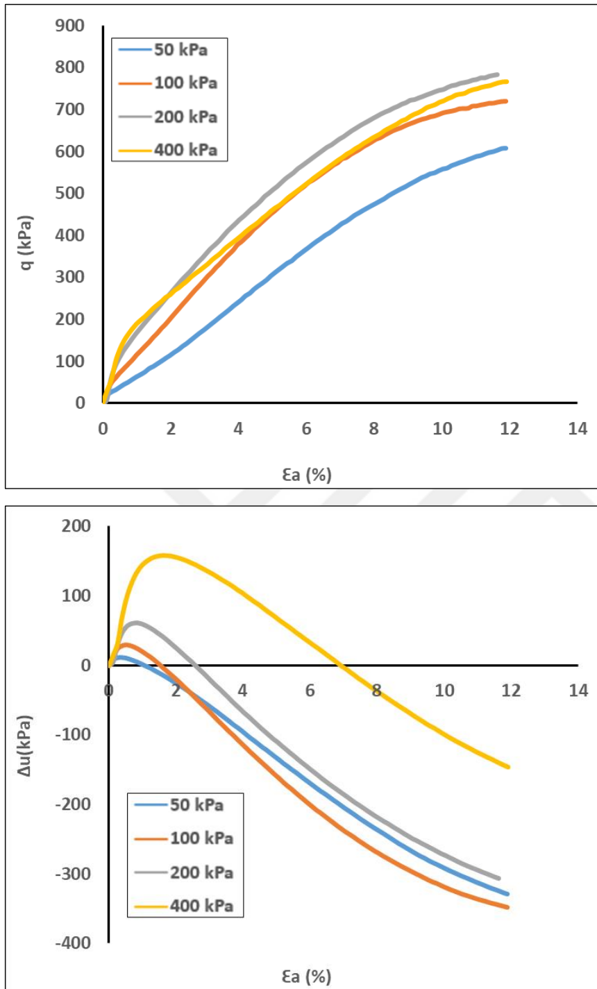
Figure 4.33. Effect of stress state on the behavior of Çine sand with 83 – 88 % relative density
