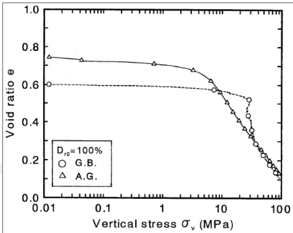
Figure 2.18. Effect of particle angularity on the compressibility behavior
