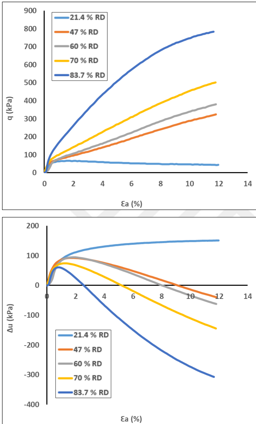
Figure 4.23. Effect of void ratio on the behavior of Çine sand under 200 kPa consolidation pressure
