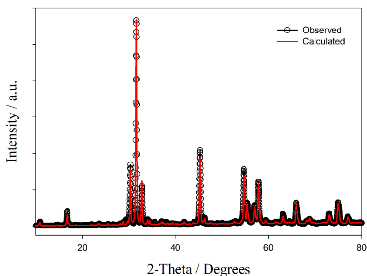
Figure 4.10 The XRD spectra and results of Rietveld refinement of synthesized \text{Ag}_2\text{WO}_4 powders (ICSD 243992). PVP-assisted hydrothermal method was investigated to decrease the particle size of \text{Ag}_2\text{WO}_4 powders. The only difference between the experiments was the addition of 1.5 g of PVP addition to the \text{AgNO}_3 solution. All other steps are similar.
