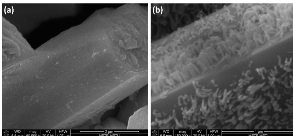
Figure 4.9 SEM images of \text{Ag}_2\text{WO}_4 powders, synthesized at PVP assisted hydrothermal synthesis, (a) at time zero and (b) after 2 minutes of the electron bombardment.
