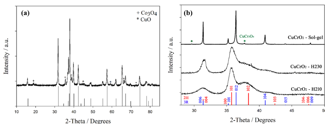
Figure 4.24 The XRD spectra of powders synthesized through (a) \text{CuCoO}_2 , (b) \text{CuCrO}_2 , \text{CuCrO}_2 -H210 and \text{CuCrO}_2 -H230 experiments.
