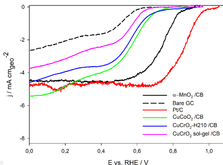
Figure 4.26 Rotating-disk voltammograms of \alpha - \text{MnO}_2 , Pt/C, \text{CuCoO}_2 , \text{CuCrO}_2 (obtained at H210 experiment) and \text{CuCrO}_2 (synthesized at sol-gel experiment) loaded and bare glassy carbon working electrode in \text{O}_2 purged 0.1 M KOH aqueous electrolyte with a sweep rate of 5 mV/s at 1600 rpm.
