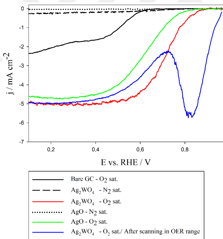
Figure 4.21 Rotating-disk voltammograms of AgO, Ag 2 WO 4 loaded and bare glassy carbon working electrode in O 2 and N 2 purged 0.1 M KOH aqueous electrolyte with a sweep rate of 5 mV/s.
