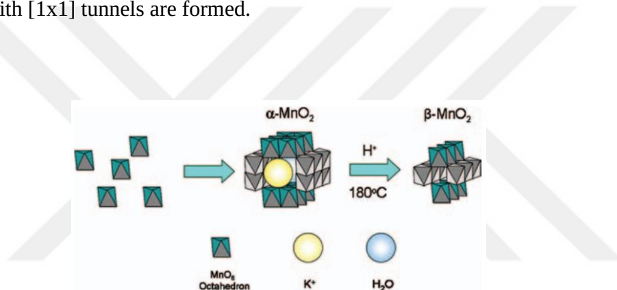
Figure 4.6 Schematic drawn of structures of \alpha -MnO 2 and \beta -MnO 2 [95].
