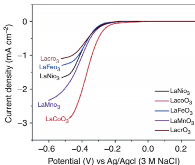
Figure 2.16 RDE test for \text{LaMO}_3 peroxides ( \text{M} = \text{Ni}, \text{Co}, \text{Fe}, \text{Mn}, \text{Cr} ) performed at 1600 rpm with a scan rate of 20 mV/s [85].
