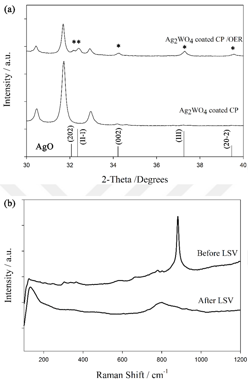
Figure 4.22 (a) The XRD spectra of Ag 2 WO 4 loaded carbon paper (CP), Ag 2 WO 4 loaded CP after LSV in OER range; (b) Raman spectra of \alpha - Ag 2 WO 4 powders before and after LSV.
