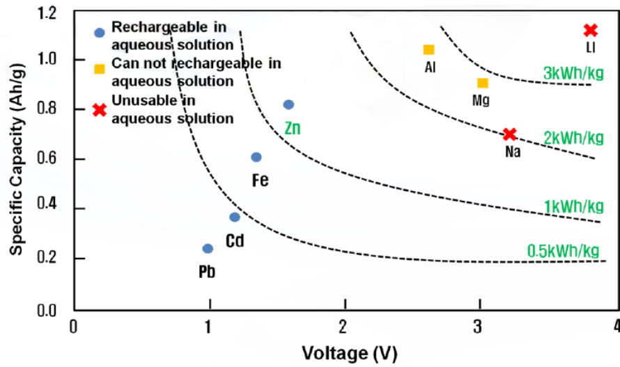
Figure 2.3 Metal-air batteries in aqueous solution [64].
