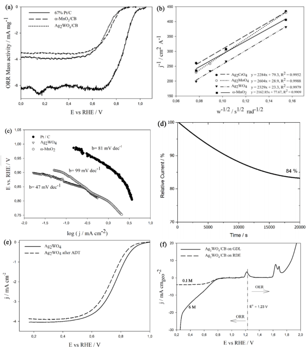
Figure 4.14 (a) Mass activities of synthesized \text{Ag}_2\text{WO}_4 , \alpha\text{-MnO}_2 with carbon black mixture and commercial 67 wt% Pt/C; (b) Koutecky-Levich plots obtained at 0.365 V (vs. RHE) for \text{Ag}_2\text{CrO}_4 , \text{Ag}_2\text{MoO}_4 , \text{Ag}_2\text{WO}_4 and \alpha\text{-MnO}_2 powders; (c) Tafel plots of synthesized \text{Ag}_2\text{WO}_4 , \alpha\text{-MnO}_2 with carbon black mixture and commercial 67 wt% Pt/C; (d) Chronoamperometry curve of \text{Ag}_2\text{WO}_4 powders; (e) Linear sweep voltammograms of \text{Ag}_2\text{WO}_4 powders before and after the accelerated durability test; (f) Linear sweep voltammogram of \text{Ag}_2\text{WO}_4 powders loaded on gas diffusion layer for ORR and OER range.
