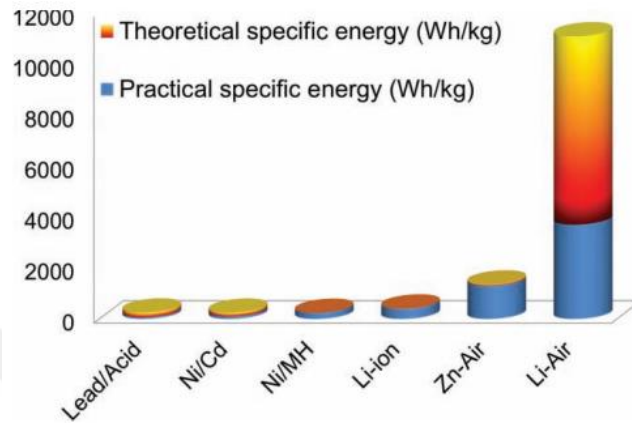
Figure 2.2 Theoretical and practical energy densities of different types of batteries [62].
