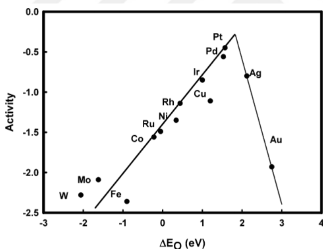
Figure 2.15 Graph of oxygen reduction activity versus oxygen binding energy [84].
