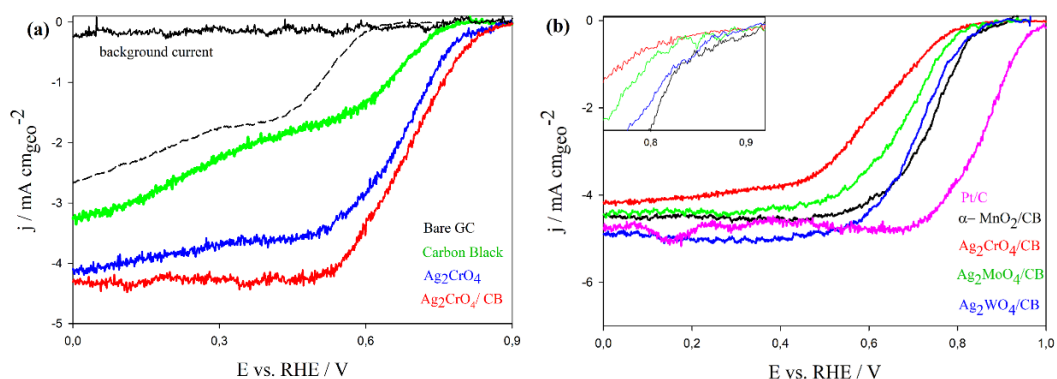
Figure 4.12 (a) Rotating-disk voltammograms of pure \text{Ag}_2\text{CrO}_4 , carbon black (CB/Printex L6) and \text{Ag}_2\text{CrO}_4/\text{CB} loaded and bare glassy carbon working electrode in \text{O}_2 purged 0.1 M KOH aqueous electrolyte with a sweep rate of 5 mV/s at 1600 rpm. Background current was recorded at \text{N}_2 saturated 0.1 M KOH aqueous electrolyte. (b) Rotating-disk voltammograms of Pt/C, \alpha\text{-MnO}_2 , \text{Ag}_2\text{CrO}_4 , \text{Ag}_2\text{MoO}_4 , \text{Ag}_2\text{WO}_4 and carbon black loaded and bare glassy carbon working electrode in \text{O}_2 purged 0.1 M KOH aqueous electrolyte with a sweep rate of 5 mV/s at 1600 rpm.
