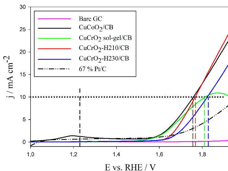
Figure 4.28 Rotating-disk voltammograms of CuCoO 2 and CuCrO 2 powders loaded and bare glassy carbon working electrode in O 2 purged 0.1 M KOH aqueous electrolyte with a sweep rate of 5 mV/s. The equilibrium potential for OER reaction ( E^0 = 1.23 V vs. RHE) and recorded potentials of each oxide at 10 mA cm -2 were shown by dotted lines.
