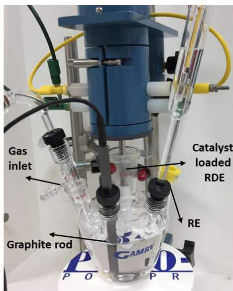
Figure 3.2 Setup of RDE experiments.
