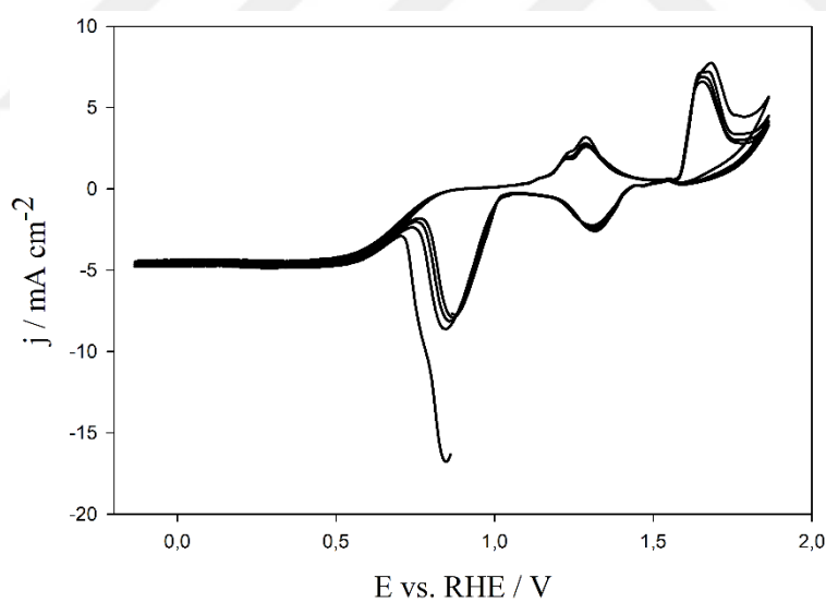
Figure 4.18 Cyclic voltammograms of \text{Ag}_2\text{WO}_4 powder in \text{O}_2 purged 0.1 M KOH aqueous electrolyte with a sweep rate of 20 mV/s.
