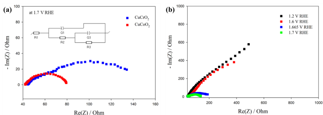
Figure 4.32 (a) EIS spectra of \text{CuCrO}_2 and \text{CuCoO}_2 samples at 1.7 RHE. Insert show the equivalent circuits used in fitting. (b) EIS spectra of \text{CuCrO}_2 samples at working potentials of 1.2, 1.6, 1.665 and 1.7 V RHE.
