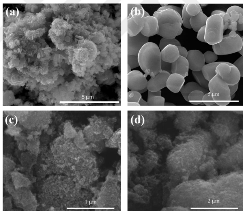
Figure 4.25 SEM images of (a) \text{CuCoO}_2 obtained via hydrothermal method, (b) \text{CuCrO}_2 obtained via sol-gel method, (c) \text{CuCrO}_2 obtained via hydrothermal method at 210 °C, (d) \text{CuCrO}_2 obtained via hydrothermal method at 230 °C.
