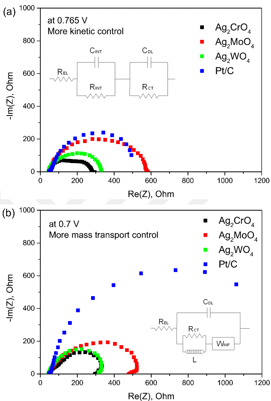
Figure 4.13 EIS spectra of samples at a working potential of (a) 0.765 V and (b) 0.7 V. Insert show the equivalent circuits used in fitting.
