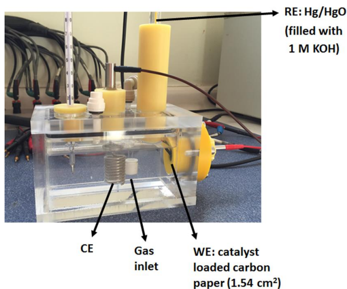
Figure 3.4 Three-electrode electrochemical cell for testing electrocatalytic activity of catalysts.
