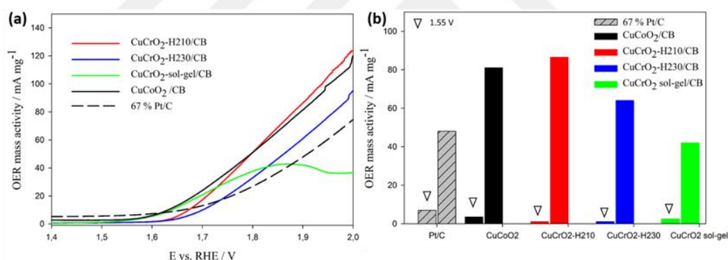
Figure 4.30 (a) Mass activities of synthesized copper delafossites with carbon black mixture and commercial 67 wt% Pt/C. (b) Bar chart of mass activities synthesized copper delafossites with carbon black mixture and commercial 67 wt% Pt/C at 1.55 and 1.9 V RHE.
