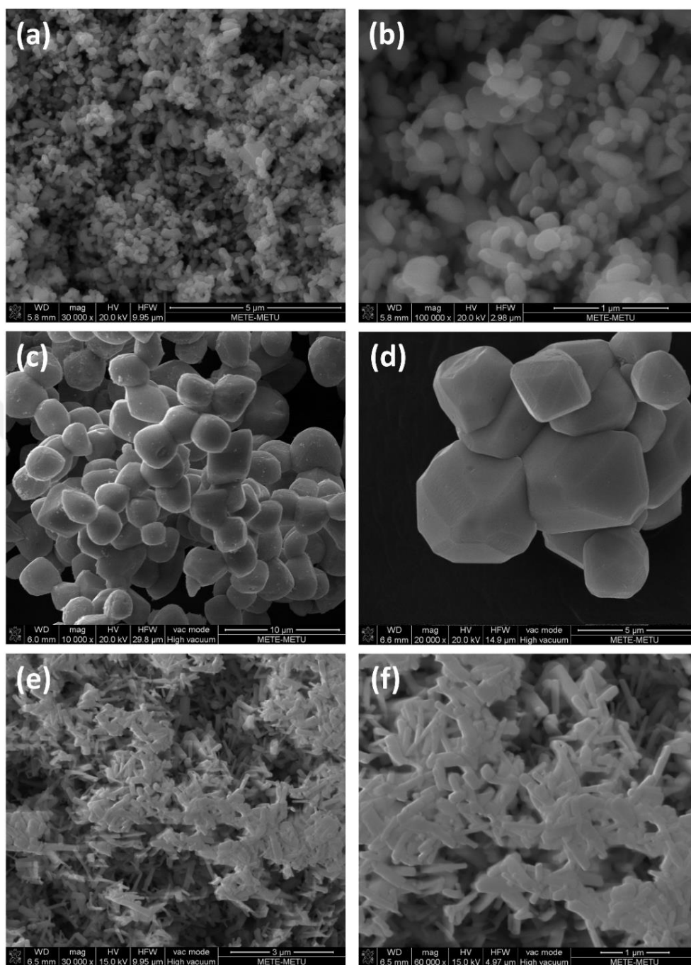
Figure 4.8 SEM images of: (a,b) \text{Ag}_2\text{CrO}_4 (c,d) \text{Ag}_2\text{MoO}_4 and (e,f) \text{Ag}_2\text{WO}_4 powders.
