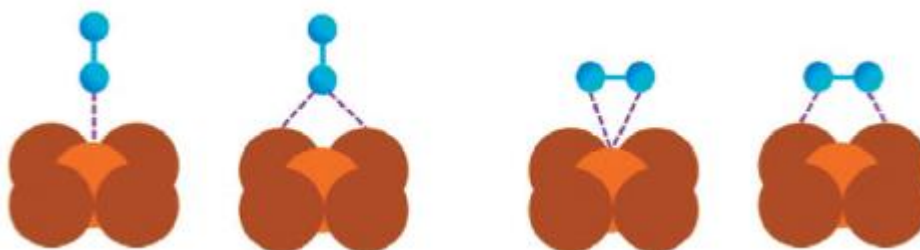
Figure 2.13 Various O_2 adsorption configurations on the surfaces of a catalyst: on top end-on, bridge end-on, bridge side-on one site, and bridge side-on two sites, from left to right [46].
