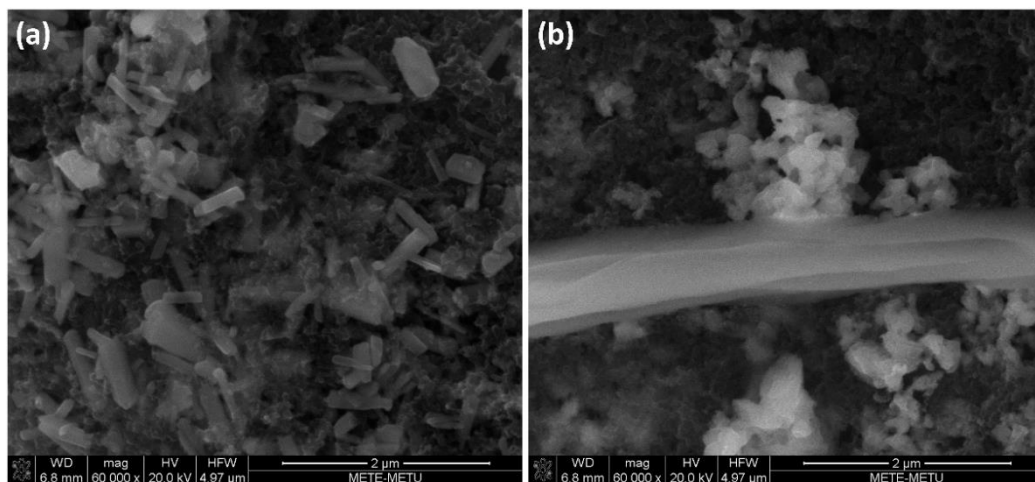
Figure 4.15 SEM micrographs of \text{Ag}_2\text{WO}_4 coated gas diffusion layer (a) before and (b) after several linear sweep voltammograms recorded in the OER range (0.865 to 2 V vs. RHE).
