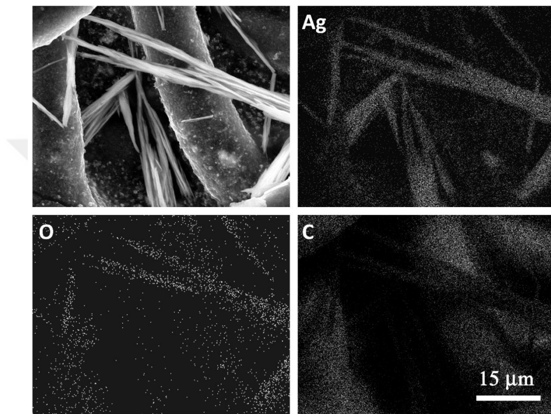
Figure 4.16 EDS mapping of \text{Ag}_2\text{WO}_4 coated gas diffusion layer after several scanning in the OER range. The scale at the right bottom applies to all.
