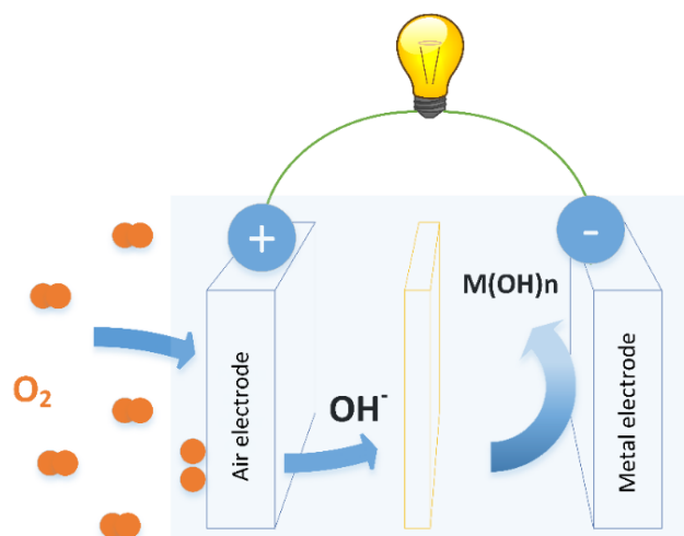
Figure 2.1 Schematic representation of a metal-air battery.
