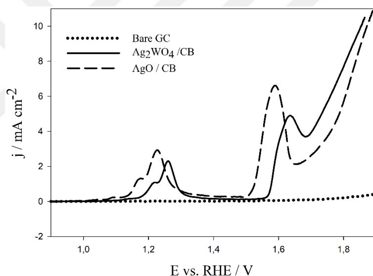
Figure 4.20 Rotating-disk voltammograms of AgO, \text{Ag}_2\text{WO}_4 loaded and bare glassy carbon working electrode in \text{O}_2 purged 0.1 M KOH electrolyte with a sweep rate of 5 mV/s at 1600 rpm.
