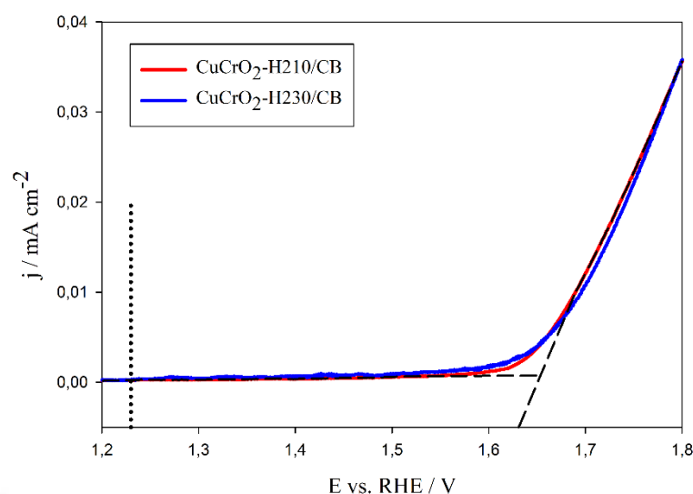
Figure 4.29 Specific activities of \text{CuCrO}_2 oxides synthesized through hydrothermal reaction at 210 and 230 °C.
