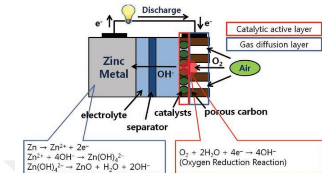
Figure 2.4 Schematic drawing and electrode reactions of zinc-air batteries during discharge [62].
