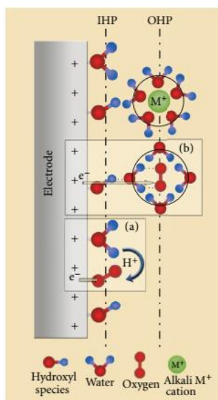
Figure 2.12 Schematic drawing of the double layer at air electrode and electrolyte interface. (a) and (b) shows the inner and outer-sphere e^- transfer processes [80].
