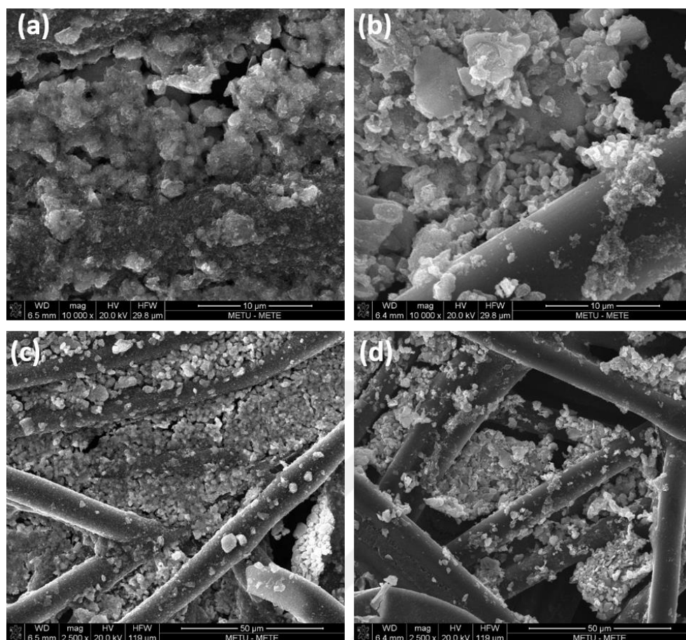
Figure 4.33 SEM micrographs of \text{CuCrO}_2 coated gas diffusion layer (a, c) before and (b, d) after holding at 1.7 V vs. RHE for 1.5 hours.
