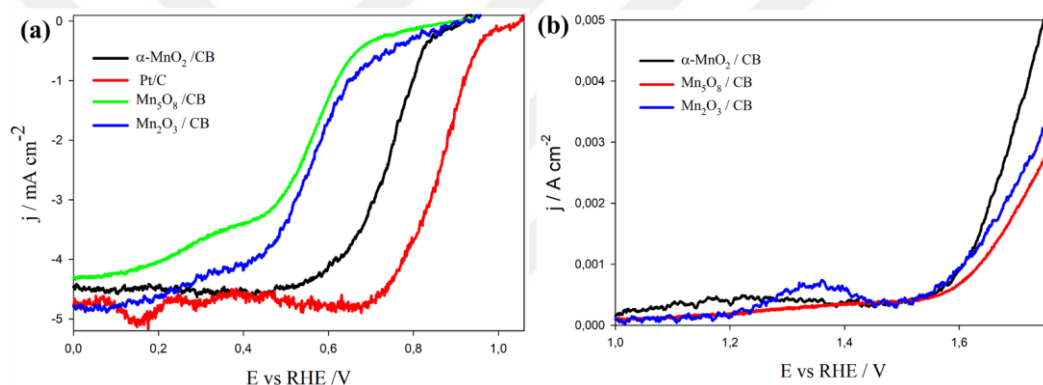
Figure 4.5 Rotating-disk voltammograms of MnO 2 , Mn 5 O 8 , Mn 2 O 3 and Pt/C loaded working electrode in O 2 purged 0.1 M KOH aqueous electrolyte with a sweep rate of 5 mV/s at 1600 rpm: (a) ORR and (b) OER range.
