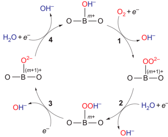
Figure 2.14 The ORR pathway on \text{ABO}_3 type oxides [38], [81].
