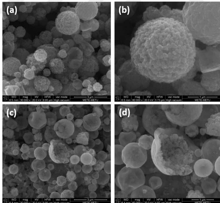
Figure 4.4 SEM images of: (a,b) \text{Mn}_5\text{O}_8 , (c,d) \text{Mn}_2\text{O}_3 powders synthesized through spray pyrolysis method.
