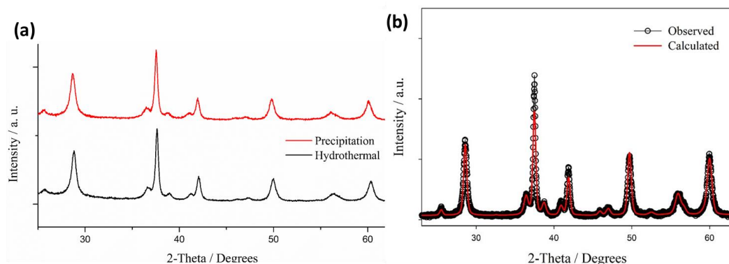
Figure 4.1(a) The XRD spectra of \alpha -MnO 2 powders synthesized by precipitation and hydrothermal methods (b) The XRD spectra and results of Rietveld refinement of precipitated \alpha -MnO 2 powders (ICSD 73363).
