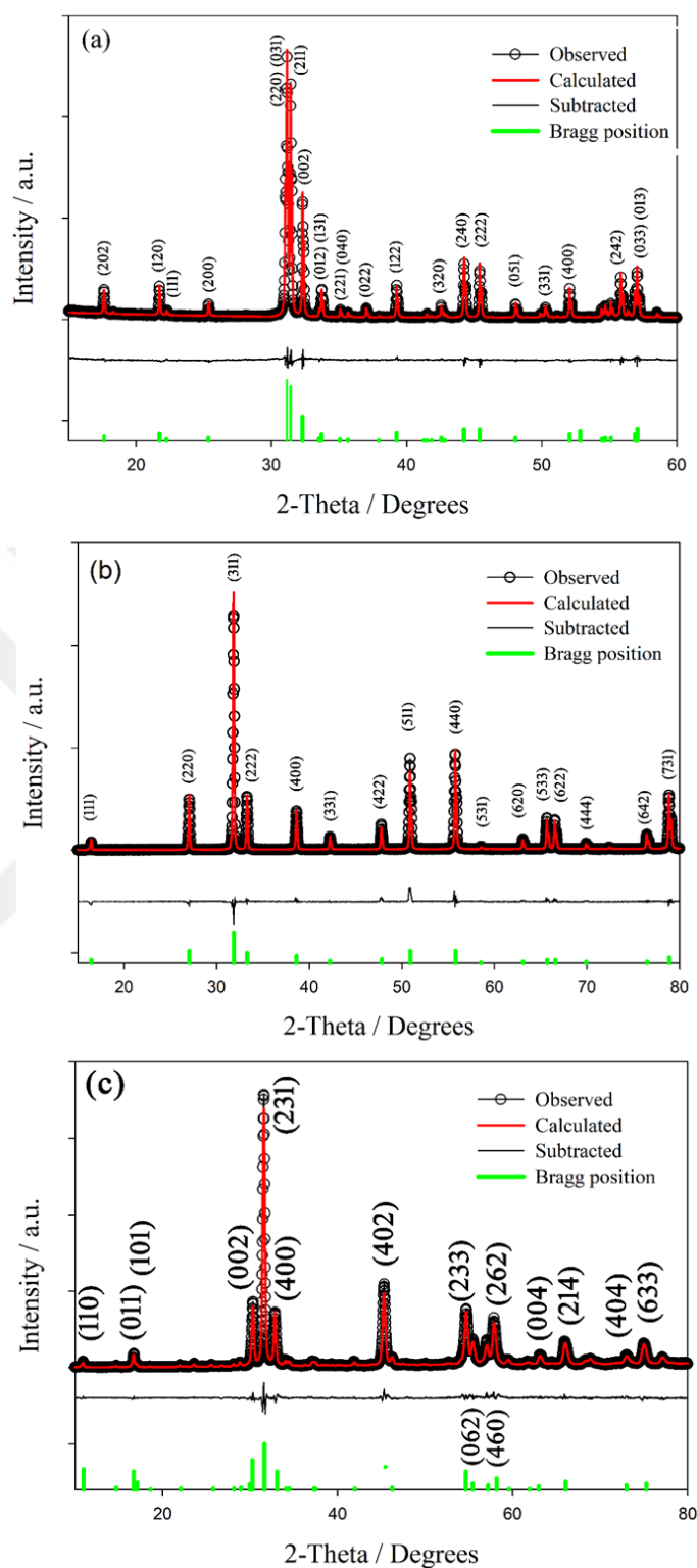
Figure 4.11 The XRD spectra and results of Rietveld refinement of (a) \text{Ag}_2\text{CrO}_4 , (b) \text{Ag}_2\text{MoO}_4 and (c) \text{Ag}_2\text{WO}_4 powders.
