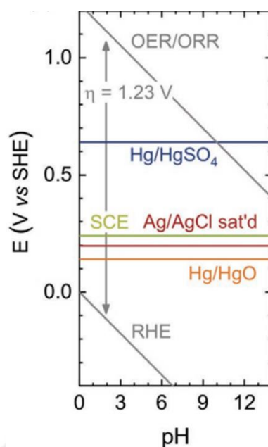
Figure 3.3 The Pourbaix diagram of water with showing potentials of commonly used reference electrodes [93].
