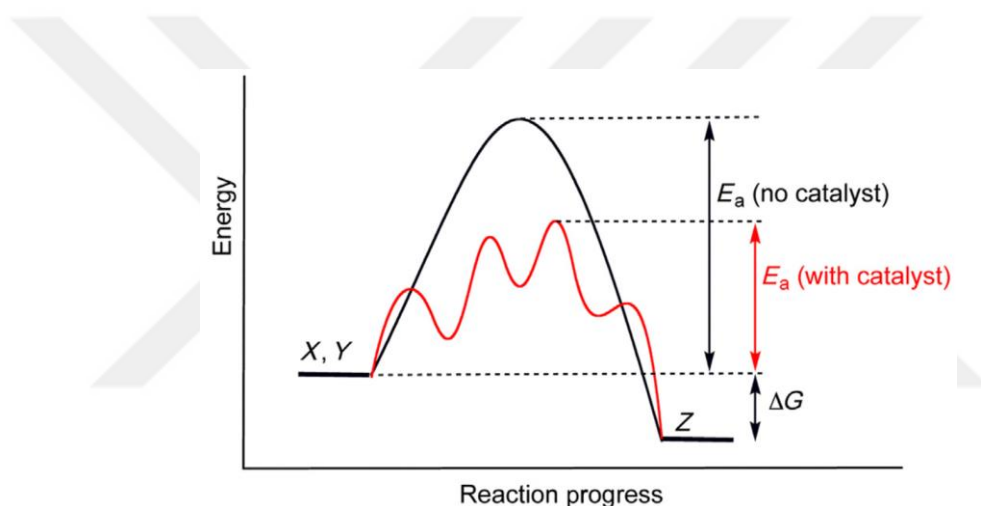
Figure 2.11 Progress of a chemical reaction [78].
