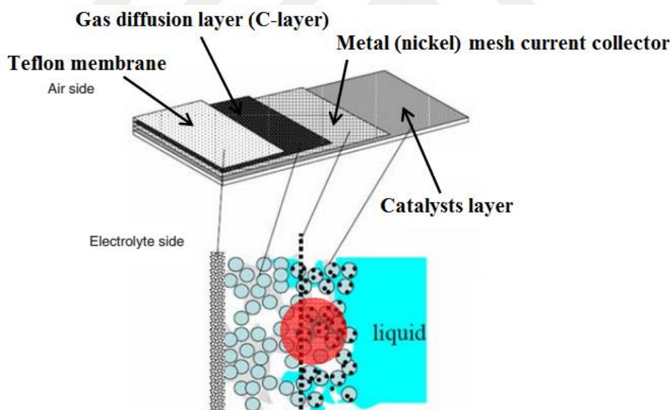
Figure 2.8 Laminated air electrode for zinc-air battery [61], [64].
