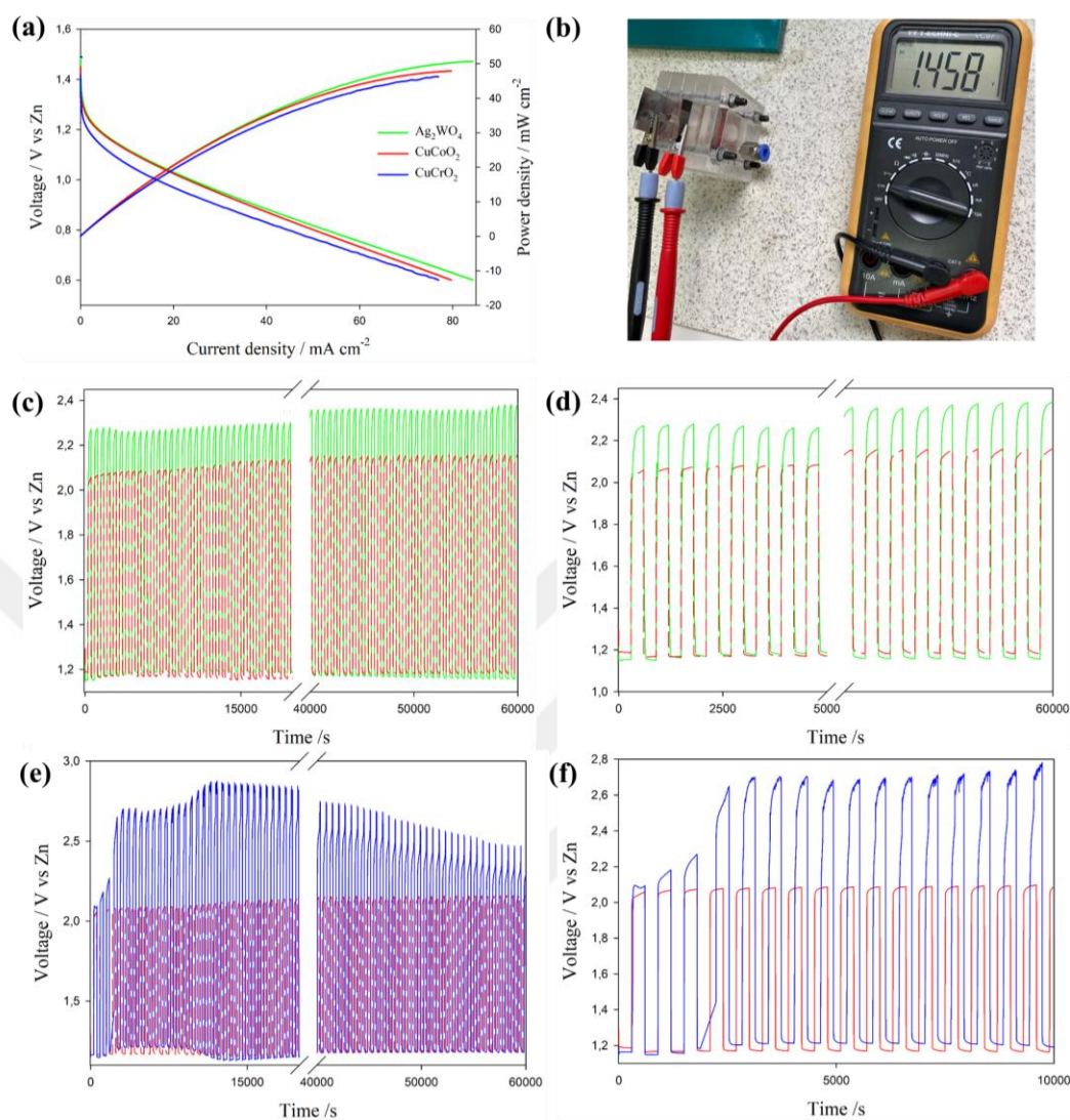
Figure 4.36 (a) Polarization and corresponding power density curves of Ag 2 WO 4 , CuCoO 2 and CuCrO 2 powders. (b) Measured open circuit voltage of the Zn-air battery with CuCrO 2 loaded air cathode. (c) Galvanostatic cycling stability of Zn-air battery with Ag 2 WO 4 and CuCoO 2 loaded air electrode at 5 mA cm -2 . (d) The enlarged version of first and last cycles of (c). (e) Galvanostatic cycling stability of Zn-air battery with CuCrO 2 and CuCoO 2 loaded air electrode at 5 mA cm -2 . (f) The enlarged version of first cycles of (e). The discharge and charge cycle time of galvanostatic cycling stability is 10 minutes.
