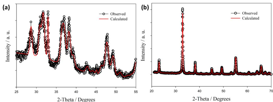
Figure 4.3 The XRD spectra and results of Rietveld refinement of (a) \text{Mn}_5\text{O}_8 powders obtained at 1 st spray experiment (Card number: 1514100) and (b) \text{Mn}_2\text{O}_3 powders obtained at 2 nd spray experiment (Card number: 1514103).
