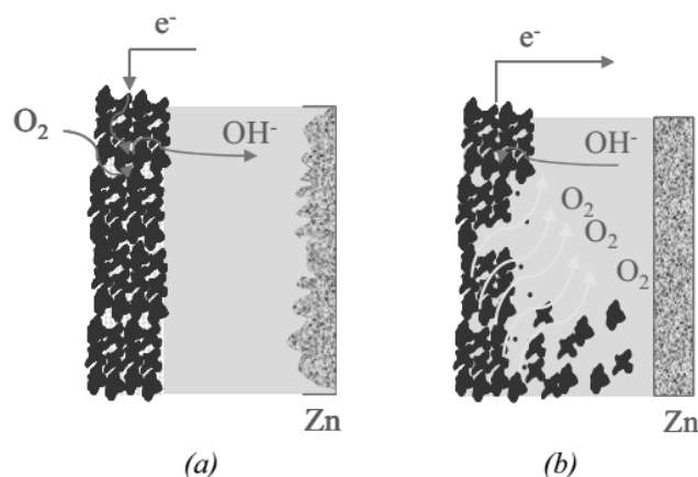
Figure 2.9 Zinc-air cell at (a) charging, and (b) discharging steps [77].
