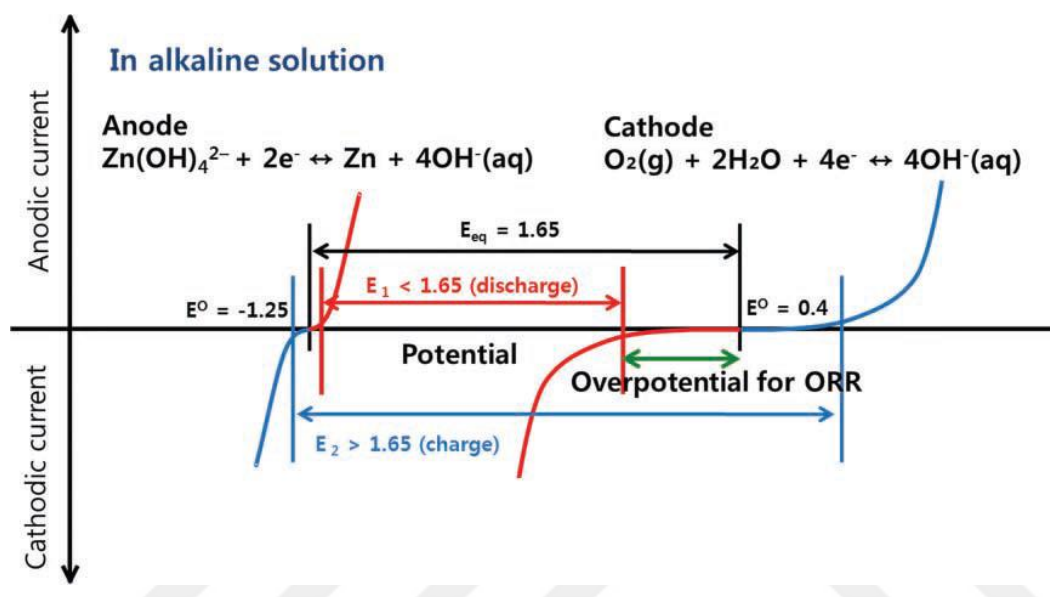
Figure 2.10 Schematic polarization curves of zinc-air battery in aqueous solution. Black lines show the equilibrium potential. Red lines show the potential of zinc-air battery in discharge. Blue lines show the potential of zinc-air battery in charge [62].
