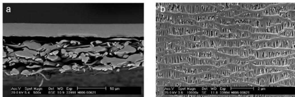
Figure 2.6 (a) Cross-section and (b) microstructure of Celgard 5550 membrane [18].
