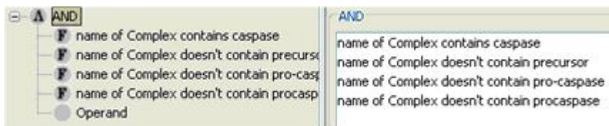
Figure 5.42: Query for Caspase complexes, which does not contain words ‘precursor’, ‘pro-caspase’ or ‘procaspase’
