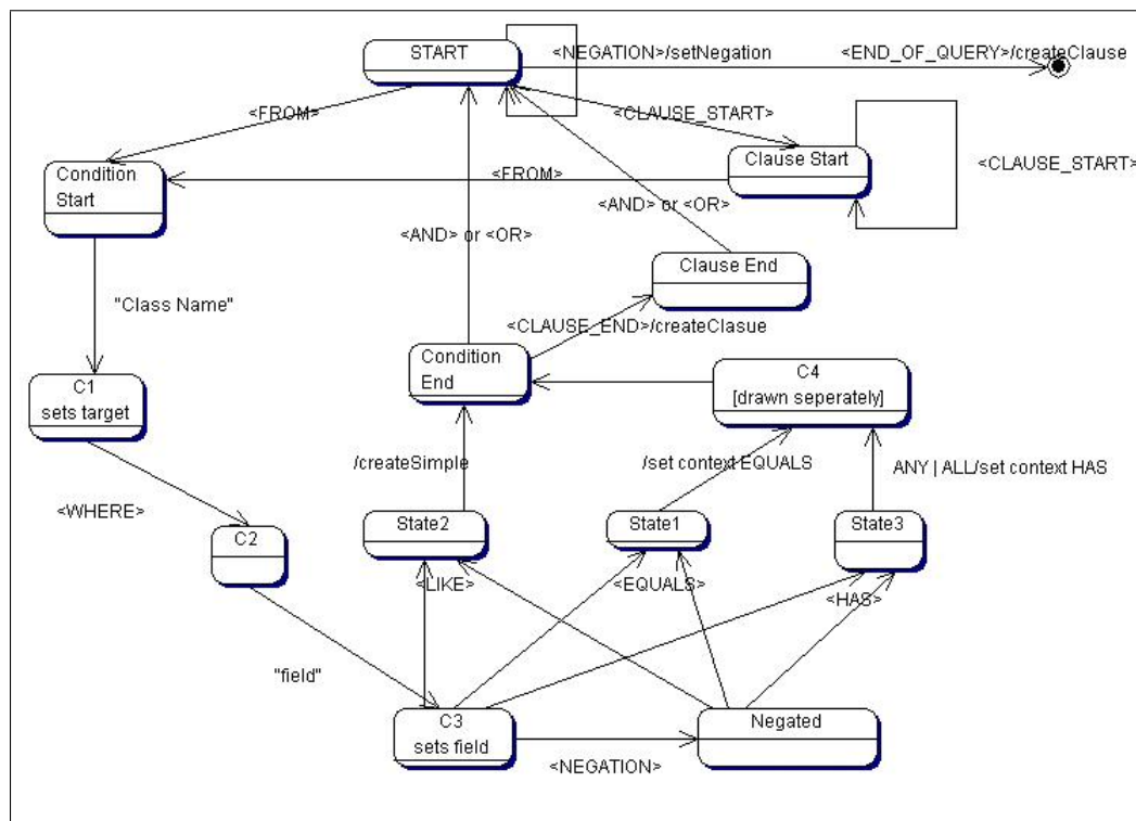
Figure 5.3: General state diagram of FieldQueryParser , for parsing the PATIKA query languages field queries.
