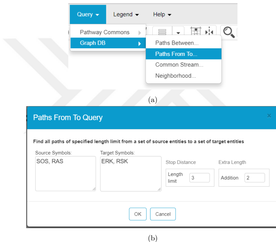
Figure 4.7: (a) Drop-down menu item for Paths-From-To query. (b) Paths-From-To query dialog of Newt.
