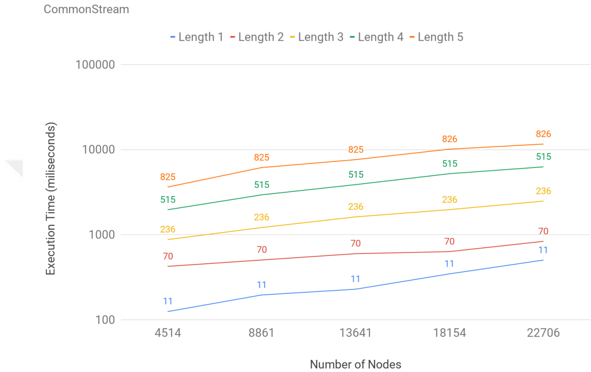
Figure 3.19: Common Stream Procedure - Execution Time vs Number of Nodes chart on large SBGN maps. Notice that the number of edges in returned graphs should be proportional to the number of nodes in SBGN maps.
