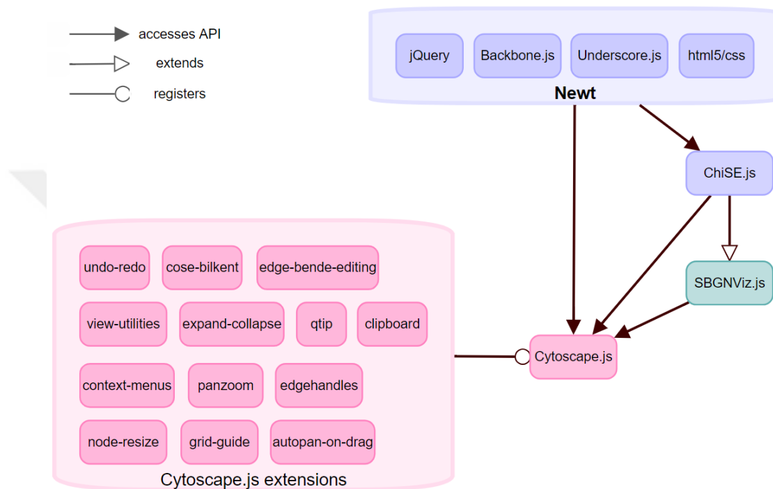
Figure 2.10: Architecture of Newt [5]
