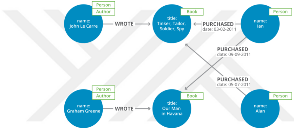
Figure 2.6: Property graph data model example for book store [2]
