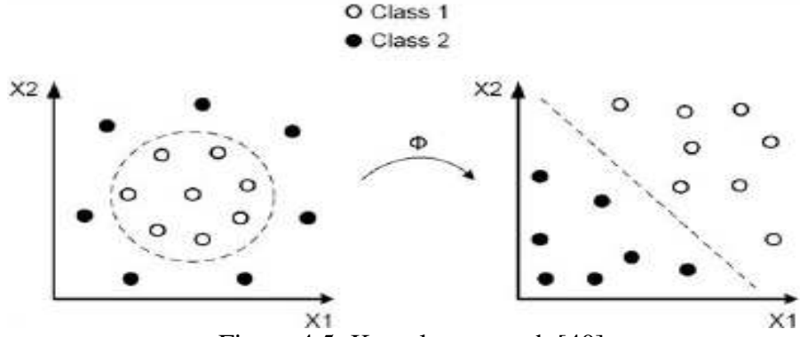
Figure 4.5: Kernels approach [40]
