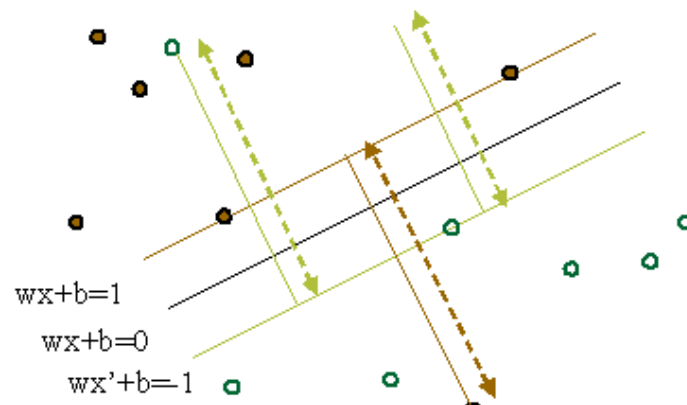
Figure 4.4: SVM hyper planes. [40]
