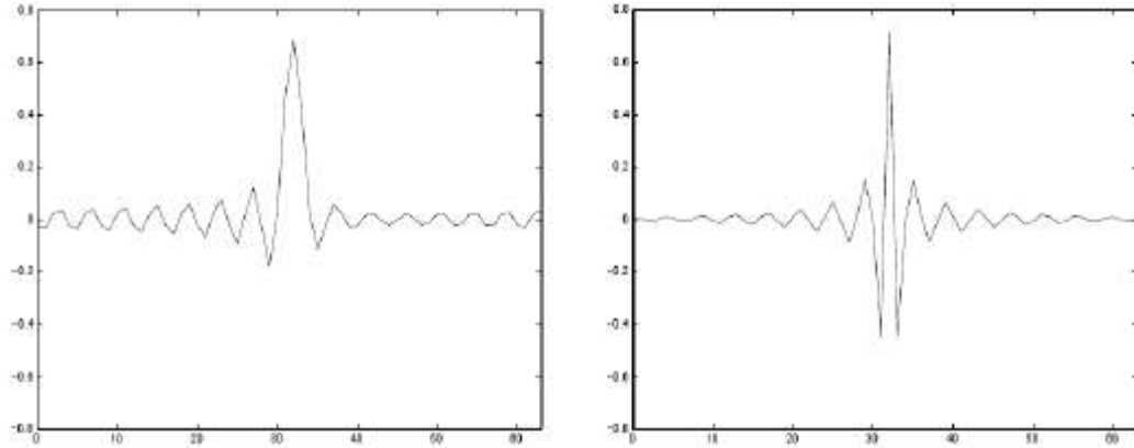
Figure 3.3: Shannon father wavelet (left) and Shannon mother wavelet (right). Notice that the father wavelet has components with lower frequency than the mother wavelet. (adapted from [31]).
