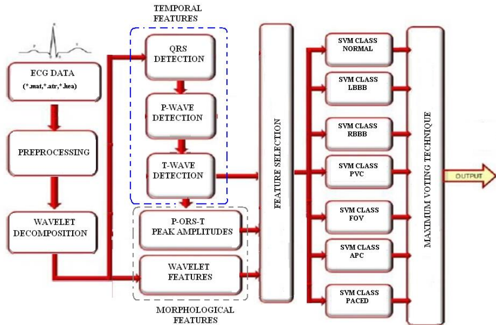
Figure 6.1: Structure of purposed ECG signal processing approach.
