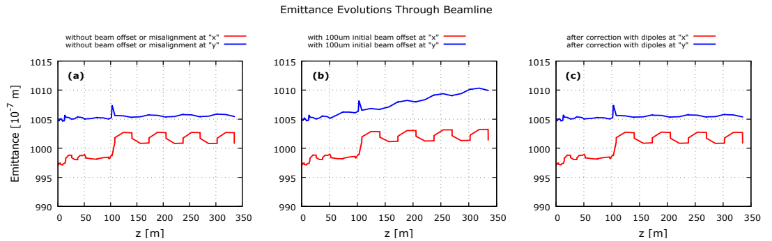
Figure 3.22. Emittance evolutions through beamline for design with 4 FODO cell sections when 100μm initial beam offset and correction of errors with dipole magnets a) without beam offset or misalignment, b) with 100μm initial beam offset, c) after correction with dipoles.
