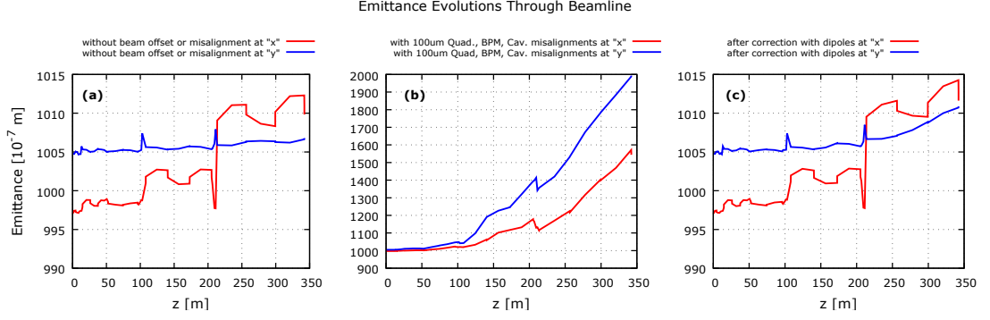
Figure 3.21. Emittance evolutions through beamline for design with 5 FODO cell sections when all components (BPMs, quadrupoles and cavities) 100μm randomly misaligned and correction of errors with dipole magnets a) without beam offset or misalignment, b) with 100μm quadrupole, BPM and cavity misalignments, c) after correction with dipoles.
