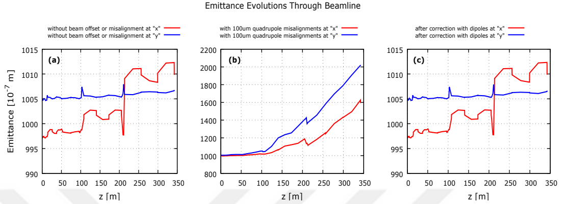
Figure 3.20. Emittance evolutions through beamline for design with 5 FODO cell sections when all quadrupole magnets 100 \mu\text{m} randomly misaligned and correction of errors with dipole magnets a) without beam offset or misalignment, b) with 100 \mu\text{m} quadrupole misalignments, c) after correction with dipoles.
