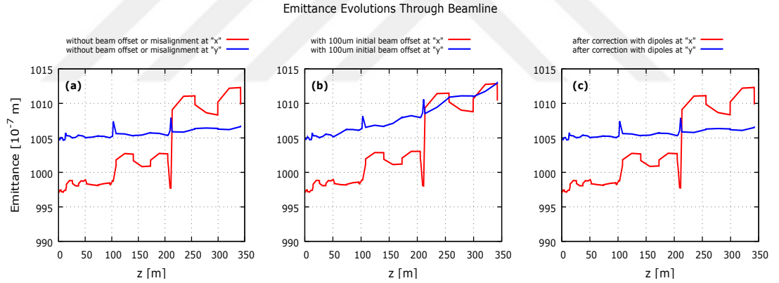
Figure 3.19. Emittance evolutions through beamline for design with 5 FODO cell sections when 100μm initial beam offset and correction of errors with dipole magnets a) without beam offset or misalignment, b) with 100μm initial beam offset, c) after correction with dipoles.
