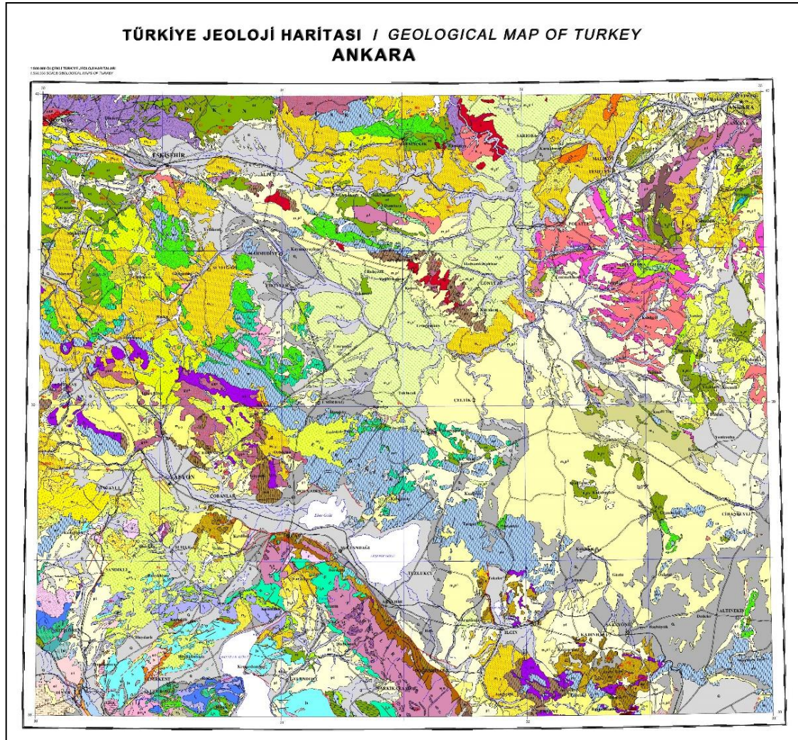
Figure 4.1. Geological map of Ankara including the province of Eskişehir ( http - 3 )
