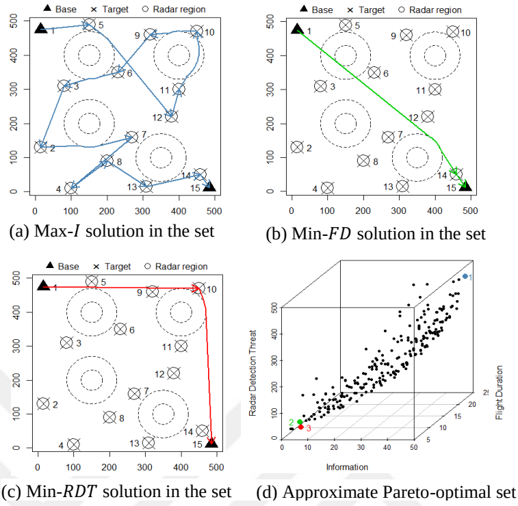
Figure 5.6: Approximation of the Pareto-optimal set of the 15-node problem
