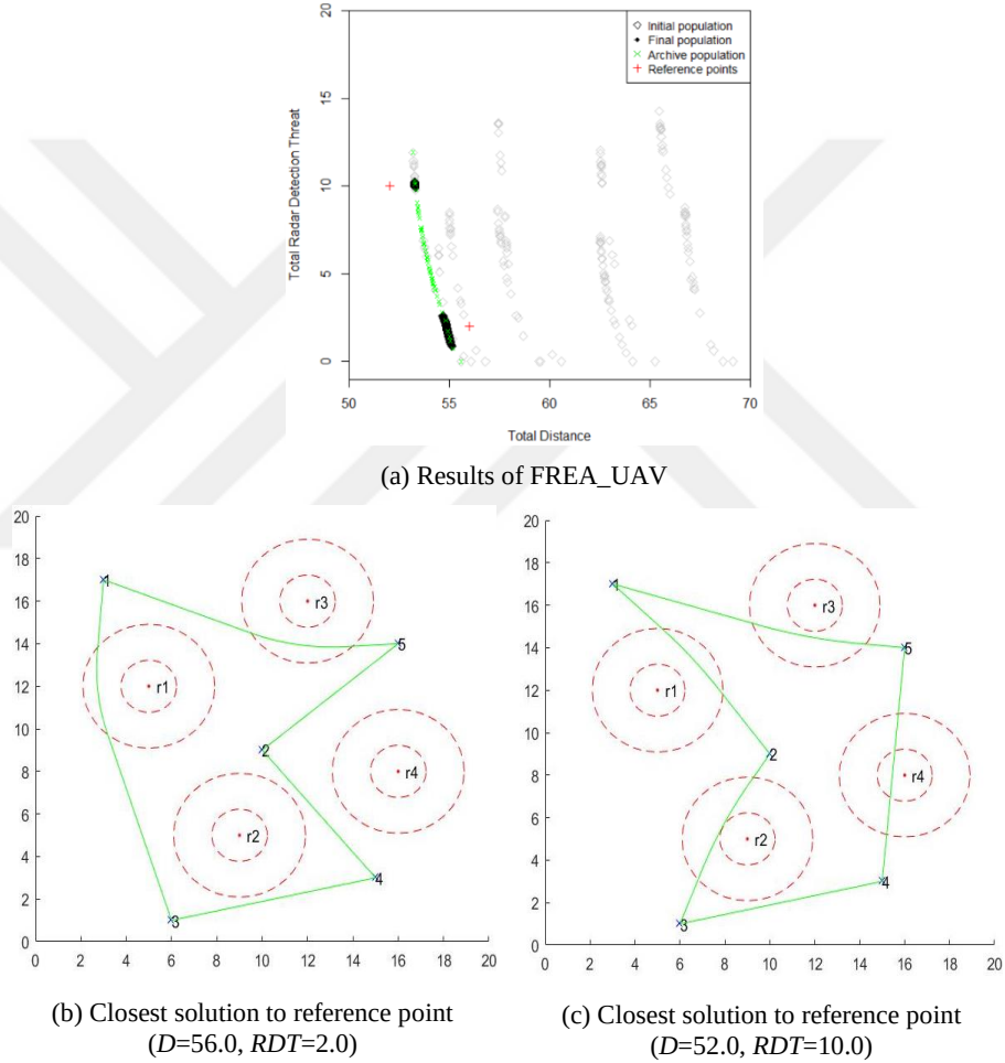
Figure 3.13: Results for the 5-Target UAV route planning problem
