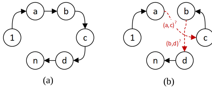
Figure 5.3: An example of the modified 2-opt improvement heuristic
