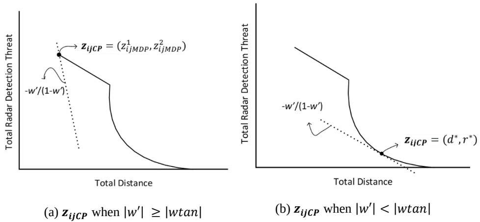
Figure 3.7: Finding z_{ijCP}
