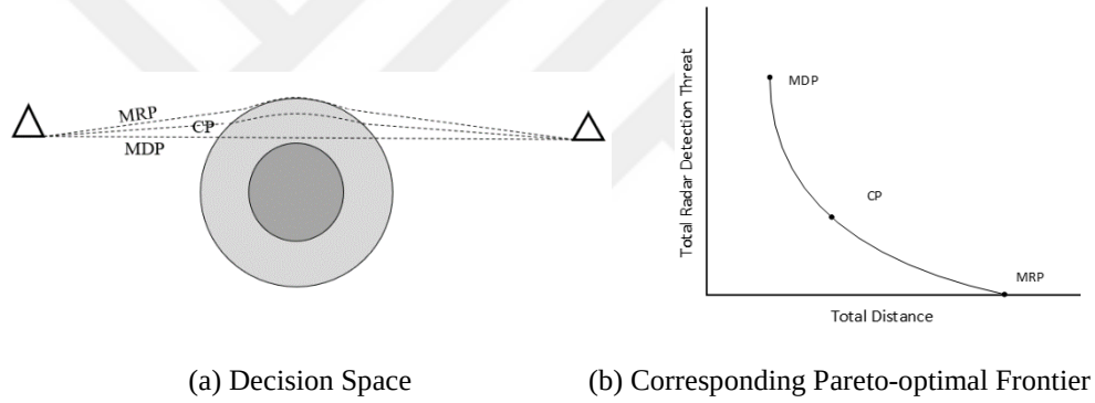
Figure 3.2: Movement Type 2
