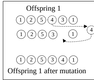
Figure 3.10: Mutation operator
