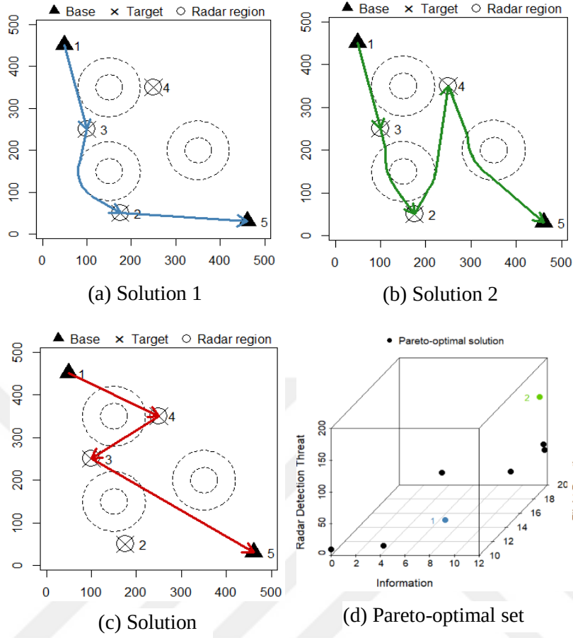
Figure 5.2: Several routes and the Pareto-optimal set of an example problem
