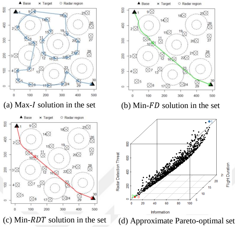
Figure 5.7: Approximation of the Pareto-optimal set of the 30-node problem
