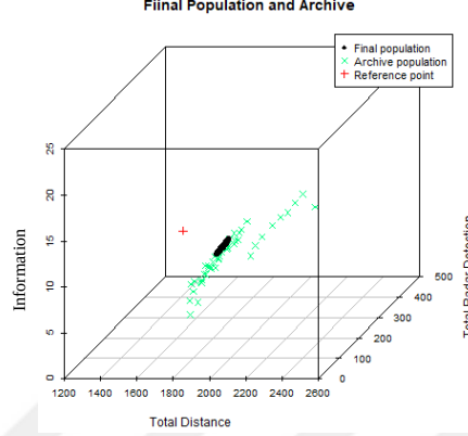
Figure 4.3: Results of the 3-objective 5-Target UAV route planning problem for the reference point ( D=1800 , RDT=50 , I=15 )
