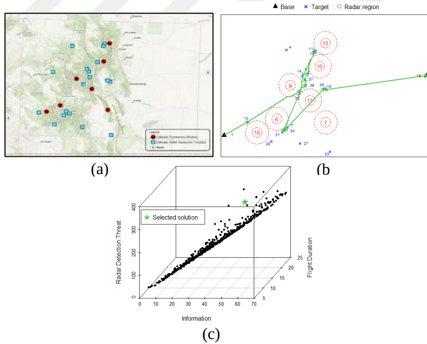
Figure 5.10: Colorado Problem Instance 2: (a) Map, (b) Route of the selected solution, (c) Pareto-optimal set.
