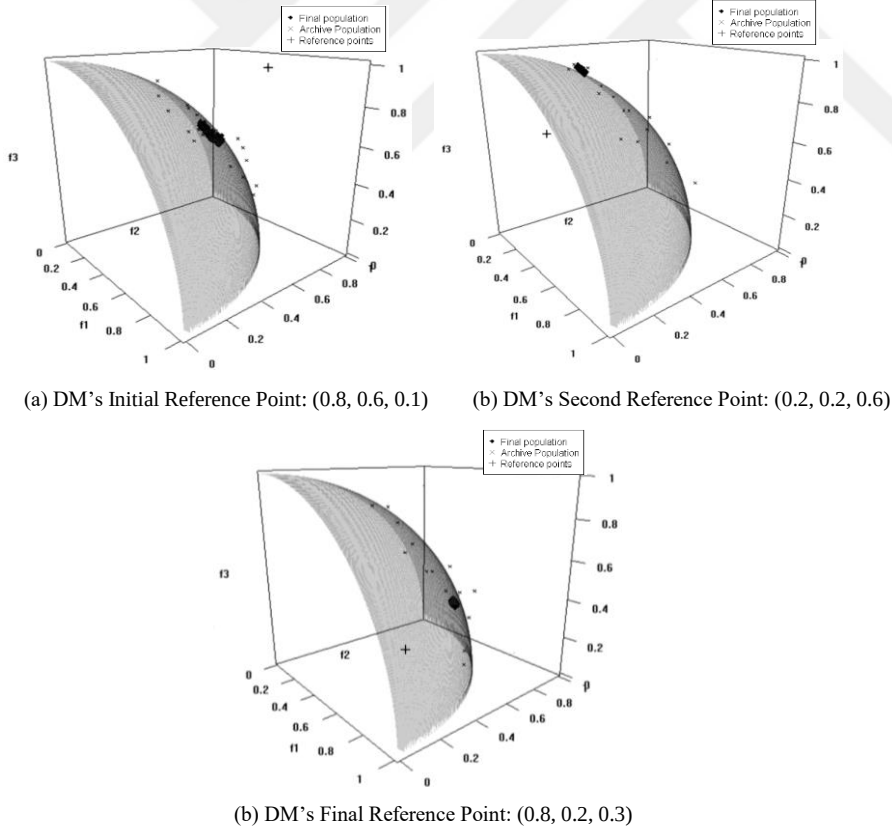
Figure 3.5: Changing reference points in FREA for DTLZ2
