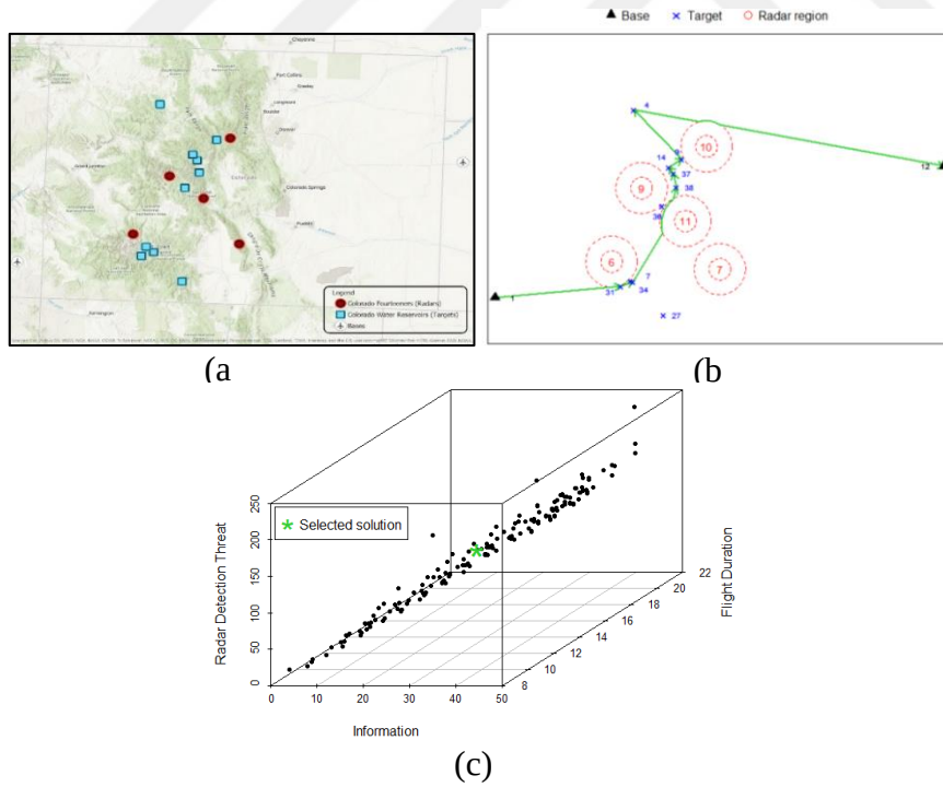
Figure 5.9: Colorado Problem Instance 1: (a) Map, (b) Route of the selected solution, (c) Pareto-optimal set.
