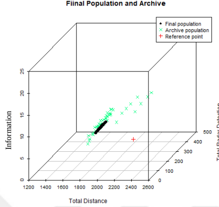
Figure 4.4: Results of the 3-objective 5-Target UAV route planning problem for the reference point ( D=2200 , RDT=200 , I=5 )
