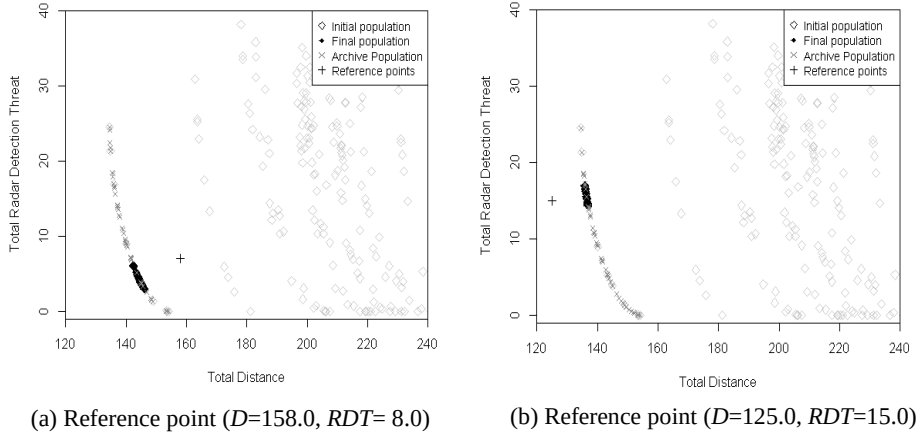
Figure 3.17: Results for the 15-Target UAV route planning problem
