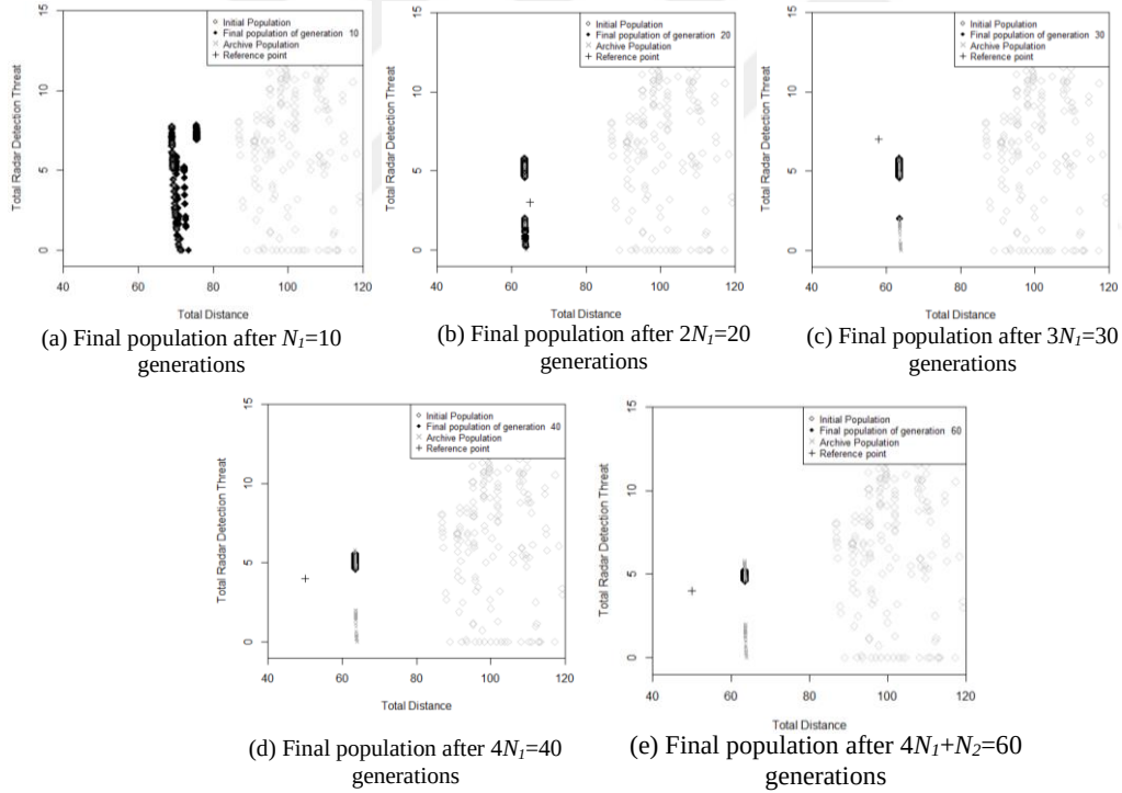
Figure 3.19: Changing reference points - Second scenario
