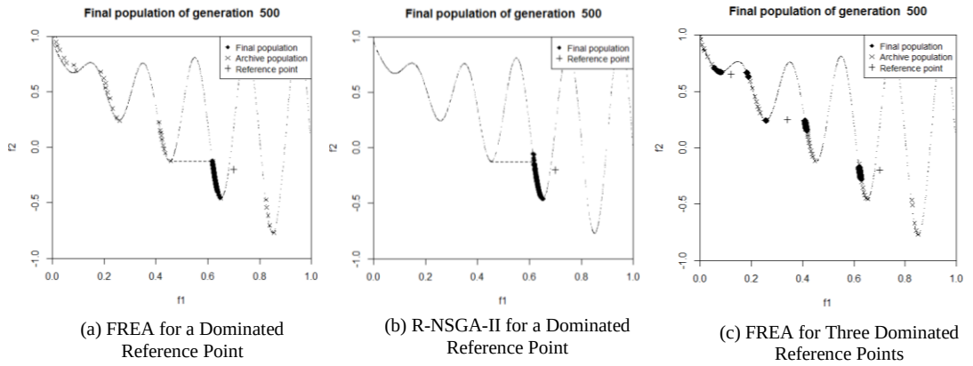
Figure 3.4: Results for ZDT3
