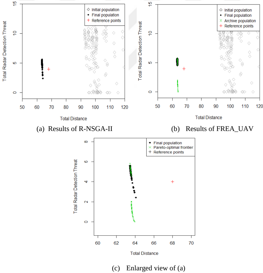
Figure 3.16: Comparison of R-NSGA-II and FREA_UAV on the 9-Target UAV route planning problem
