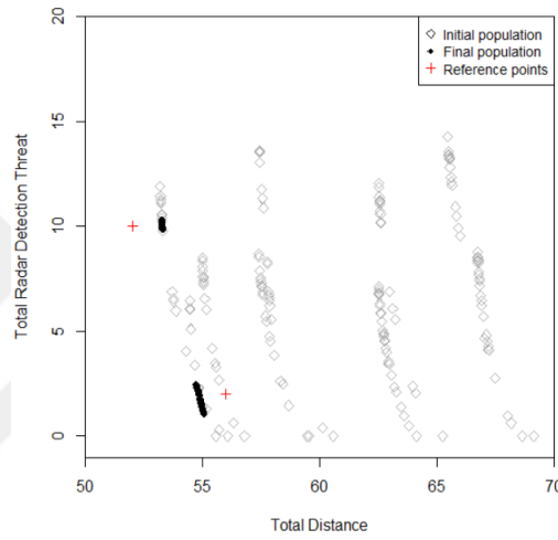
Figure 3.14: Results of R-NSGA-II for the 5-Target UAV route planning problem
