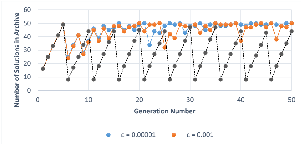
Figure 3.12: The effects of using different \epsilon values for archive for the 5-Target UAV route planning problem
