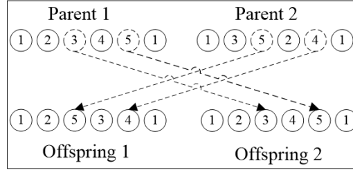
Figure 3.9: POS crossover
