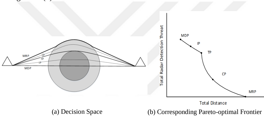
Figure 3.3: Movement Type 3
