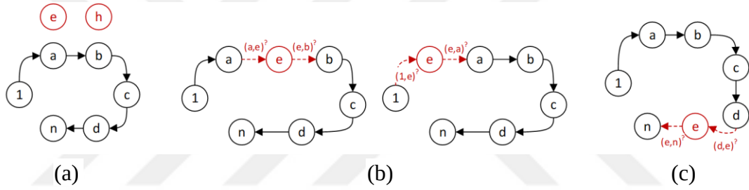
Figure 5.4: An example for node insertion improvement
