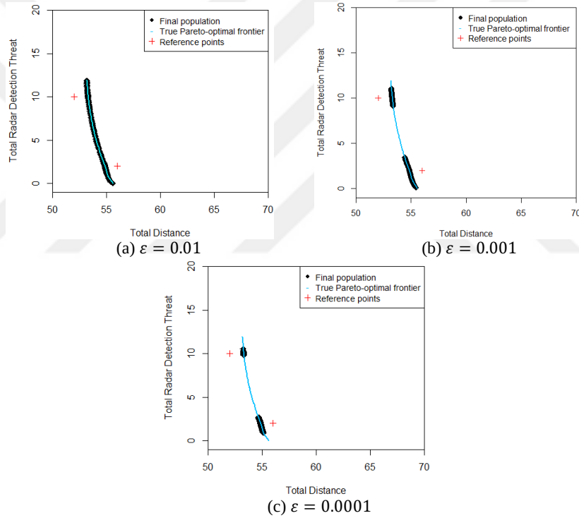
Figure 3.11: The effects of different \varepsilon values on the distribution of the final set for the 5-Target UAV route planning problem
