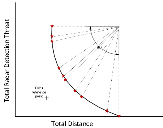
Figure 3.8: Selecting representative points
