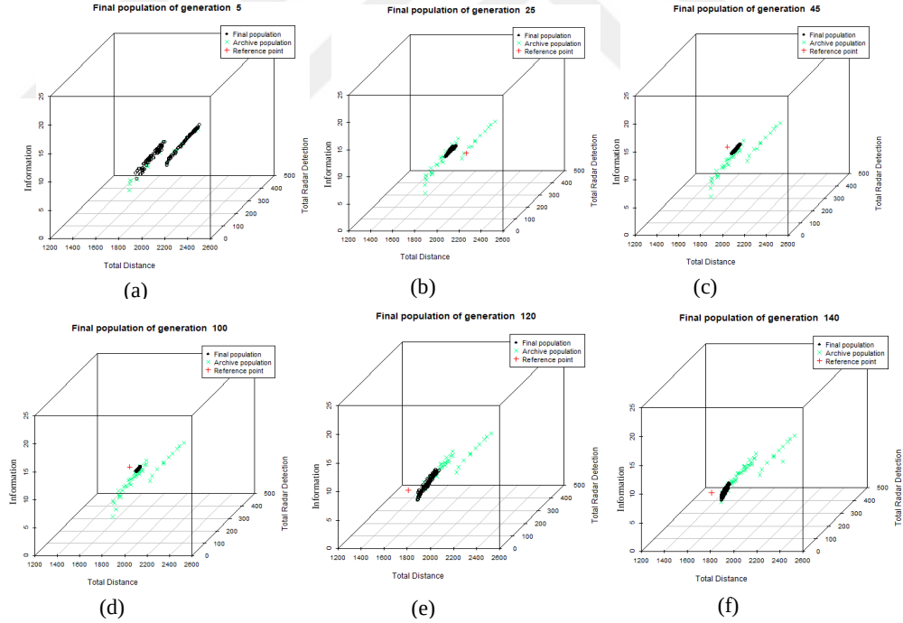
Figure 4.5: Changing reference points: 3-Objective 5-Target UAV route planning problem
