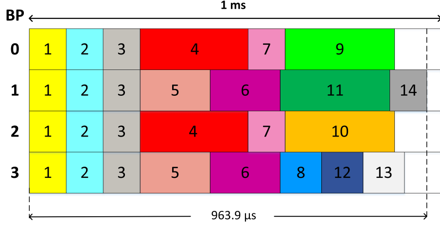
Figure 4.5: MVB Schedule with MLB for S2T
