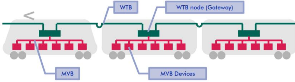
Figure 2.1: TCN Architecture
