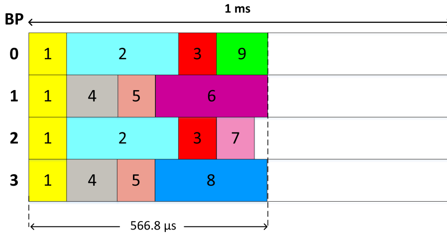
Figure 4.2: MLB schedule after SMB
