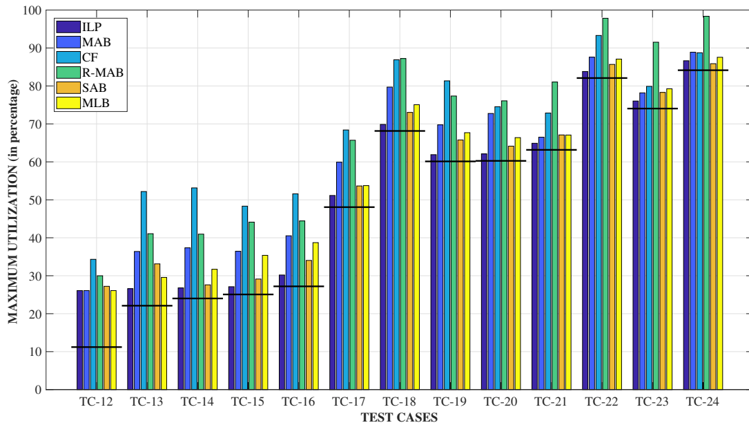
Figure 3.15: Maximum Utilization in Normal Test Cases
