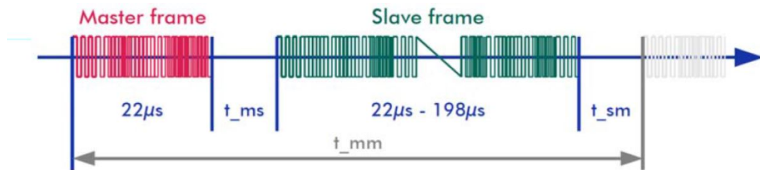
Figure 2.3: Telegram Structure and Timing
