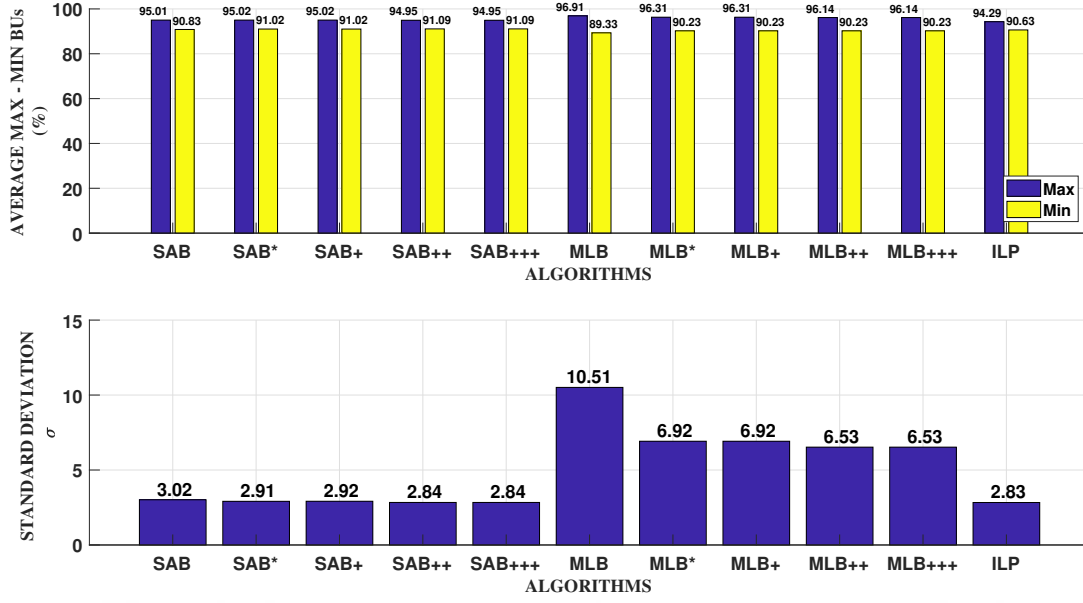
Figure 4.9: Performance Metrics for TC-11
