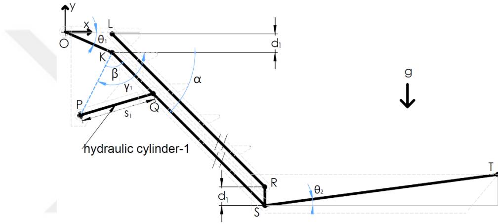
Figure 5.1 Schematic of the gangway transforming mechanism
