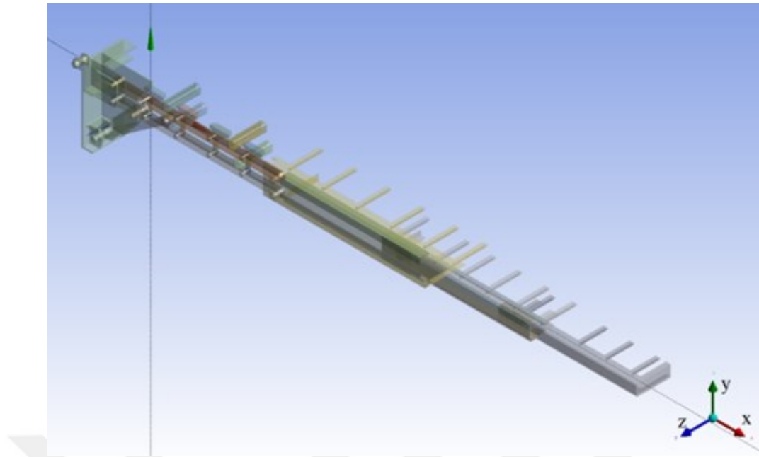
Figure 6.1 Half-geometry of the fully-extended gangway
