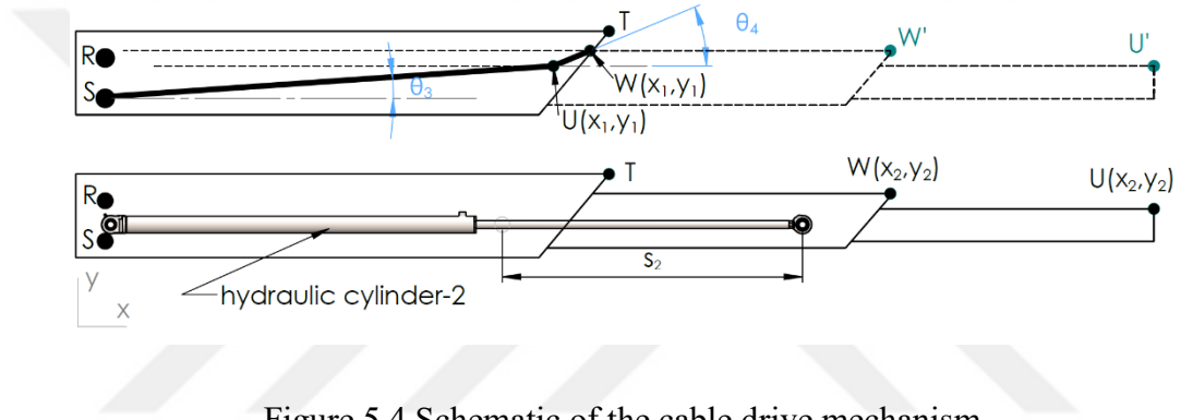
Figure 5.4 Schematic of the cable drive mechanism
