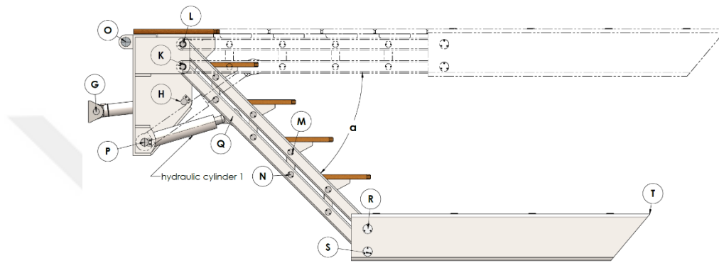
Figure 4.1 Side view of the gangway transforming mechanism
