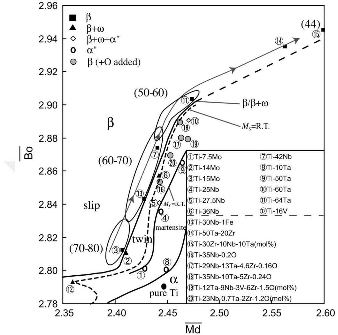
Figure 2.14 Bo-Md diagram in which the \beta/\beta+\omega phase boundary is shown together with the boundaries. Young's modulus (GPa) is given in parentheses for typical alloys [34].
