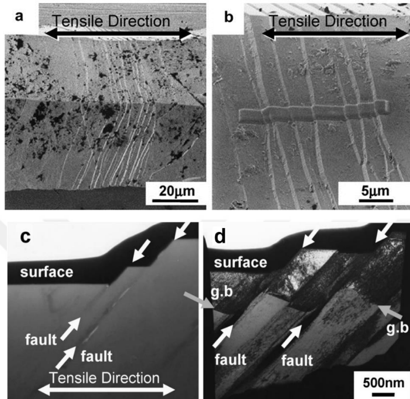
Figure 2.18 Giant Faults on the free surface (a, b) and longitudinal section (c, d) of the deformed surface of Gum metal [62].
