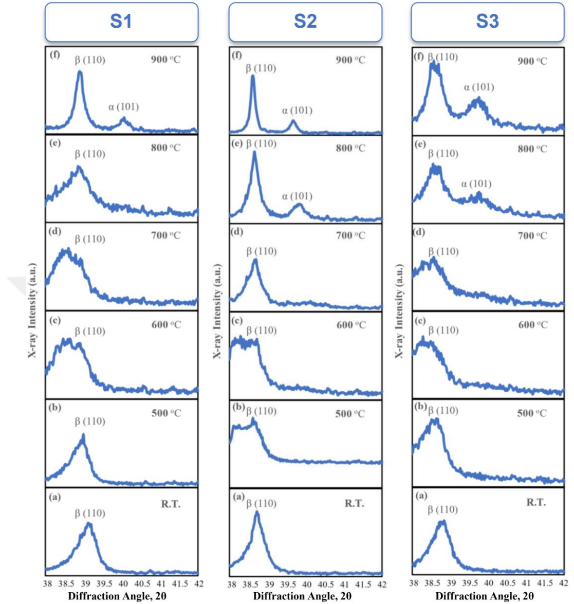
Figure 4.11 In-situ thermal XRD analysis of 85% cold deformed S1 (Ti-23.8Nb-2Zr-1.2O), S2 (Ti-23Nb-0.93V-2Zr-1.2O) and S3 (Ti-25Nb-0.7Ta-2Zr-2Al-1.2O) alloys at different temperature.
