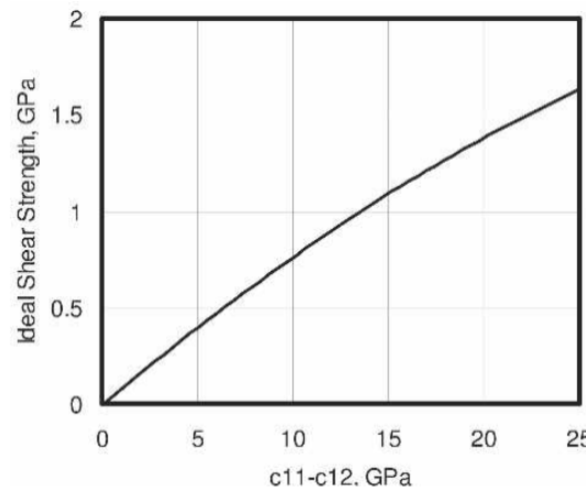
Figure 2.15 Ideal Shear Strength vs C_{11} - C_{12} graph [11].
