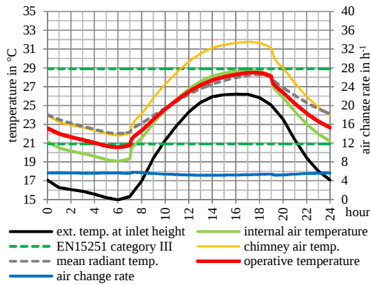
Figure 6.13: Outputs for extreme summer conditions in Stuttgart sized for 5 ACH \triangleq A_{\text{chi}} = 23,3 \text{ m}^2 .
