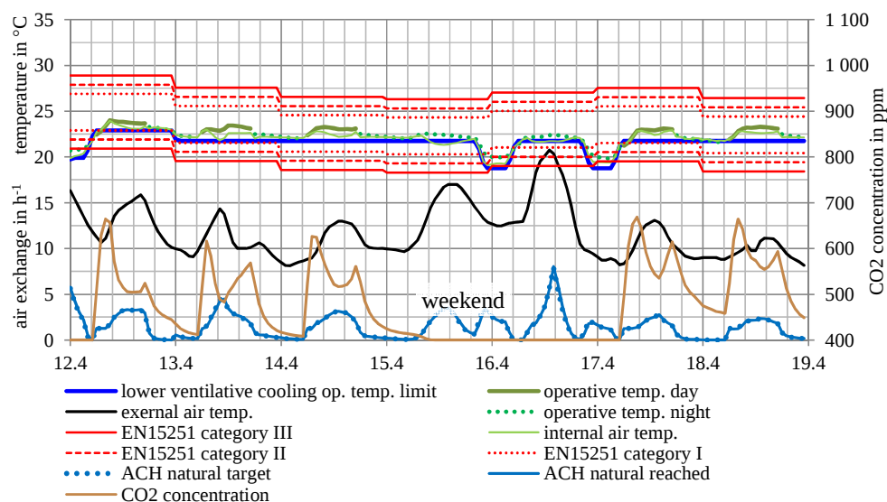
Figure 3.37: Resulting EMS controlled air change rate for a typical spring week in Istanbul.
