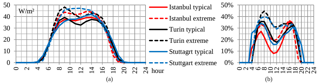
Figure B.9: Hourly SWMD (a) total transmitted solar radiation for Canyon building without external shading devices per m 2 net office floor area and (b) the direct beam solar radiation share.
