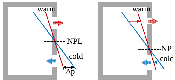
Figure 2.24: Pressure distribution and NPL for two openings buoyant flow with the same and different opening areas.
