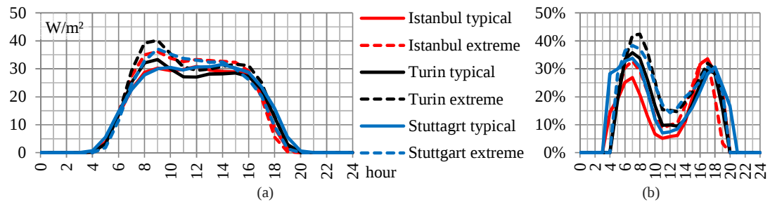
Figure B.10: Hourly SWMD (a) total transmitted solar gains for Canyon building with the actual shading devices per m 2 net office floor area and (b) the direct beam solar radiation share.
