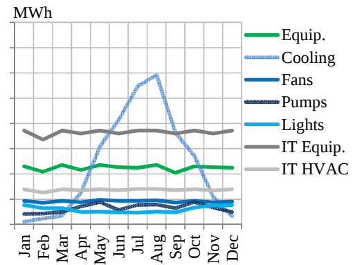
Figure 6.22: Monthly simulated electricity consumption of the different consumers.
