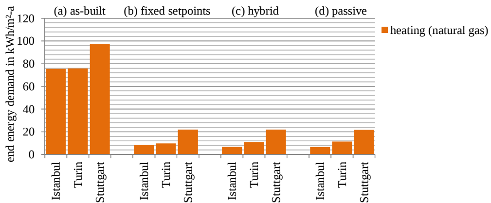
Figure 7.28: Simulated natural-gas consumption of the mechanically and passively cooled base-case scenarios.
