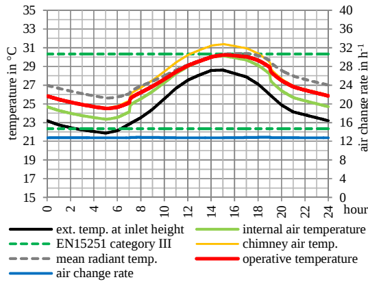
Figure 6.9: Outputs for extreme summer conditions in Istanbul sized for 13 ACH \triangleq A_{\text{chi}} = 29,4 \text{ m}^2 .
