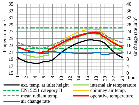
Figure 6.12: Outputs for typical summer conditions in Turin sized for 13 ACH \triangleq A_{\text{chi}} = 93,4 \text{ m}^2 .
