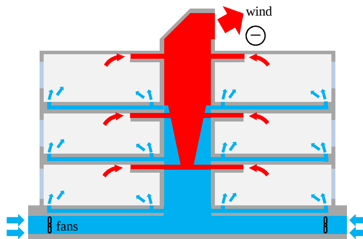
Figure 2.9: ‘Termite’ chimney ventilation example.
