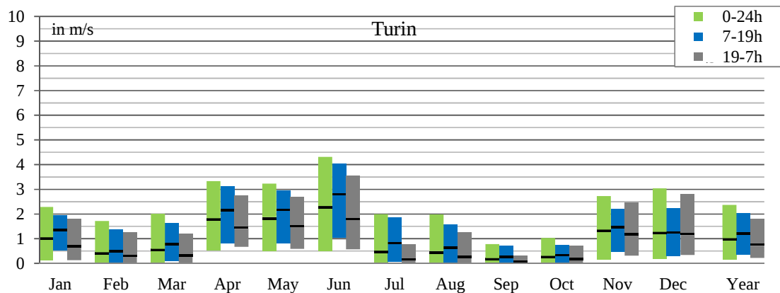
Figure 5.5: Average daily mean (black bar), daily maxima and daily minima wind velocity in Turin according to [141].
