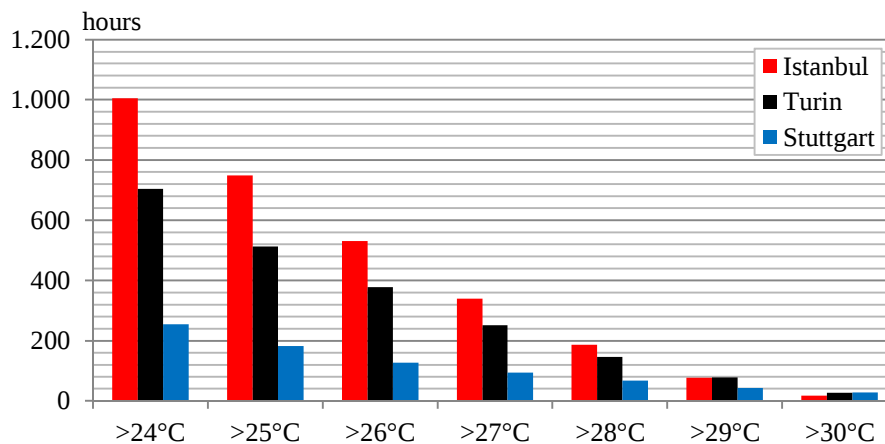
Figure 5.14: Excess frequency of fixed outdoor temperature [141] limits.
