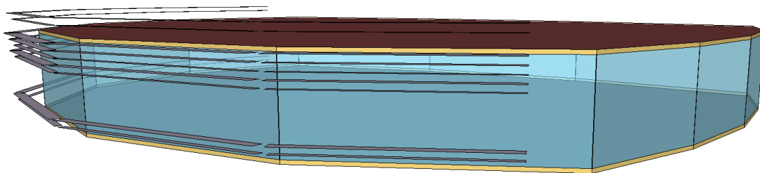
Figure B.8: EnergyPlus simulation model for gathering the transmitted solar radiation of one storey of the Canyon building with the as-built external shading and the glazing ratio of ~ 91 % (~ SE view).
