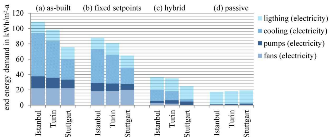
Figure 7.27: Simulated electricity consumption of the mechanically and passively cooled base-case scenarios.
