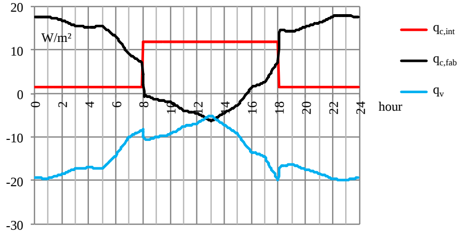
Figure B-2: Typical heat flux balance of the cell air per m 2 net office floor area (850 m 2 ).
