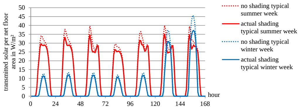
Figure 4.12: Simulated effectiveness of the actual shading devices in a typical summer and winter week period according to the ASHRAE IEWC weather data (storey net floor area = 1 000m 2 ).
