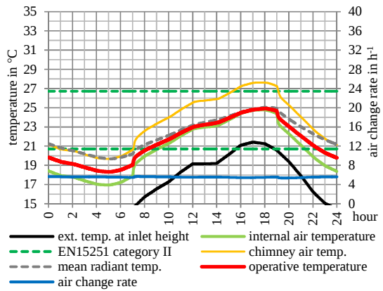
Figure 6.14: Outputs for typical summer conditions in Stuttgart sized for 5 ACH \triangleq A_{\text{chi}} = 23,3 \text{ m}^2 .
