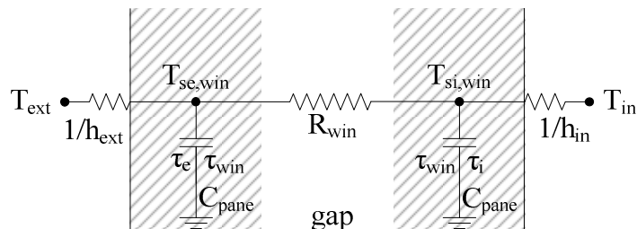
Figure 3.18: RC-model for the windows.
