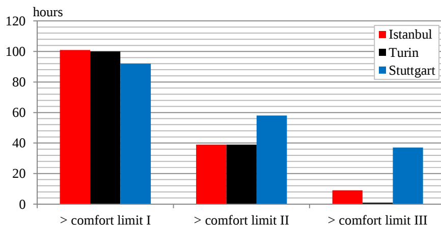
Figure 5.15: Excess frequency of outdoor temperature [141] limits above climate specific upper adaptive comfort category limits [41].
