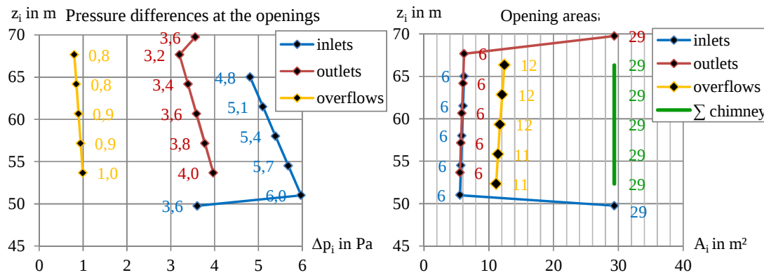
Figure 3.4: Example of the steady state ( \Delta T=3^{\circ}\text{C} , v_{\text{met}} = 5 \text{ m/s} ) ventilation design major outputs for a 5-storey building segment with a internal chimney, sized for 13 air changes per hour
