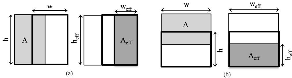
Figure 2.10: Geometrical representations of horizontally (a) and vertically (b) movable sliding windows and their resulting effective opening area, height, and width.
