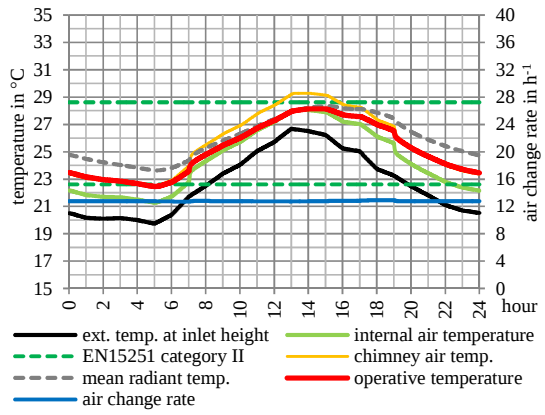
Figure 6.10: Outputs for typical summer conditions in Istanbul sized for 13 ACH \triangleq A_{\text{chi}} = 29,4 \text{ m}^2 .
