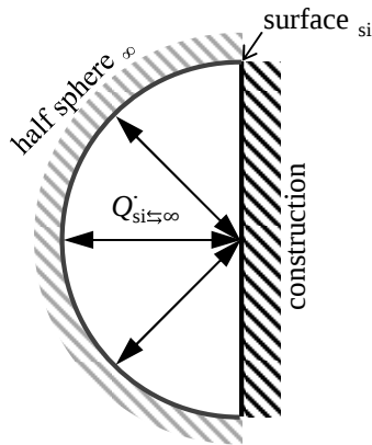
Figure 3.21: Long wave radiation exchange at the interior surfaces.
