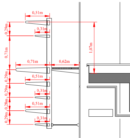
Figure 4.11: External shading device drawing detail.
