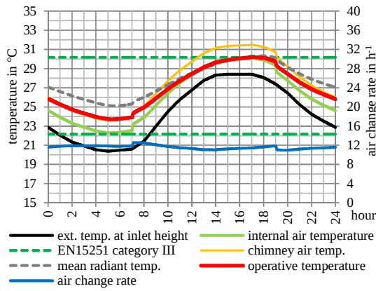
Figure 6.11: Outputs for extreme summer conditions in Turin sized for 13 ACH \triangleq A_{\text{chi}} = 93,4 \text{ m}^2 .
