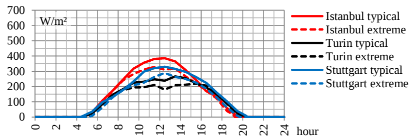
Figure 5.26: SWMD external horizontal diffuse solar radiation profiles.
