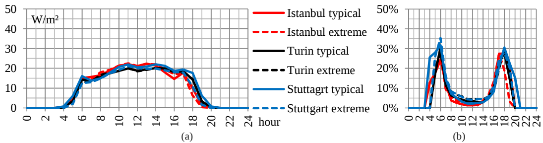
Figure B.11: Hourly SWMD (a) total transmitted solar gains for Canyon building with adaptive blinds per m 2 net office floor area and (b) the direct beam solar radiation share.
