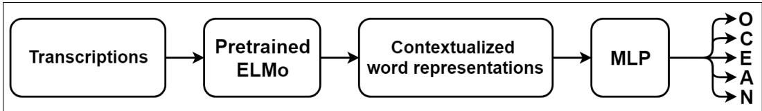
Figure 3.6: The transcription feature-based neural network.
