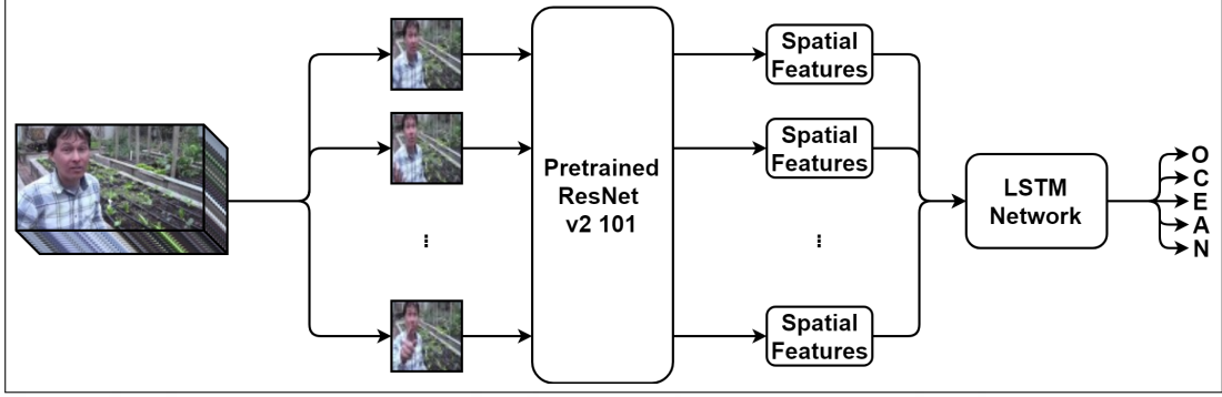
Figure 3.3: The ambient feature-based neural network.
