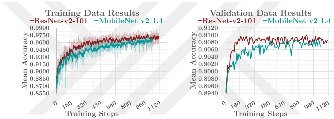
Figure 4.13: The results for ResNet-v2-101 and MobileNetV2 (1.4) networks.
