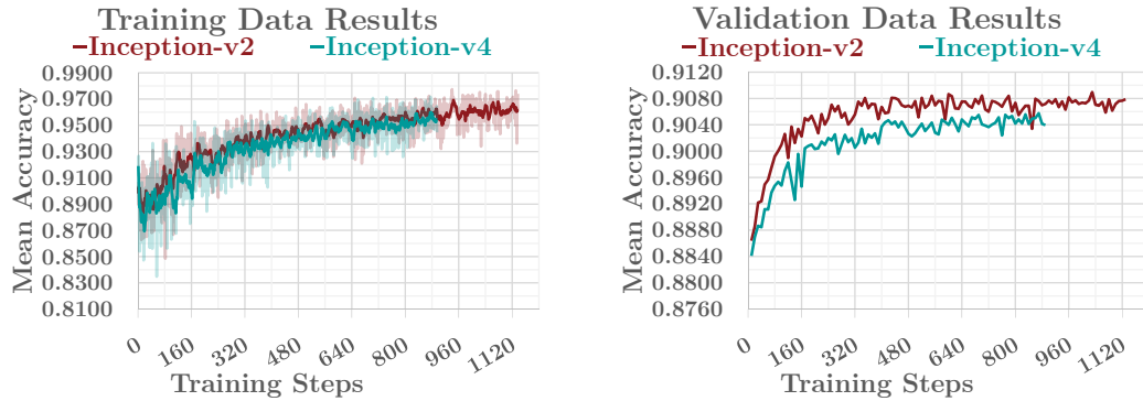
Figure 4.7: The results for Inception-v2 vs. Inception-v4 networks.
