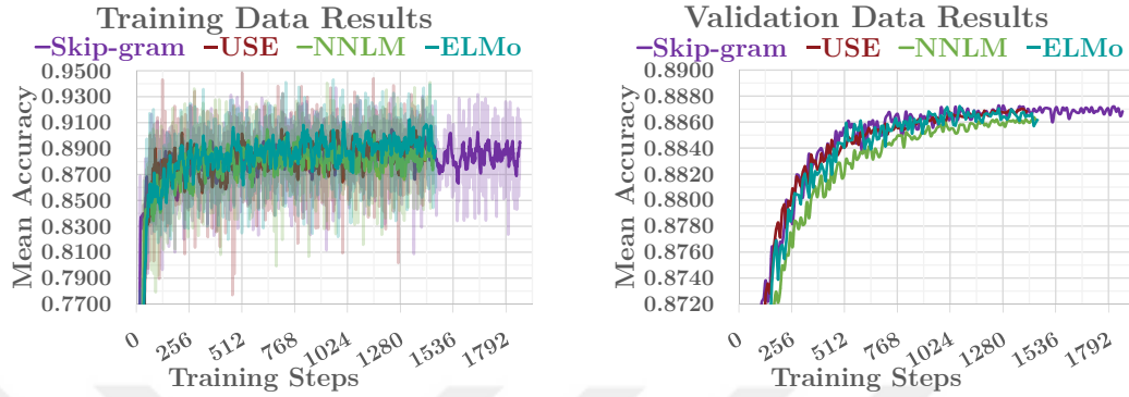
Figure 4.20: The results of various models used for transcription input.
