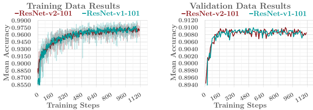
Figure 4.12: Comparison of ResNet-v2-101 and ResNet-v1-101 networks.
