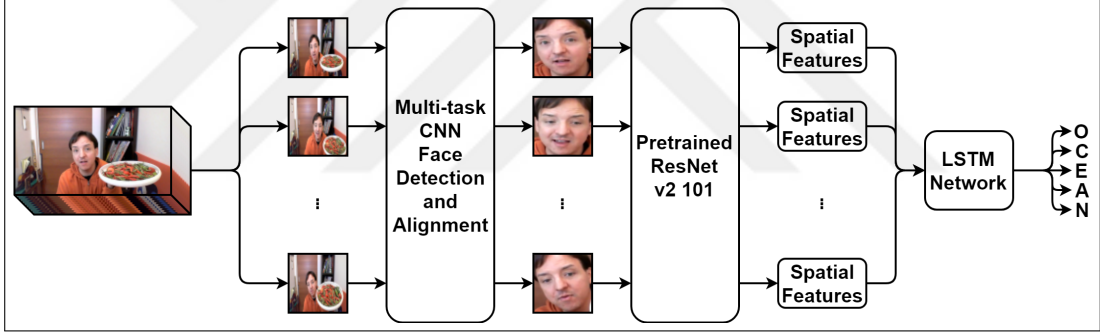
Figure 3.4: The facial feature-based neural network.
