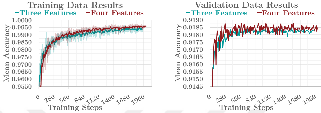
Figure 4.24: The comparison of the three and four feature-based networks. The four-feature network uses ambient, audio, facial, and transcription features.
