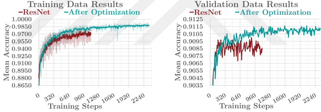
Figure 4.15: The results of ResNet-v2-101 network after hyperparameter and LSTM network optimization.
