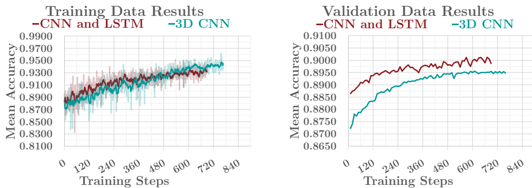
Figure 4.4: The results for 3D-CNN and CNN-LSTM networks.
