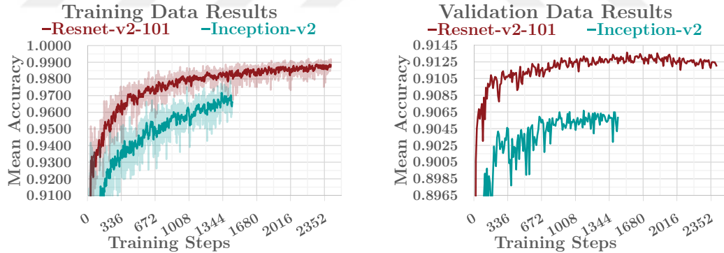
Figure 4.18: The results for ResNet-v2-101 and Inception-v2 networks using face aligned images.
