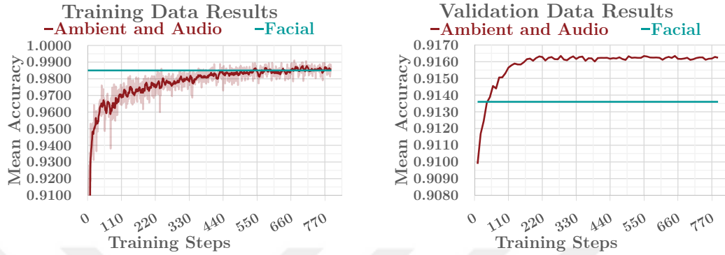
Figure 4.22: The results of the simple multimodal network consisting of ambient feature-based and audio feature-based subnetworks with early fusion.
