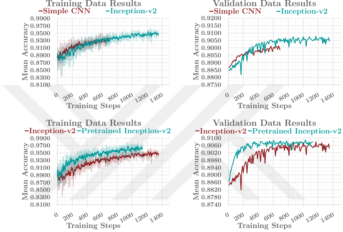
Figure 4.5: The results of training Inception-v2 from scratch compared to simple CNN (top), and fine-tuning the pretrained Inception-v2 model compared to the previous version (bottom).
