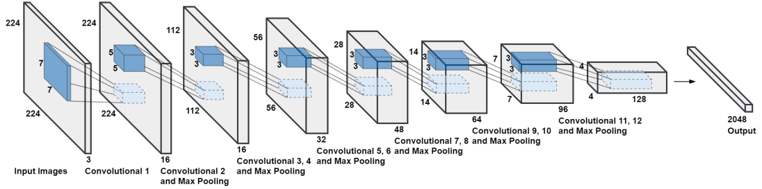
Figure 4.2: Architecture of CNN.
