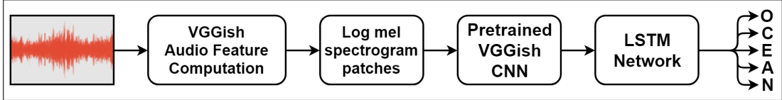
Figure 3.5: The audio feature-based neural network.
