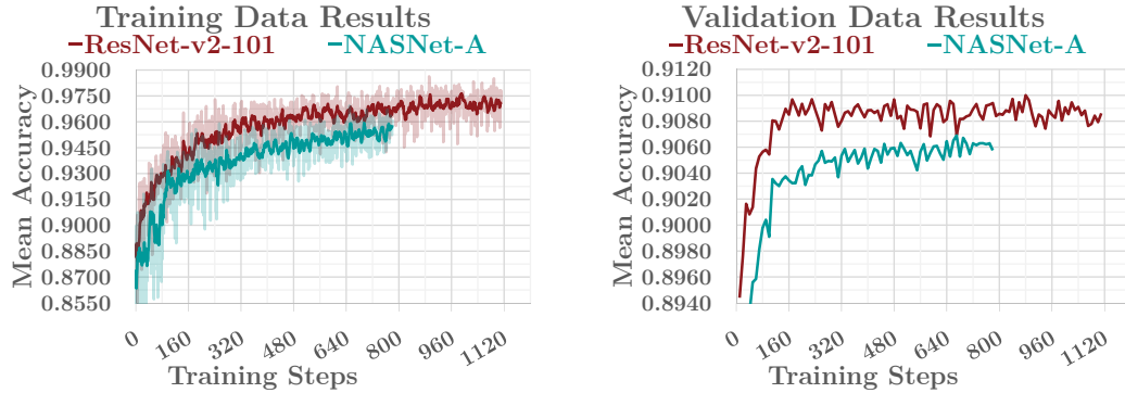
Figure 4.14: The results for ResNet-v2-101 and NASNet-A networks.
