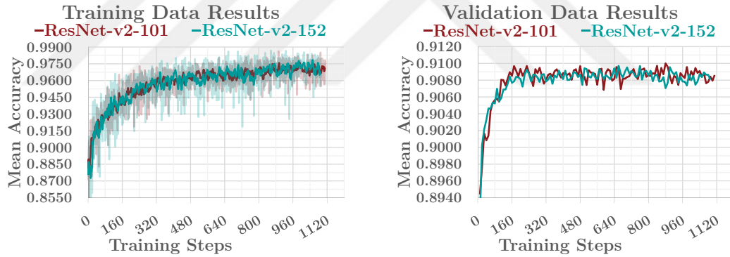
Figure 4.11: Comparison of ResNet-v2-101 and ResNet-v2-152 networks.
