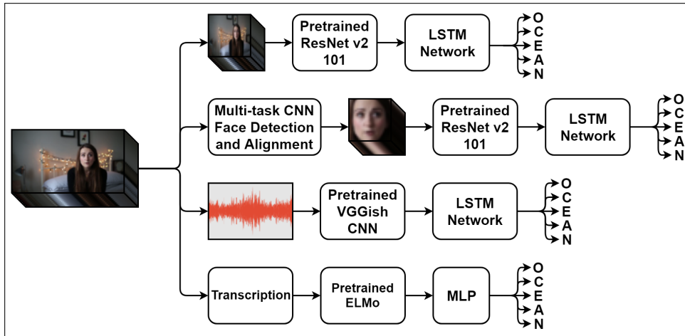
Figure 3.1: The first stage of the proposed model. Subnetworks learn to recognize personality traits based on the corresponding input features.
