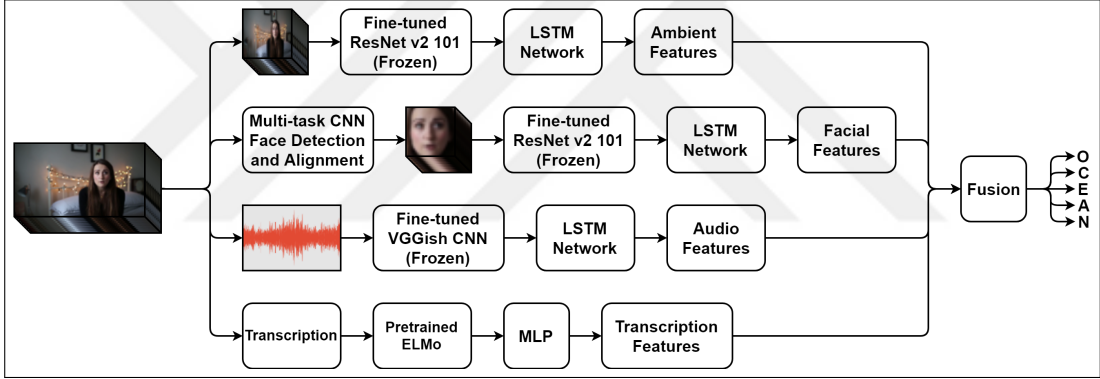
Figure 3.2: The second stage of the proposed model. We use trained subnetworks as feature extractors and fuse the results of them to obtain the final score for traits.
