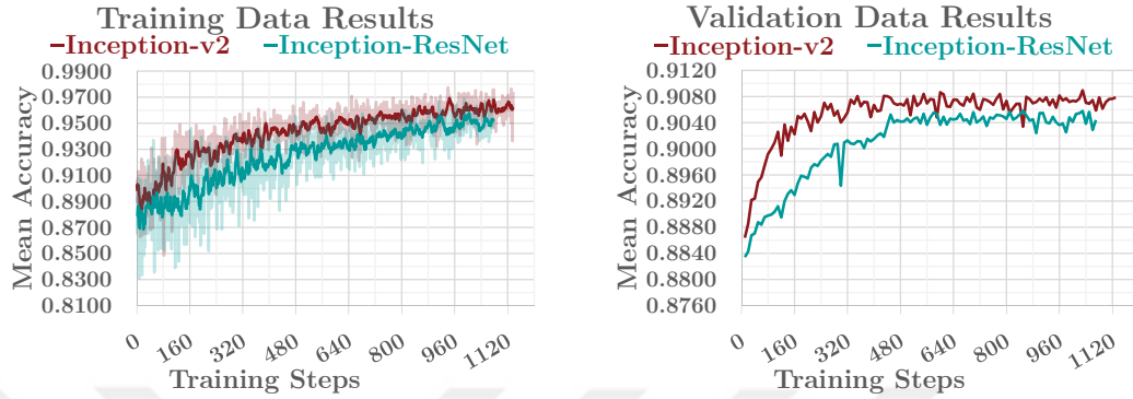
Figure 4.8: The results for Inception-v2 vs. Inception-ResNet-v2 networks.
