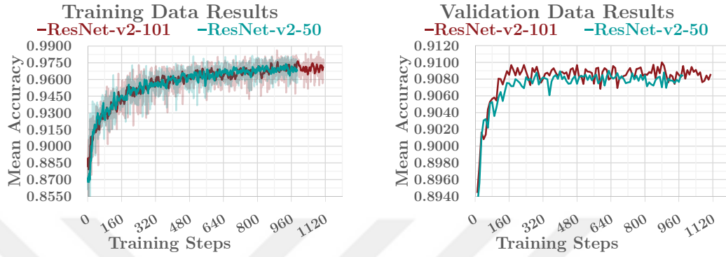
Figure 4.10: Comparison of ResNet-v2-101 and ResNet-v2-50 networks.
