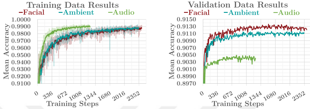
Figure 4.19: The comparison of audio feature-based, facial feature-based, and ambient feature-based subnetworks.
