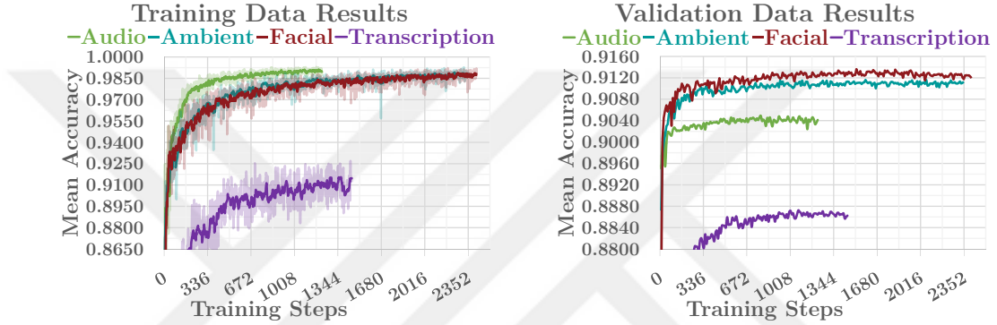
Figure 4.21: The comparison of facial feature-based, ambient feature-based, audio feature-based, and transcription feature-based subnetworks.
