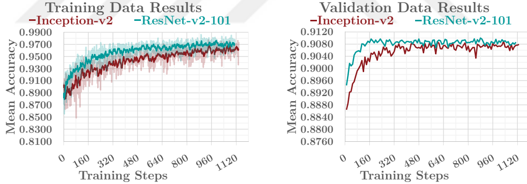
Figure 4.9: The results for Inception-v2 and ResNet-v2-101 network architectures.
