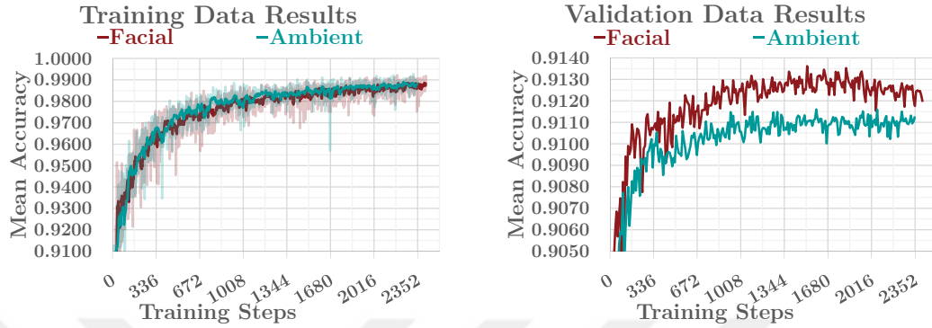
Figure 4.17: Comparison of facial feature-based subnetwork and ambient feature-based subnetwork.
