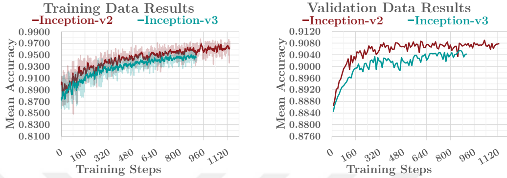
Figure 4.6: The results for Inception-v2 vs. Inception-v3 networks.
