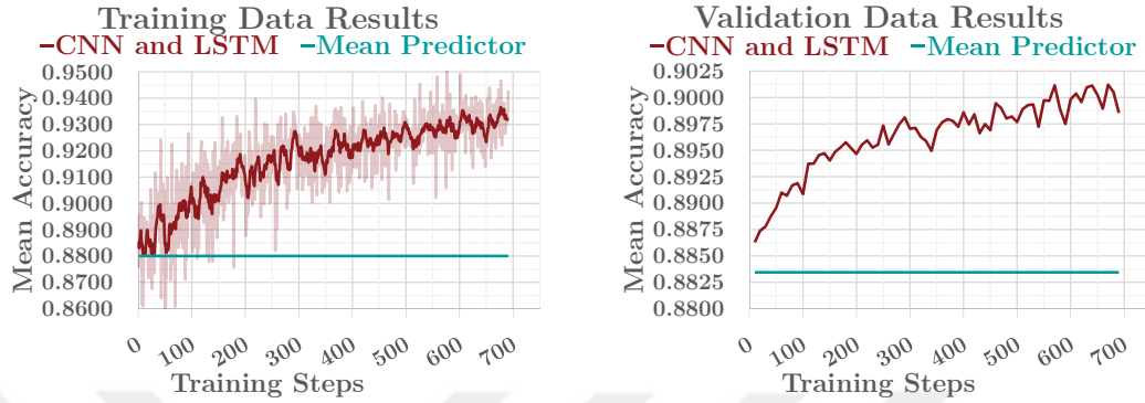
Figure 4.3: The results of simple CNN and LSTM network.
