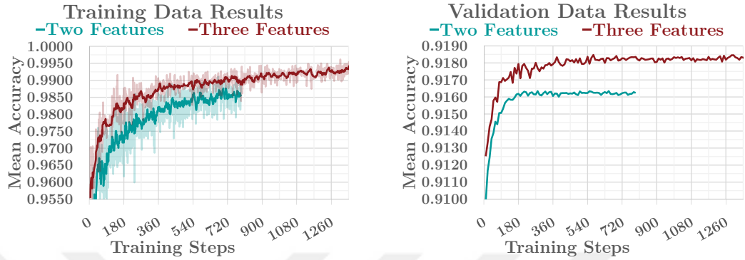
Figure 4.23: The comparison of the two and three feature-based networks. The two feature-based network uses ambient and audio features and the three-feature-based network uses ambient, audio, and facial features.
