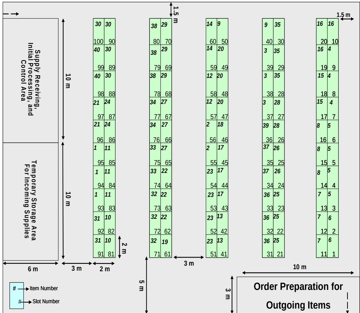
Figure A11. Single-Level Storage System: Configuration #6
