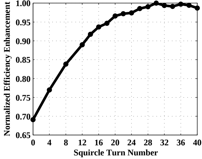
Figure 3.4: Normalized power transfer efficiency enhancement as a function of the outer squirle turn number of the proposed coil architecture calculated for the aluminum plate (for the total turn number kept fixed at 44).
