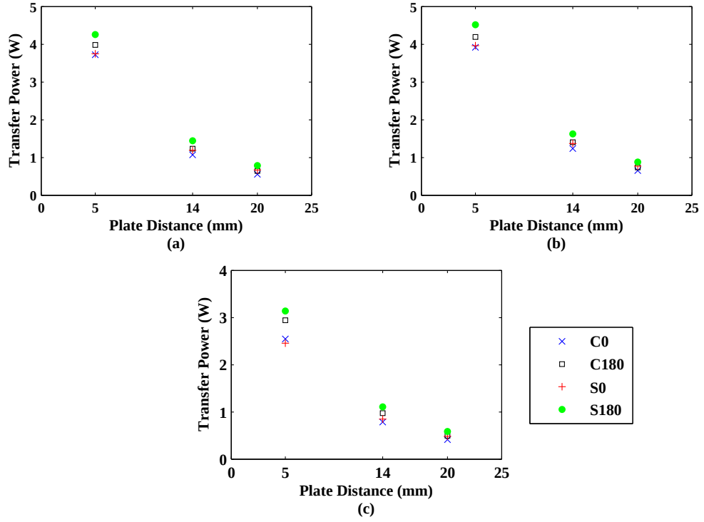
Figure A.8: Power transfer as a function of plate distance for systems in which pair of circular and squirrel coils are driven with the 0^\circ and 180^\circ phase differences and aluminum plate with diameter of (a) 180 mm, (b) 120 mm, and (c) 75 mm is located. Here, the distance between the plate's center and the side-by-side placed coils' midpoint is 12.5 mm on a constant horizontal plane. In the figure, labels S0 and S180 correspond to the systems in which squirrel coils are driven with the 0^\circ and 180^\circ phase differences, respectively. Similarly, C0 and C180 represent the systems where circular coils are driven with the 0^\circ and 180^\circ phase differences.
