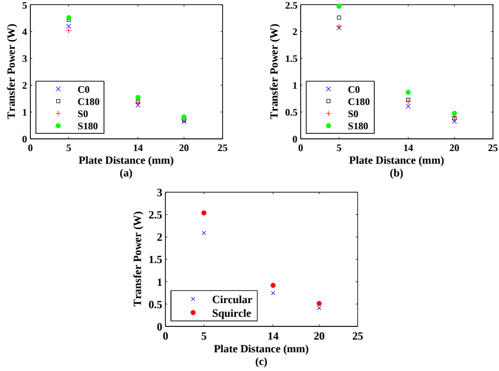
Figure A.12: Power transfer as a function of plate distance for systems in which pair of circular and squircle coils are driven with the 0^\circ and 180^\circ phase differences and aluminum plate with diameter of (a) 180 mm, (b) 120 mm, and (c) 75 mm is located. Here, the distance between the plate's center and the side-by-side placed coils' midpoint is 37.5 mm on a constant horizontal plane. In subfigures (a) and (b), labels S0 and S180 correspond to the systems in which squircle coils are driven with the 0^\circ and 180^\circ phase differences, respectively. Similarly, C0 and C180 represent the systems where circular coils are driven with the 0^\circ and 180^\circ phase differences. In subfigure (c), on the other hand, labels circular and squircle represent the systems in which single circular and single squircle coil is driven.
