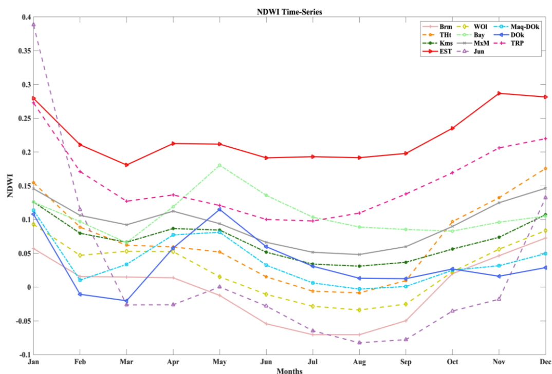
Figure 5.21. NDWI time-series.
