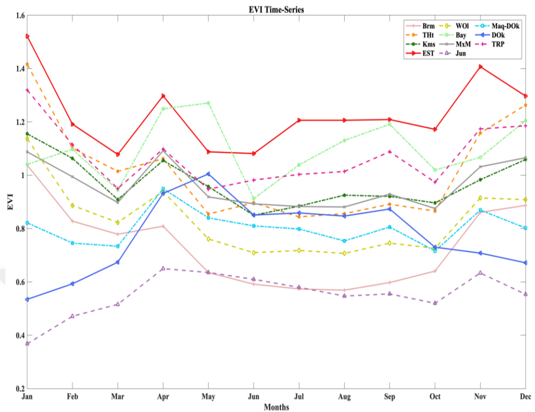
Figure 5.27. EVI time-series.
