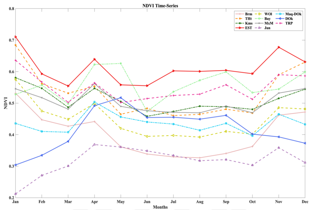
Figure 5.17. NDVI time-series.
