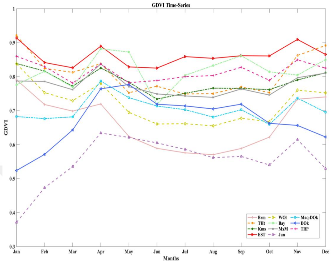
Figure 5.29. GDVI time-series.
