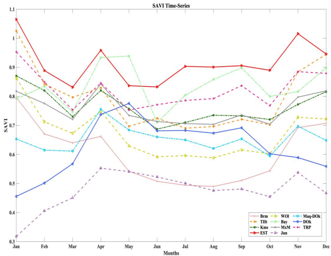
Figure 5.26. SAVI time-series.
