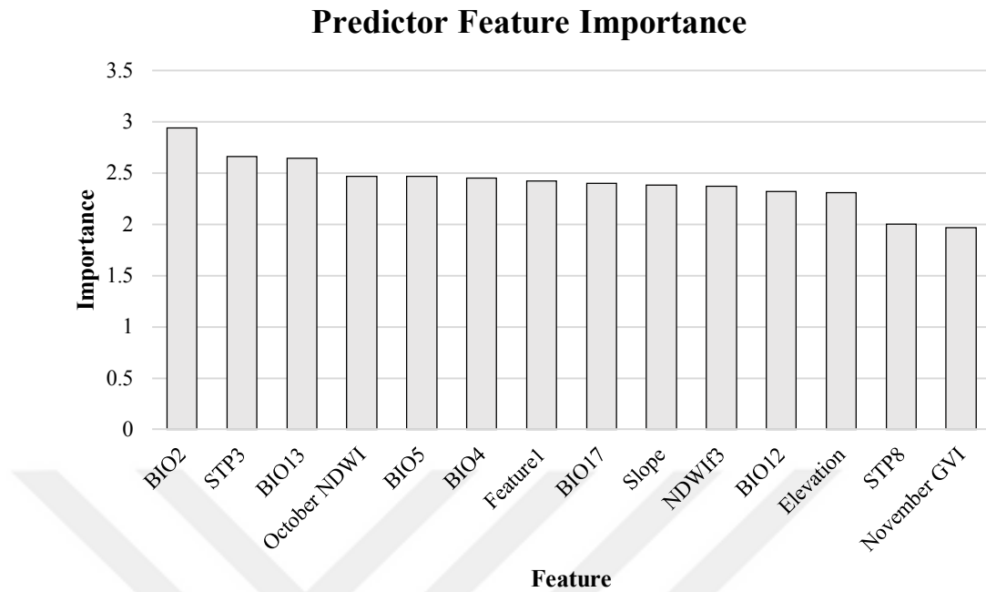
Figure 5.37. Predictor feature importance chart.
