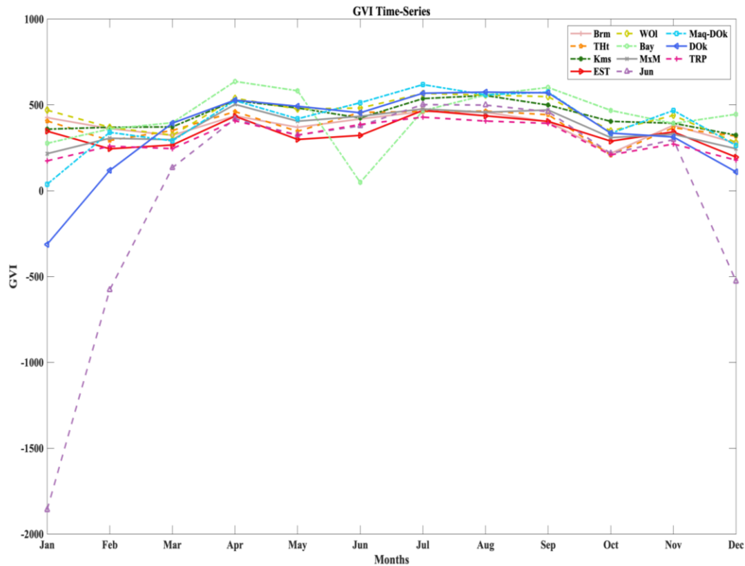
Figure 5.28. GVI time-series.
