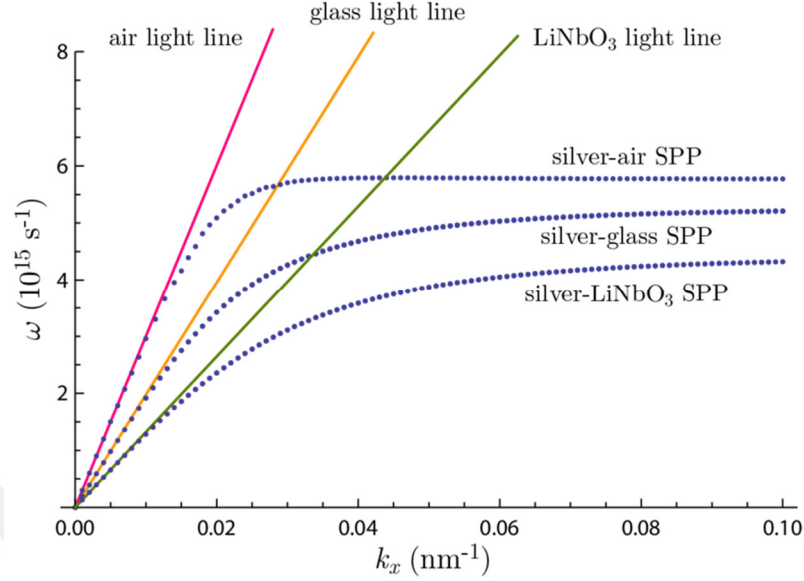
Figure 1.6. Dispersion diagram relations for air, dielectric medium (silver and LiNbO 3 ) and SPs at the interface between two different mediums. It is important to note that the SP for the case of silver-LiNbO 3 does not cross with that of light. As a result, SPs cannot be excited by light propagations.
