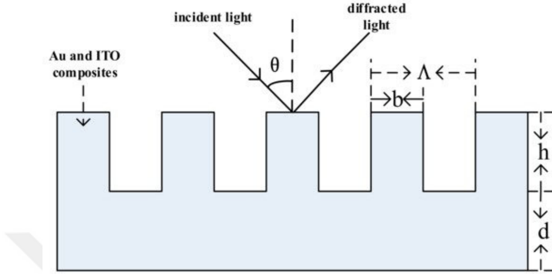
Figure 1.8. Phase matching of the incident light with the wavevector using a metallic grating surface. Figure adapted from Li.W et al [34].
