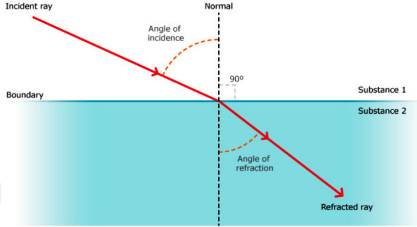
Figure 1.5. Schematic diagram illustrating the refraction of light at the interface between two different media with refractive indexes of n_1 and n_2 at the incident angle \theta .
