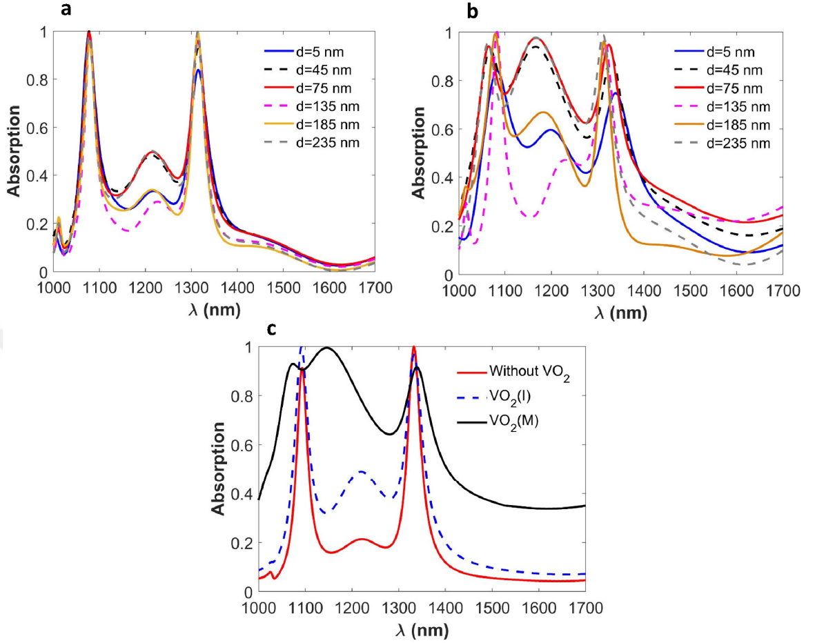
Figure 3.3. The calculated absorption spectra of the proposed absorber based on distances of \text{VO}_2 film mid plane from the bottom metallic layer (a) in the insulator phase (b) in the metallic phase (c) and the obtained optimized distances of \text{VO}_2 layer in the insulator and metallic phases compared with absorption spectra without \text{VO}_2 layer.
