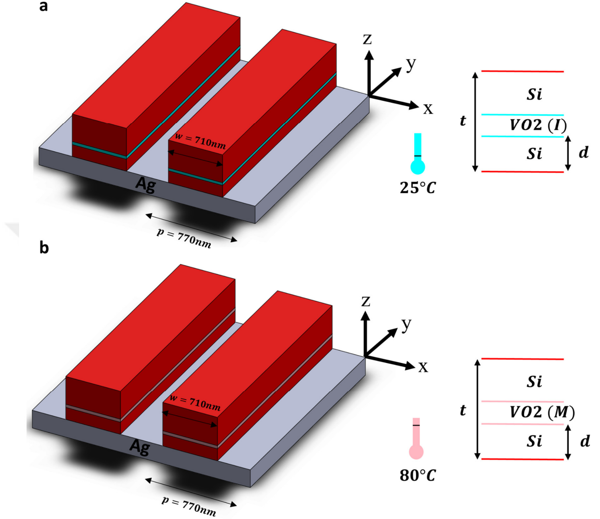
Figure 3.2. Geometry and schematic of the VO 2 -based metamaterial absorber. The absorber consists of VO 2 in (a) the insulating phase and (b) the metallic phase sandwiched between layers of a-Si and continuous film of Ag as the bottom layer of the structure.
