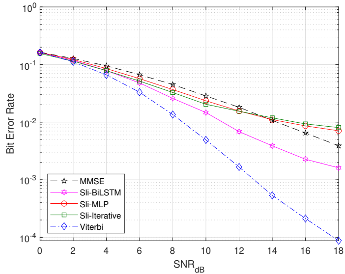
Figure 4.4: BER results of the Sli-BiLSTM, Sli-MLP, and Sli-Iterative detectors for MIMO ISI, varying channels, L = 3 and n_R=n_T=2 .
