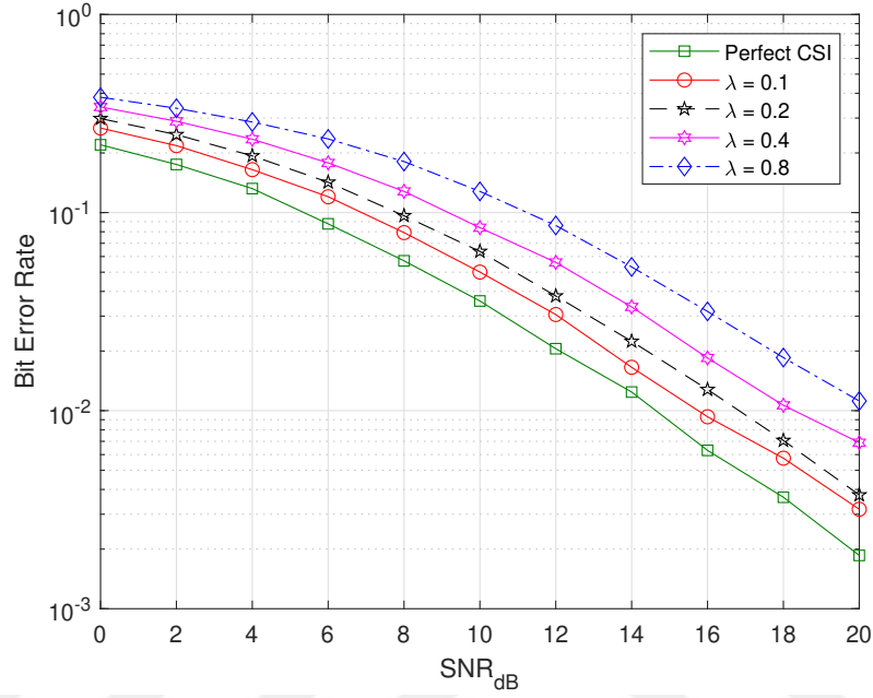
Figure 3.13: BER results of the Sli-BiLSTM model for the varying channels L = 3 , N = 10 , and different channel state information error levels.
