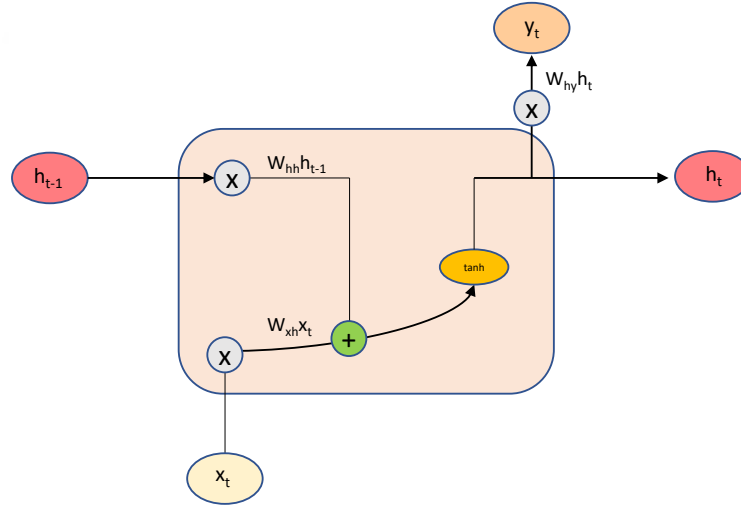
Figure 2.6: Structure of an RNN cell.
