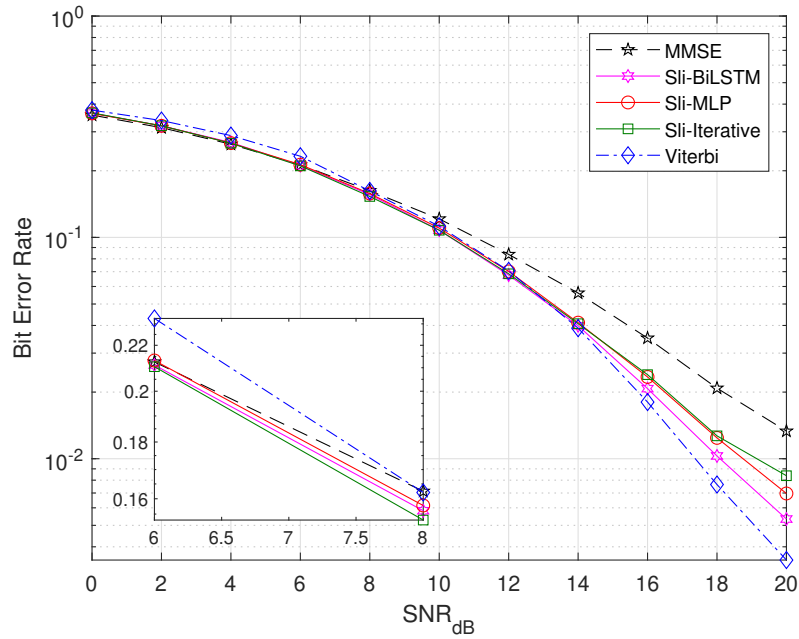
Figure 3.14: BER results of the Sli-BiLSTM, Sli-MLP, and Sli-Iterative model for the varying channels, L = 5 , N = 10 , and \lambda = 0.4 .
