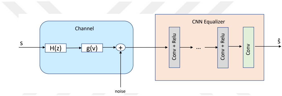
Figure 2.13: The system architecture of CNN equalizer.
