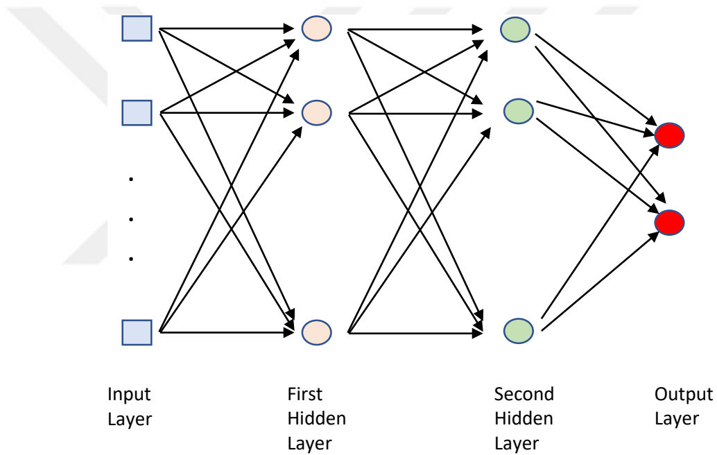
Figure 2.2: An example of an MLP network
