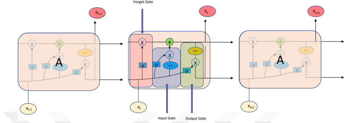
Figure 2.7: The repeating module in an LSTM.
