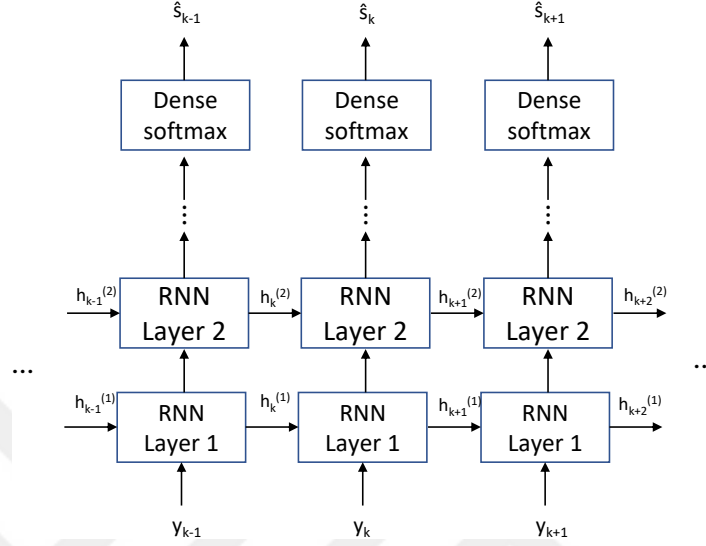
Figure 2.15: RNN architecture for detection.
