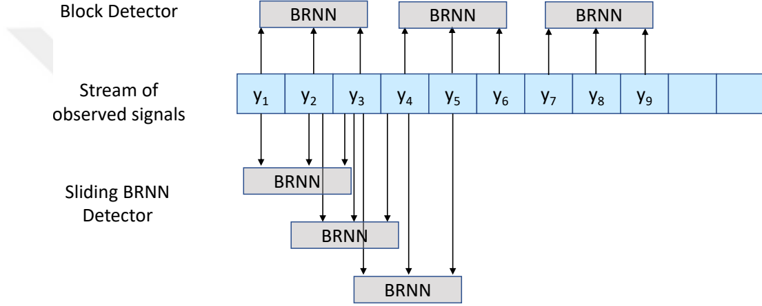
Figure 2.10: The sliding BRNN detector.
