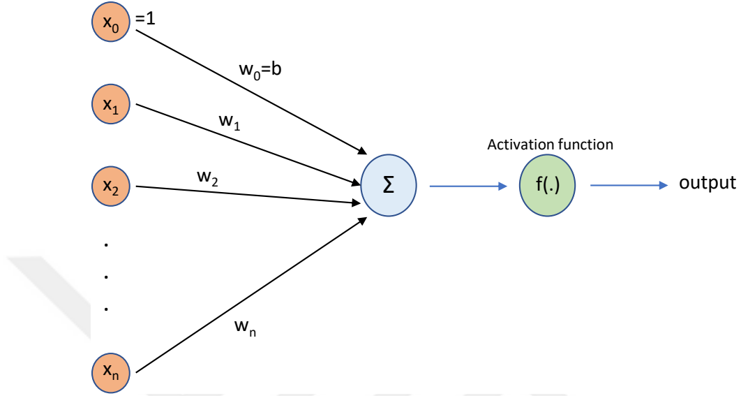
Figure 2.1: Perceptron.
