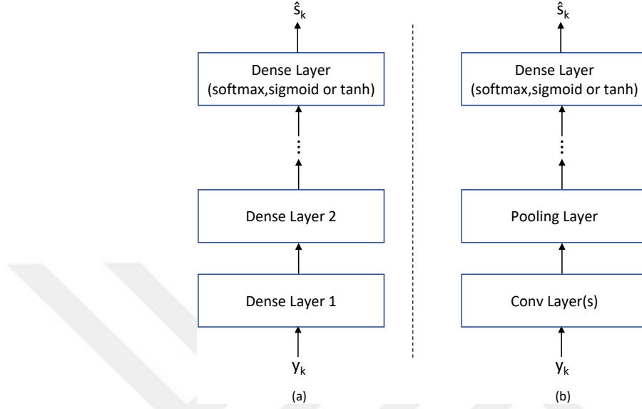
Figure 2.14: Symbol-by-Symbol Detector.
