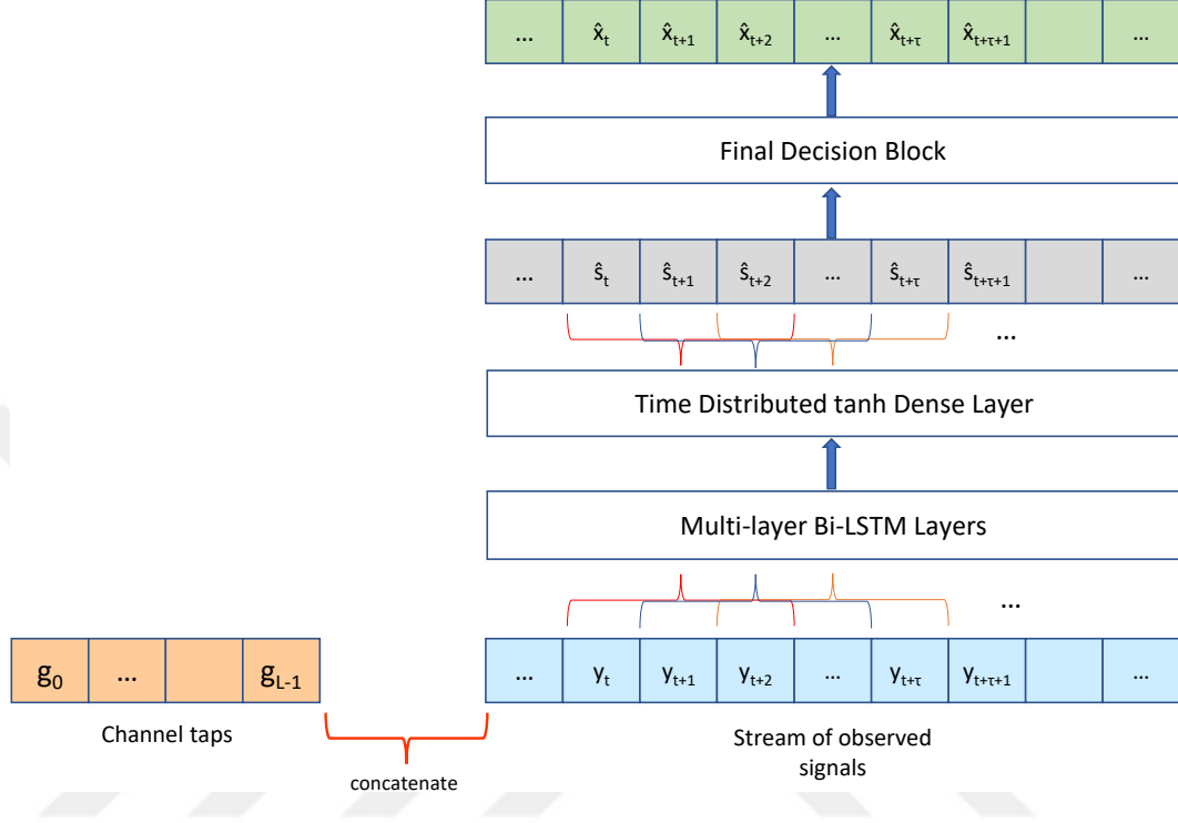
Figure 3.2: The network architecture of Sliding Bi-LSTM ISI detector.
