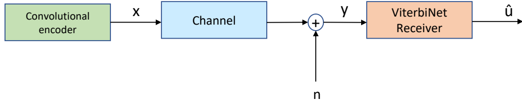
Figure 2.12: ViterbiNet receiver with joint symbol detection and channel decoding.
