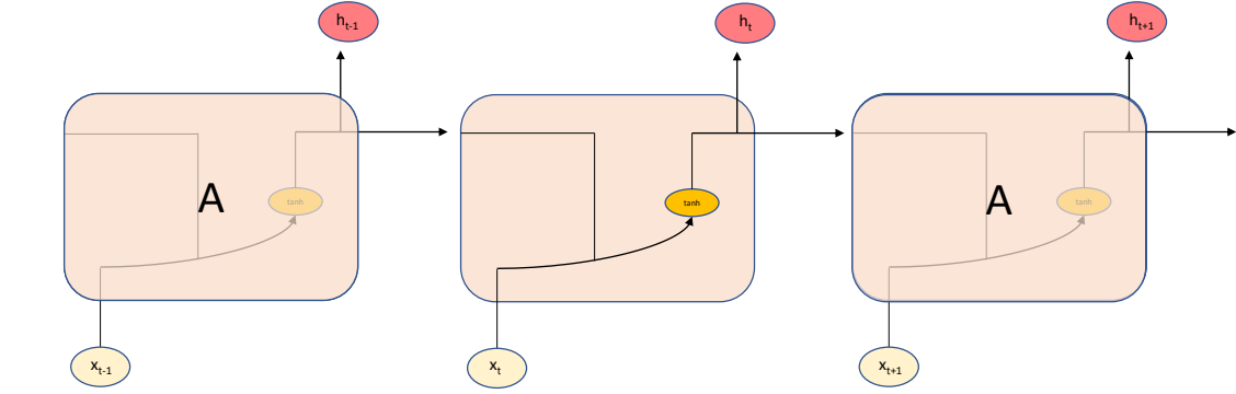
Figure 2.5: The repeating module in a standard RNN.
