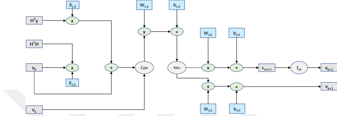
Figure 2.16: A flowchart representing a single layer of DetNet.
