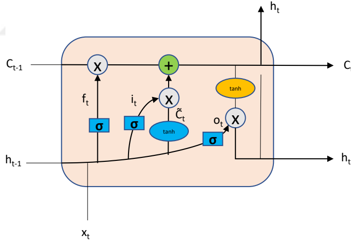
Figure 2.8: Structure of LSTM cell.
