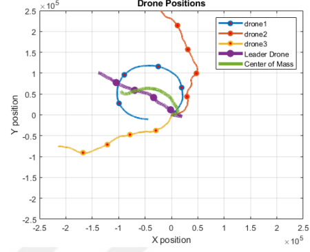
(b) 100 km communication range.
