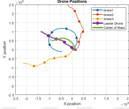
(a) 50 km communication range.
