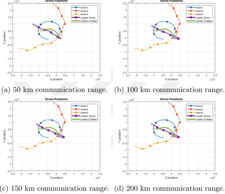
Figure 5.14: Optimal trajectory of path planner with no optimization horizon.
