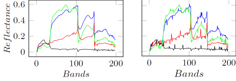
Figure 3.5: Four multispectral signatures that are corrupted with the concept of Denoising Autoencoder.
