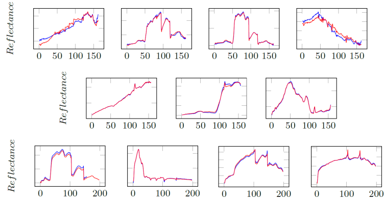
Figure 3.13: Ground truth (blue) and estimated (red) endmember signatures for Urban (first row), Samson (second row) and Jasper (third row) datasets.
