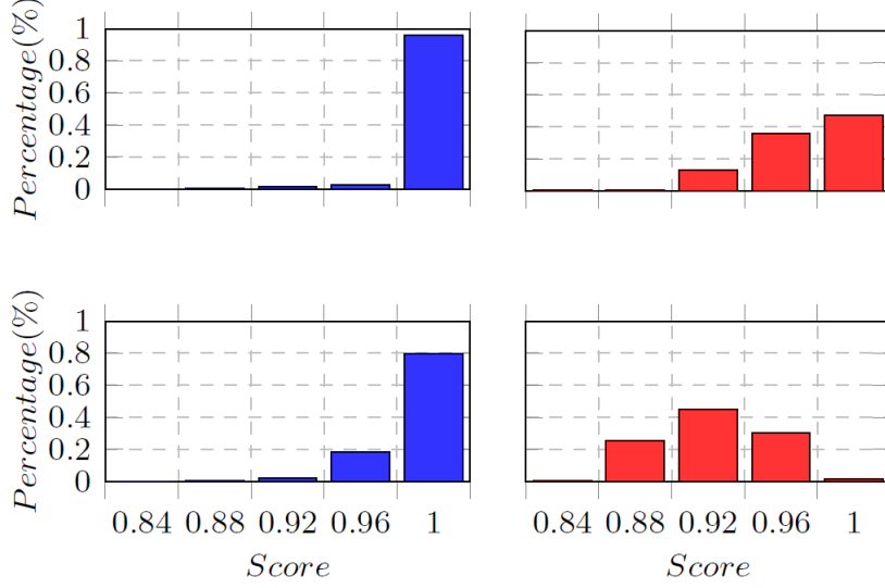
Figure 3.3: Normalized similarity score distributions for same (blue) and coherent (red) materials. Results for inner product (first row) and SAD (second row) are illustrated.
