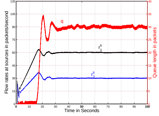
Figure 4.12: Results for Case 4
