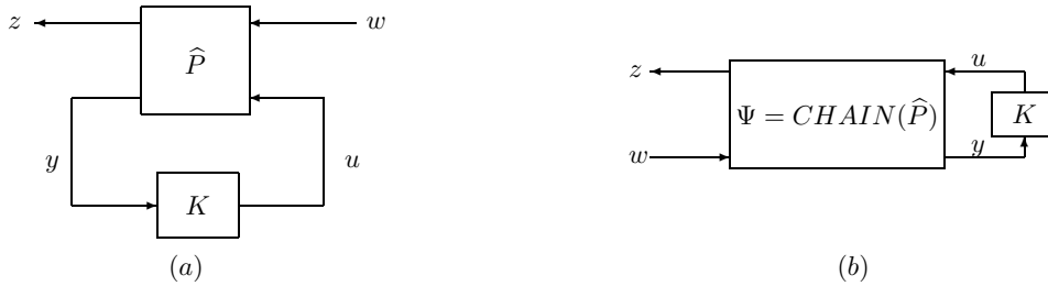
Figure 2.1: a) Generalized framework b) Its chain-scattering representation
