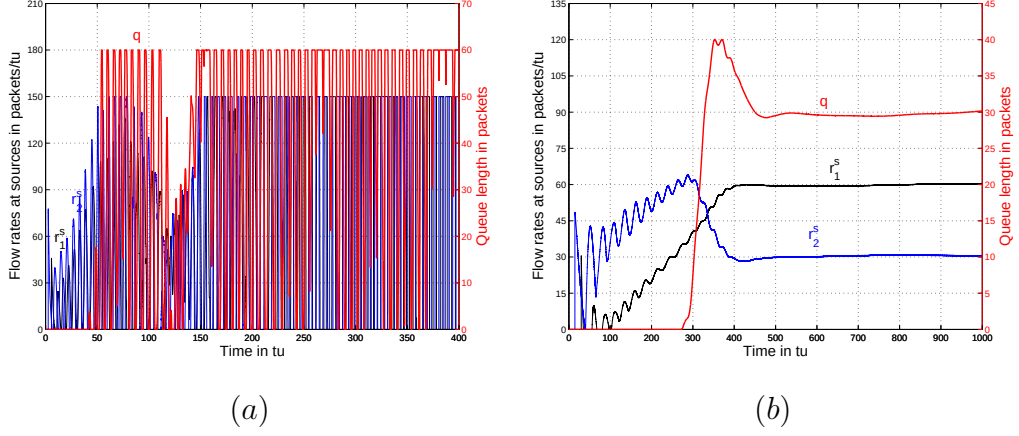
Figure 5.4: Simulation results for Case 2a
