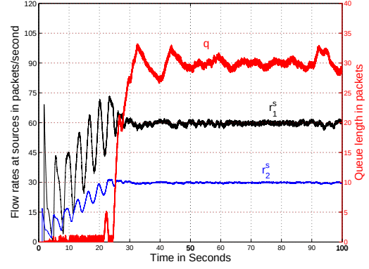
Figure 4.14: Results of [23] for Case 1
