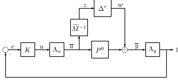
Figure 3.9: Feedback configuration with right co-prime factorization [39]
