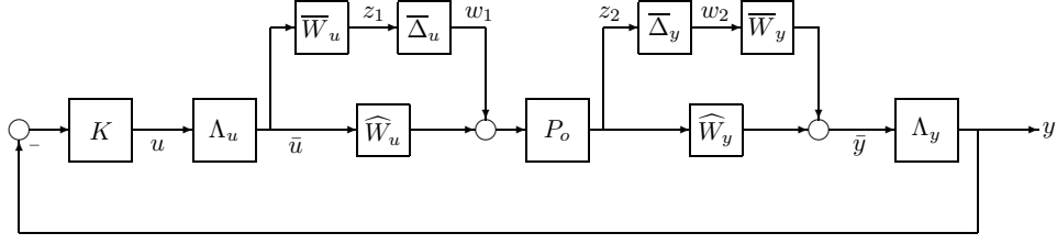
Figure 3.10: Feedback configuration for the actual plant \Omega
