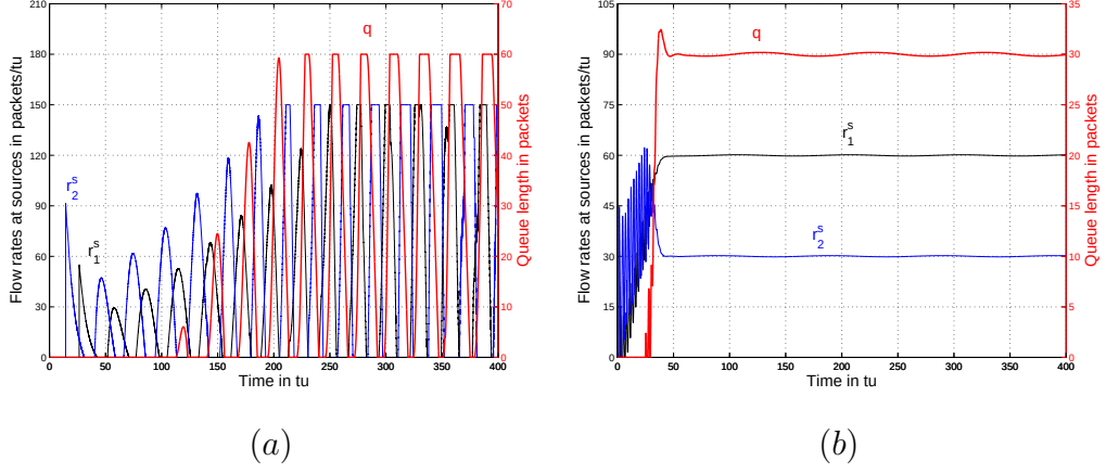
Figure 5.2: Simulation results for Case 1a
