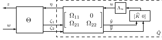
Figure 4.6: New problem definition under chain-scattering representation [42]
