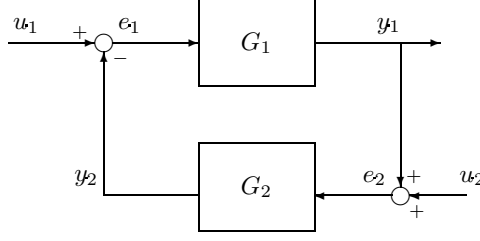
Figure 3.2: Feedback system [36]
