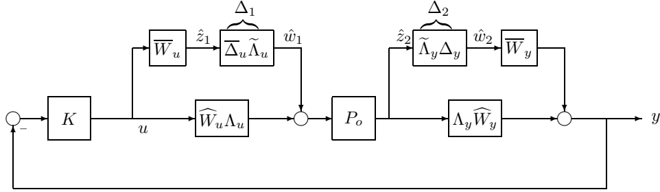
Figure 3.11: Equivalent system
