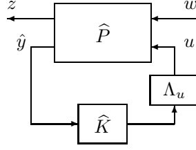
Figure 4.5: General four-block problem [42]
