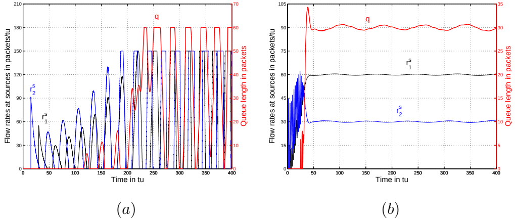
Figure 5.3: Simulation results for Case 1b
