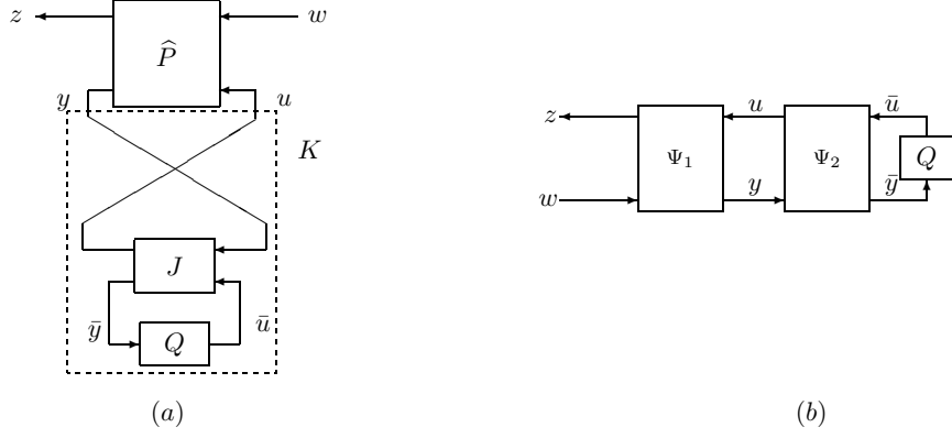
Figure 2.2: a) Star product of systems, b) Cascade connection in chain-scattering representation
