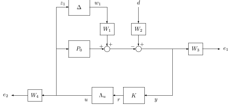
Figure 4.3: System for the mixed sensitivity minimization problem [25]
