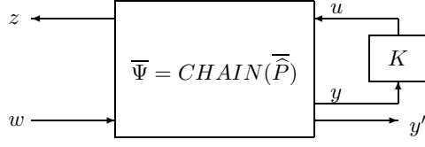
Figure 2.3: Chain scattering representation of output augmented system
