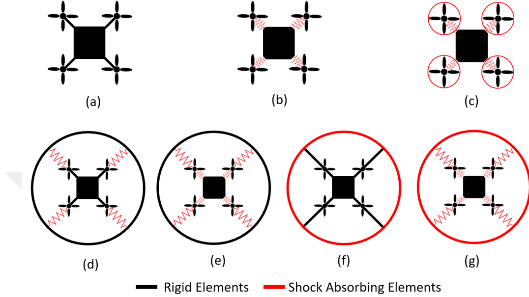
Figure 1.3: Collision protection strategies. ( Inspired from [1] )
