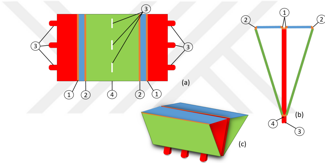
Figure 3.4: Folding of the arms. (a) Unfolded paper sheet, orange seam lines are perforated with laser for accurate folding. Folding hierarchy is noted with numbers. (b) Cutaway of the folded load bearing arms, triangular cells can be seen. (c) Overall shape of the folded arms.
