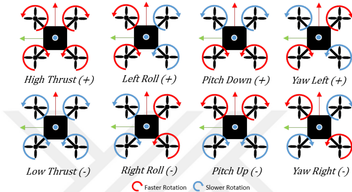
Figure 2.1: Roll, pitch, yaw operator inputs translated into rotor inputs for X-Quad configuration.
