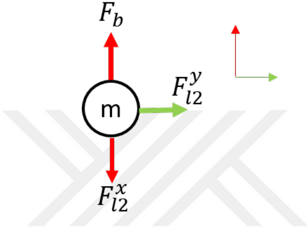
Figure 3.19: Free body diagram of the forces acting on the mass hinge point.
