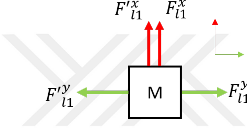
Figure 3.17: Free body diagram of the forces acting on the mass hinge point.
