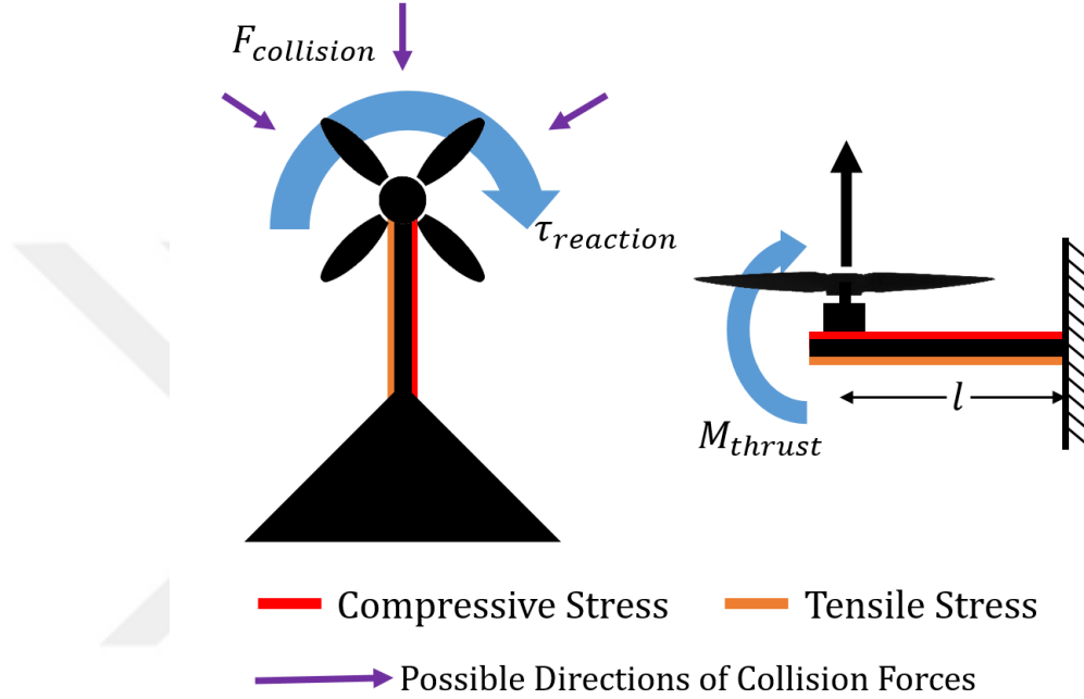
Figure 3.2: Forces acting on the arms.
