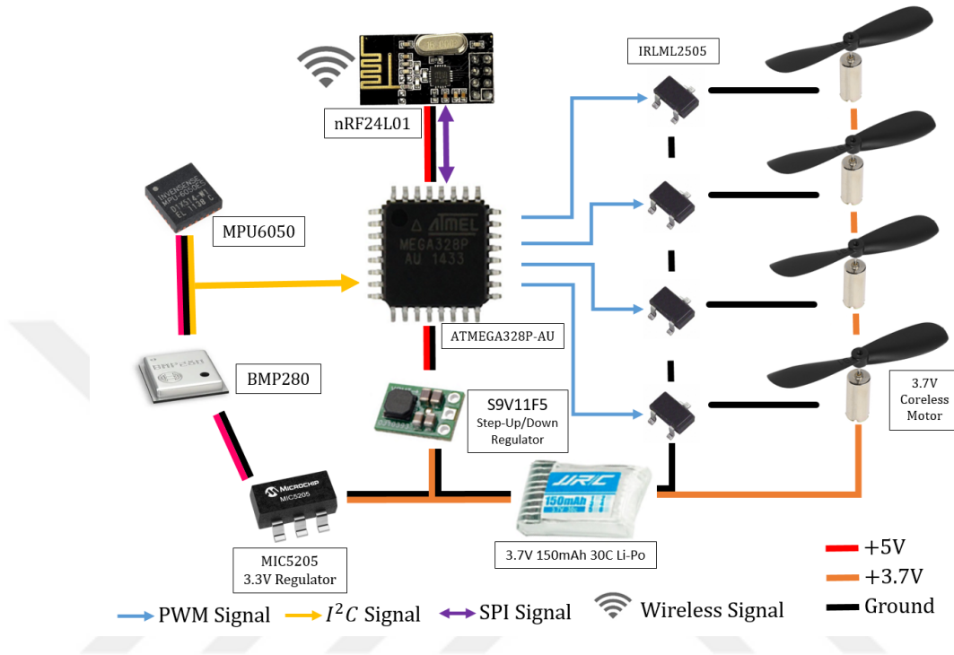
Figure 3.10: Active electronic elements and circuitry including power and signal layout. Passive components are not included.
