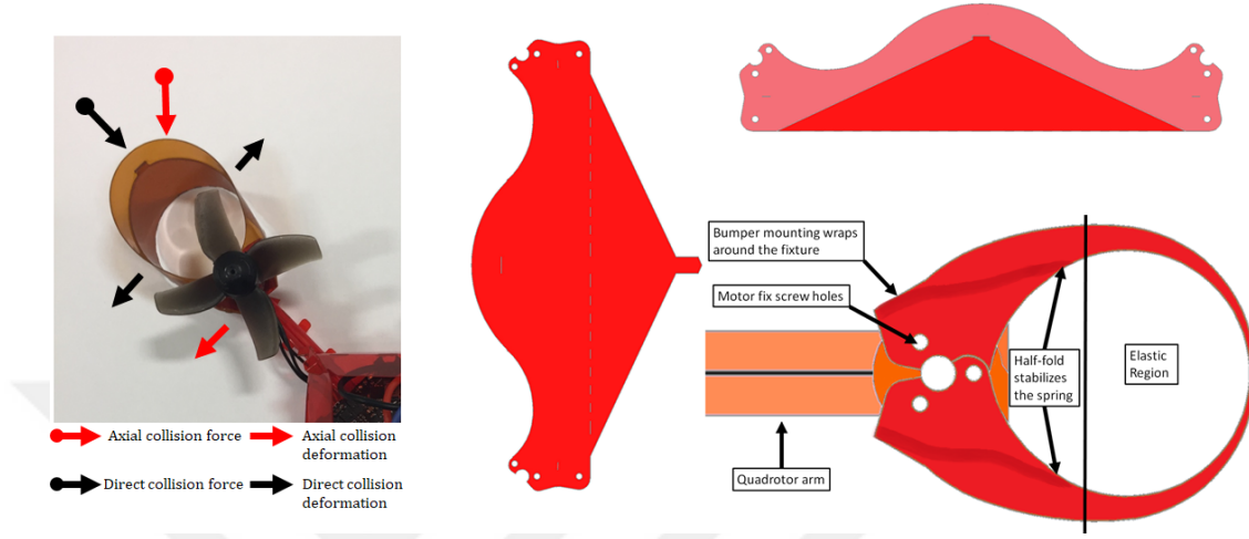
Figure 3.8: Collision scenarios and related force reactions(left), Unfolded bumper part (middle), folded and fixed bumper part (right top), bumper and rotor fixture assembly seen from top (right bottom)
