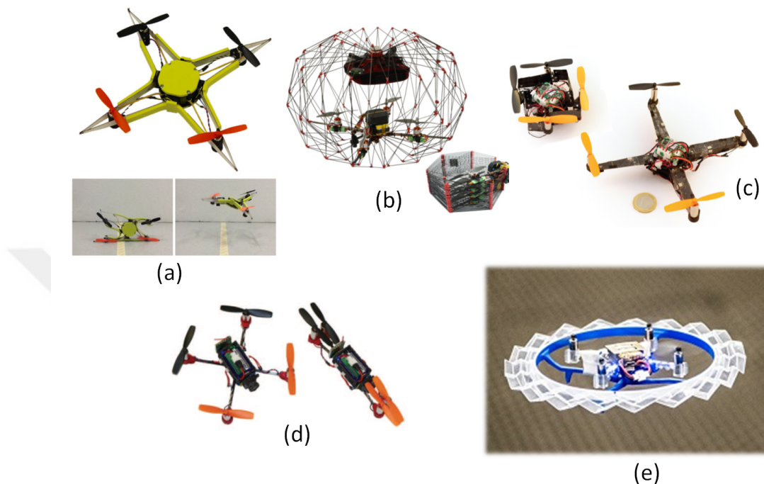
Figure 1.4: (a) Collision resilient drone [1], (b) Origami inspired protective cage equipped drone [2], (c) Pocket-size self deployable drone [3], (d) Pocket-size collapsible drone [4], (e) Rotorigami: origami cushion for collision protection.
