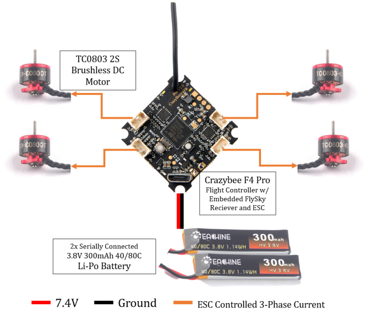
Figure 3.15: Setup of the finalized electronic suite equipped with Crazybee F4 Pro.
