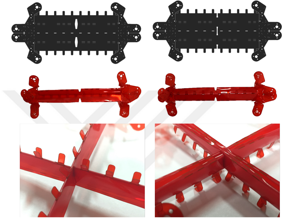
Figure 3.5: Two diagonal arms joined together with half-lap joint.
