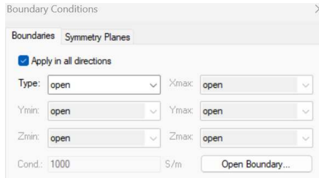
Figure 3.23. Used boundary conditions for frequency domain solver
