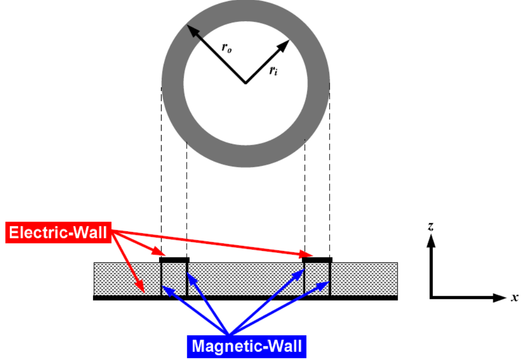
Figure 34: Magnetic-wall model of the ring resonator
