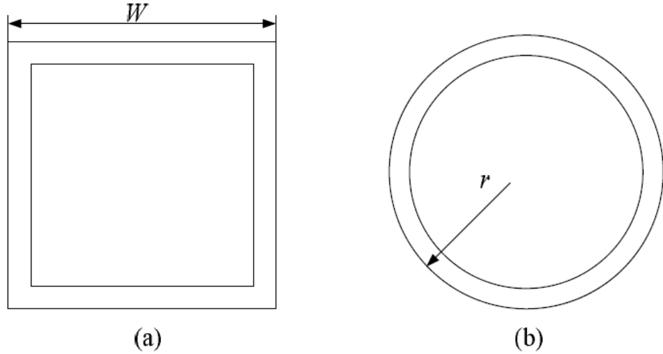
Figure 33: Unsplit-loop microstrip ring resonator (a) Square ring, (b) Annular ring
