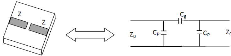
Figure 12: Gap discontinuity
