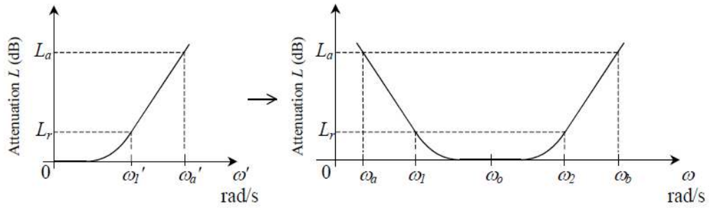
Figure 28: Corresponding bandpass filter response regarding the Butterworth lowpass filter response
