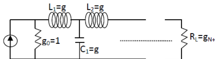
Figure 24: Lowpass filter prototype
