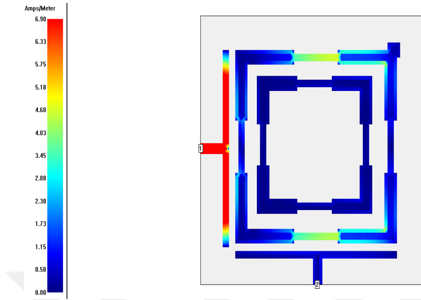
Figure 46: Simulated current density distributions of the proposed BPF at 3.3 GHz (in stopband region)
