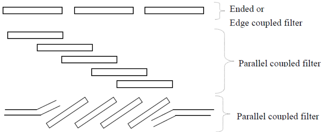
Figure 30: Couple resonator bandpass filters
