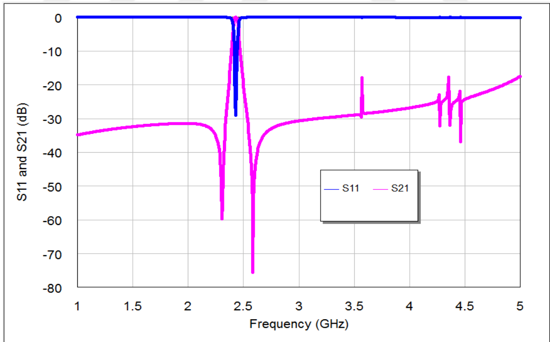
Figure 42: The out-of-band transmission responses of the proposed filter designed for 2.43 GHz fundamental frequency
