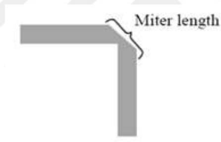
Figure 15: Mitering the bend
