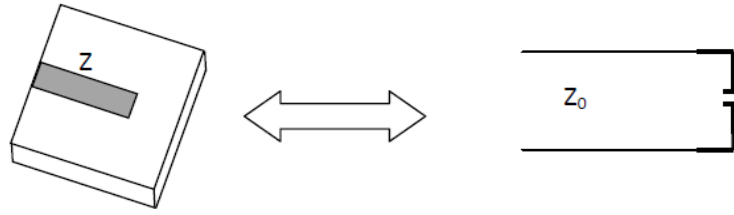
Figure 11: Open-ended discontinuity
