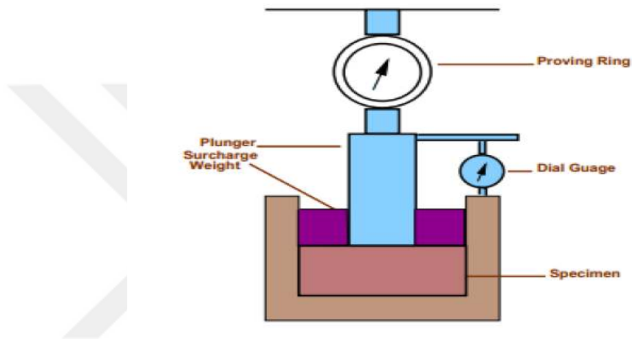
Figure 3.4 California bearing ratio testing machine
