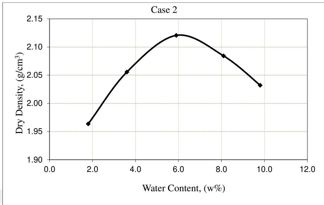
Figure 4.5 Modified Proctor Test result for case 2
