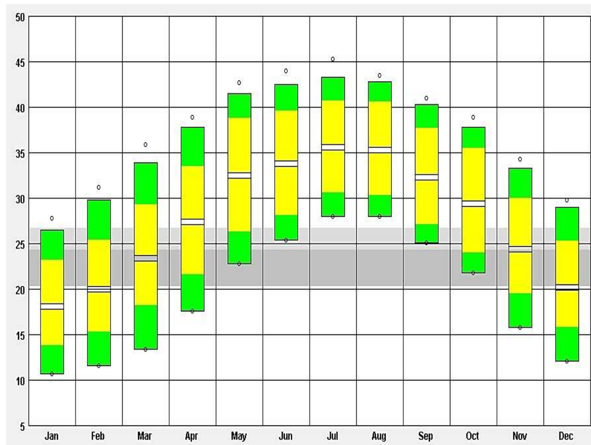
Figure 4.3: Temperature Range Diagram (Source: Climate Consultant)
