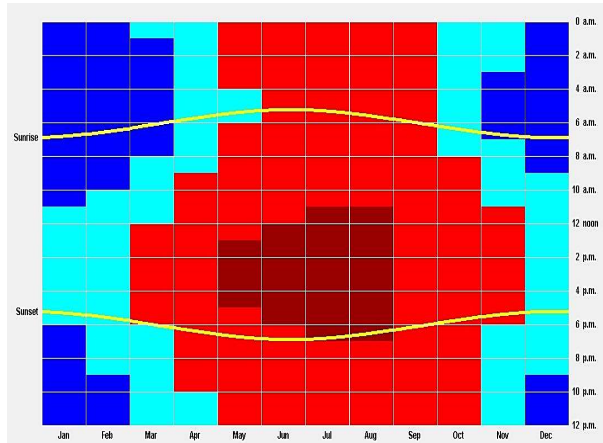
Figure 4.5: Kish Climate Calendar (Source: Climate Consultant Software)
