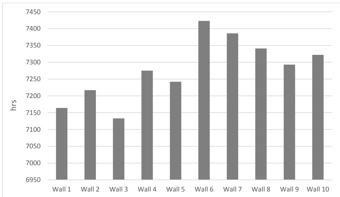
Figure 4. 30: Annual Comfort Hours for Walls 1-10 ( -0.5 < \text{PMV} < 0.5 )
