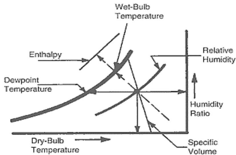
Figure 3.2: Psychometric Chart Main Indicators [202]
