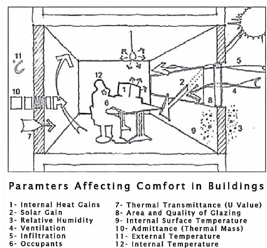
Figure 2.1: Parameters Affecting Thermal Comfort in Buildings [89]
