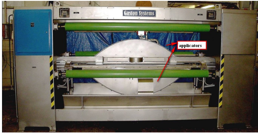
Figure 3.6 CFS parabolic applicator [51]
