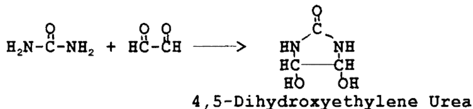
Figure 2.8 Synthesis of 4,5 - dihydroxyethylene urea [14]
