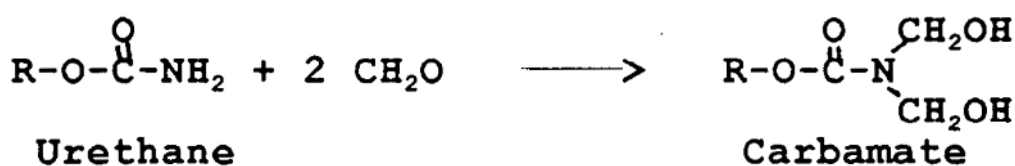
Figure 2.9 Synthesis of carbamates [15]
