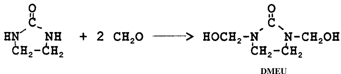
Figure 2.7 Methylation reaction [15]
