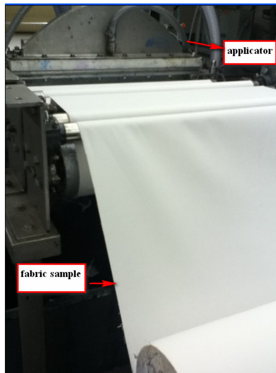
Figure 3.5 Laboratory type foam applicator
