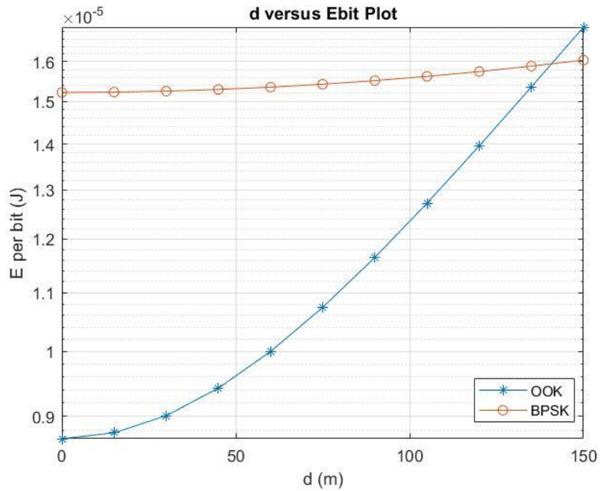
Figure 3.1. Energy per bit for various RF front-end architecture with Class A PA in narrow-bandwidth applications, BW= 10 kHz and d = (0\ 150] m.
