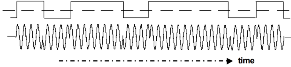
Figure 2.12. BPSK signal in the time domain [34].
