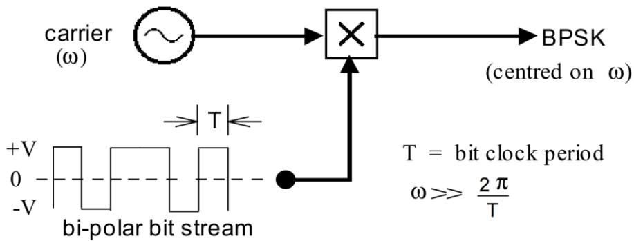
Figure 2.11. Generation of BPSK [34].
