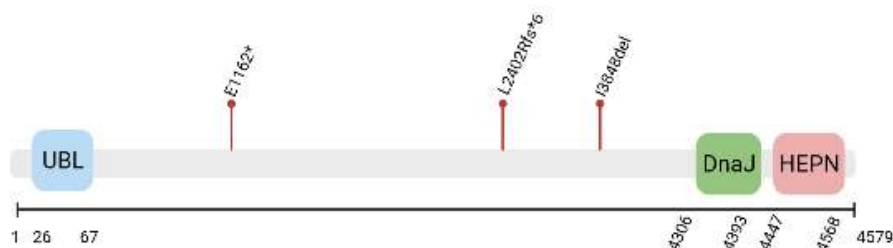
Figure 6.1 Mutations in the sacs1 protein are shown in red. UBL: Ubiquitin like domain, HEPN: Higher eukaryotes and prokaryotes nucleotide-binding domain. Positions were taken from InterPro ( https://www.ebi.ac.uk/interpro/protein/UniProt/Q9NZJ4/ ).
