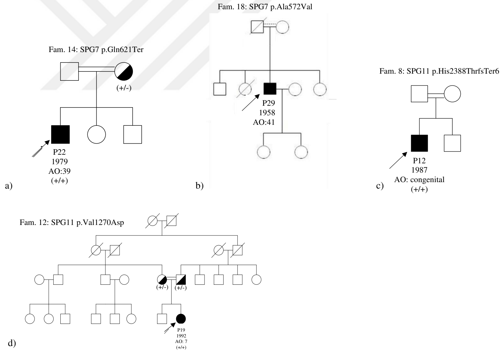
Figure 5.5 SPG7 and SPG11 families. a) SPG7-fam 14, b) SPG7- fam 18, c) SPG11-fam 8, d) SPG11-fam 12.
