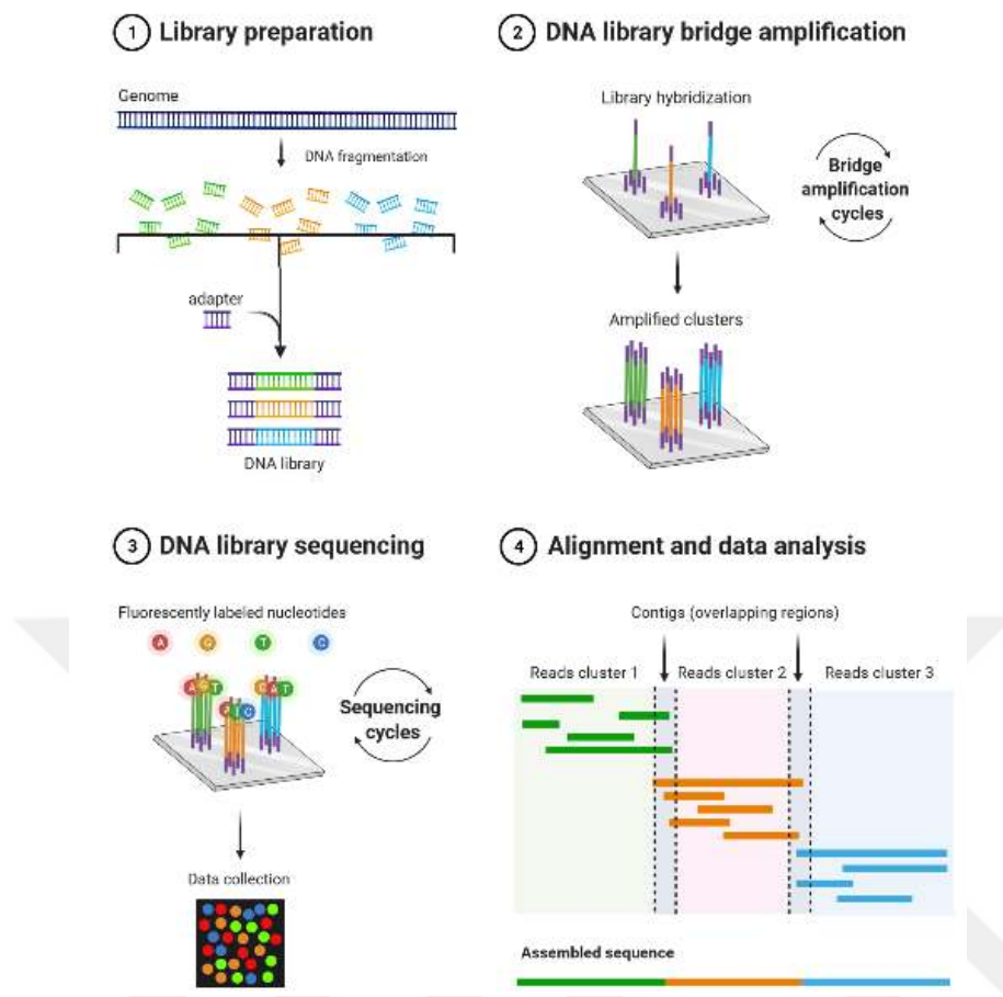
Figure 4.1 Steps of whole exome sequencing. Reprinted from “Next Generation Sequencing (Illumina)”, by BioRender.com (2021). Retrieved from https://app.biorender.com/biorender-templates .
