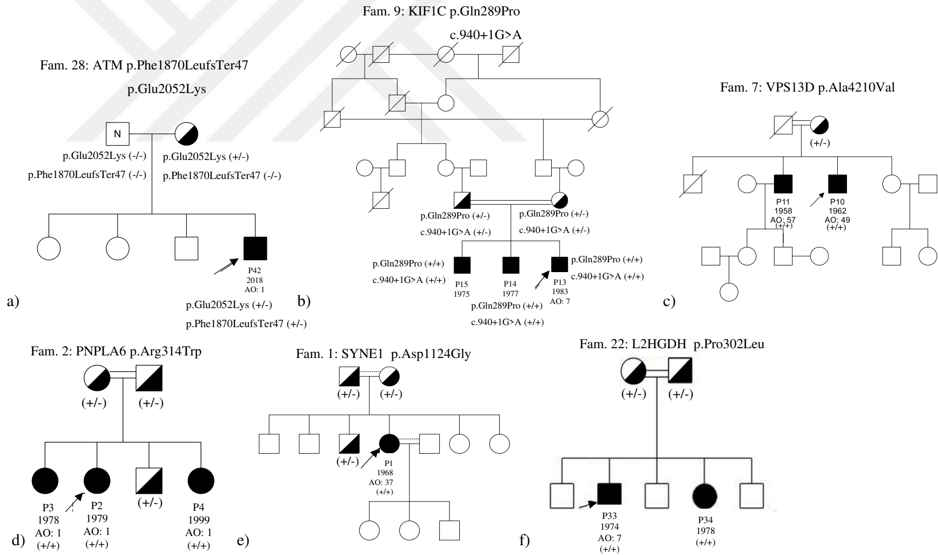
Figure 5.7 a) ATM-fam 28, b) KIF1C-fam 9, c) VPS13D-fam 7 d) PNPLA6-fam 2, e) SYNE1-fam 1, f) L2HGDH-fam 22.
