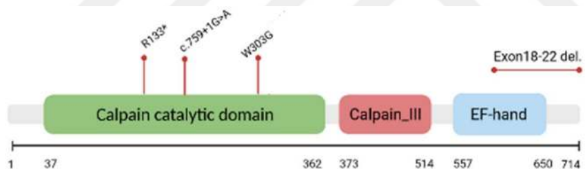
Figure 6.2 Mutations described in calpain-1 in the cohort shown in red. Domains were taken from InterPro ( https://www.ebi.ac.uk/interpro/protein/UniProt/P07384/ ).
