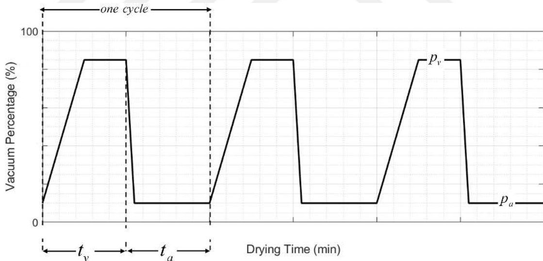
Figure 4.3: Explanation of vacuum modulation.
