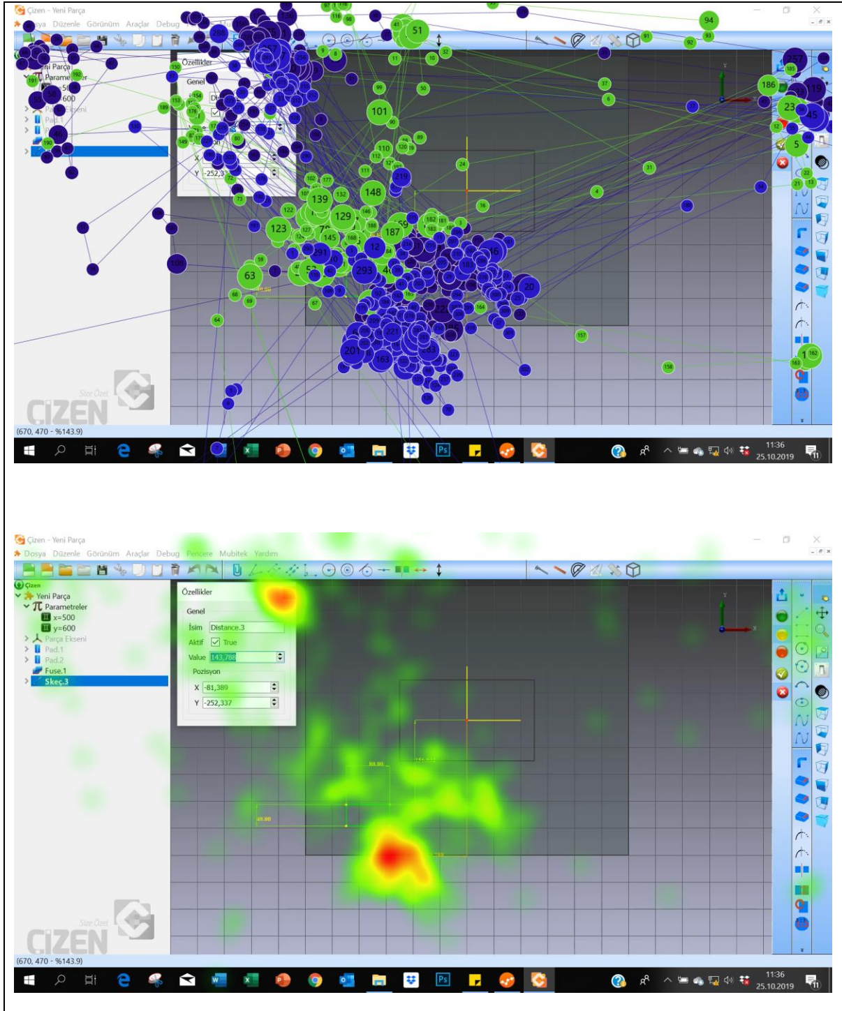
Figure 37. Task 5 Gazeplot and Heatmap (Right Menu Users)
