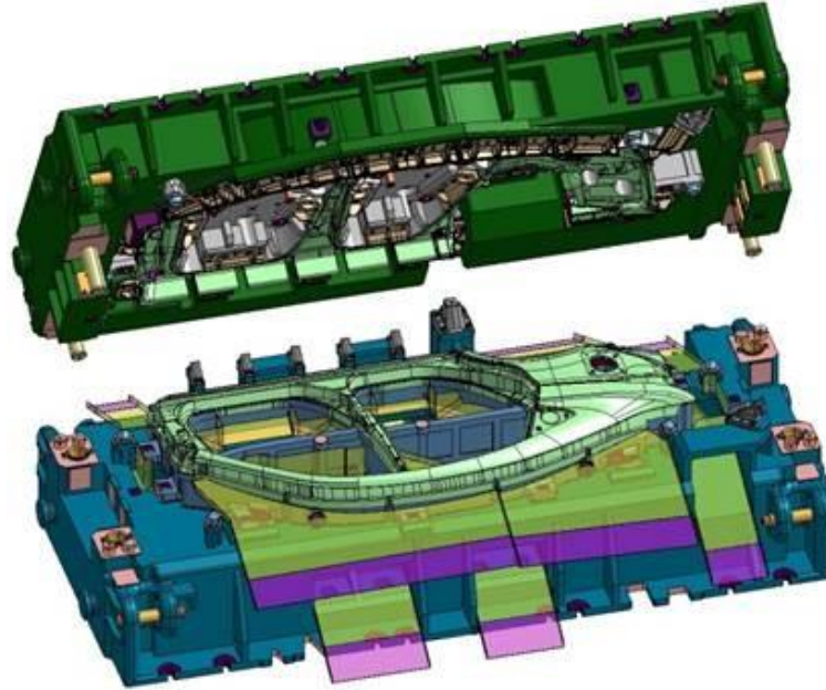
Figure 12. Bodyside Sheet Metal Forming Design
