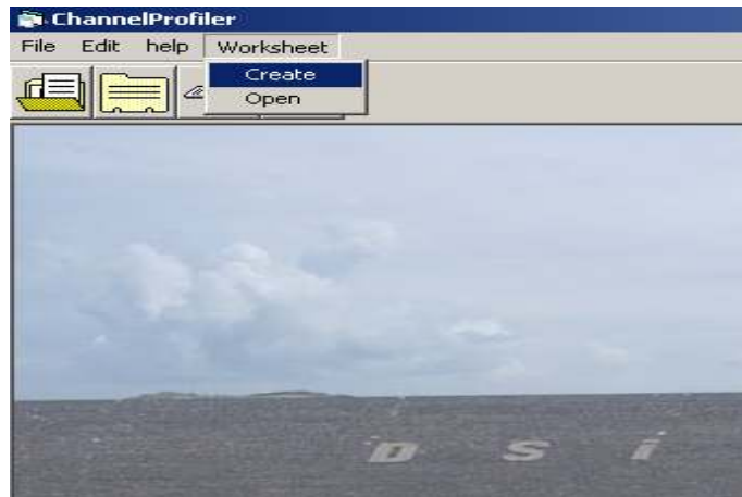
Figure 5.3 Worksheet Menu.
