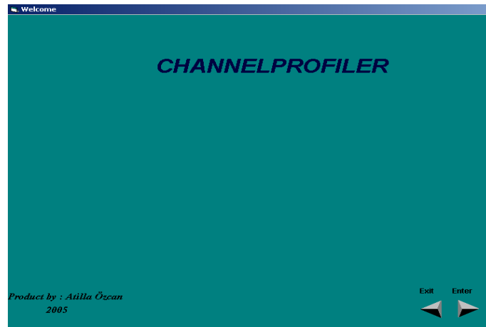
Figure 5.1 Beginning Form.
