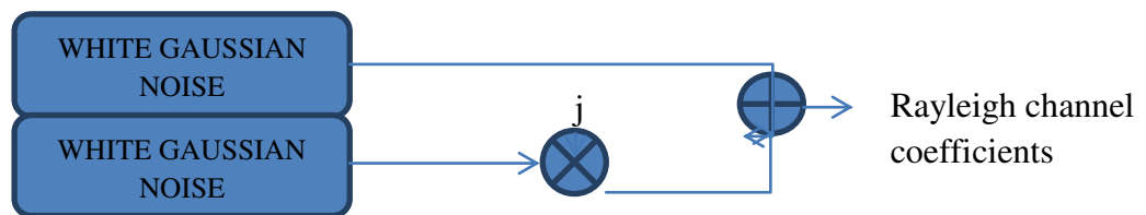
Figure 2.3 Rayleigh fading simulator
