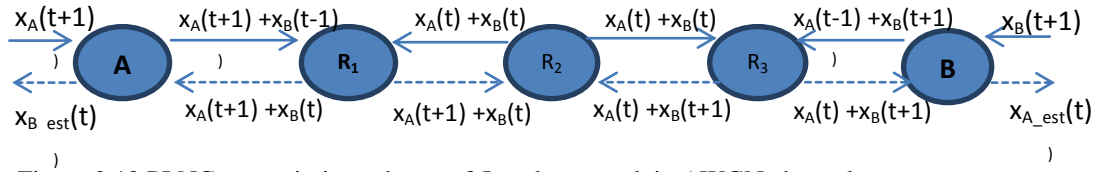
Figure 3.12 PLNC transmission scheme of 5-node network in AWGN channel
