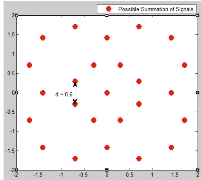
Figure 4.2 Possible summation of QPSK and 8-PSK signals
