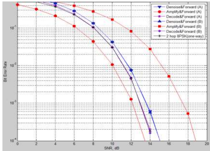
Figure 4.5 SER performance of transmission schedule 1 in AWGN channel
