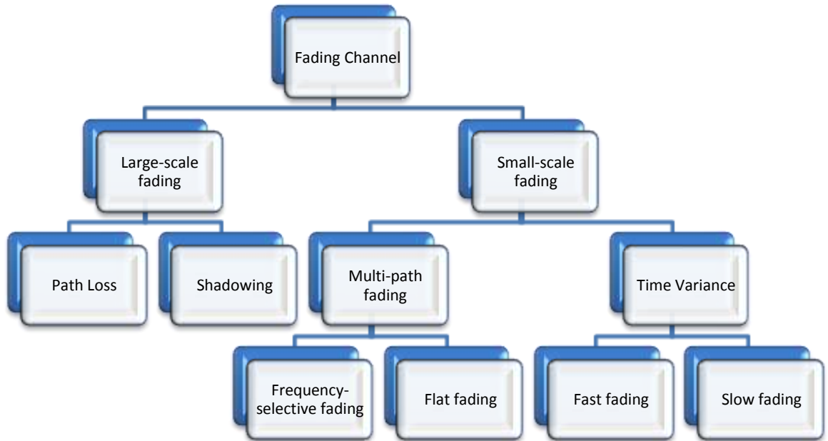
Figure 2.1 Classification of fading channels
