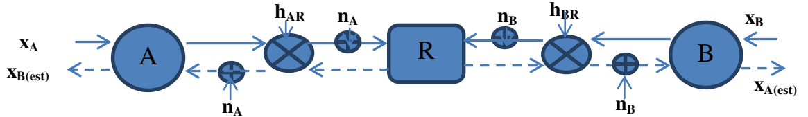
Figure 3.4 Physical layer network coding for the Alice-Relay-Bob model
