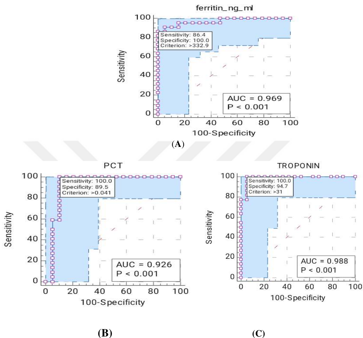
Figure 4.4. The ROC curves of (A) FER, (B) PCT and (C) cTnI in COVID-19 patients.
