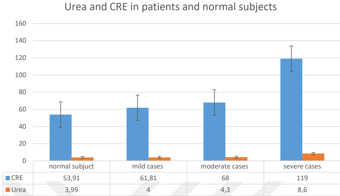
Figure 4.7. The Level of Urea and CRE in patients' groups with COVID-19 and control group.
