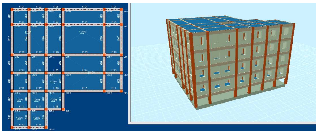
Figure 27: Torsional irregularity
