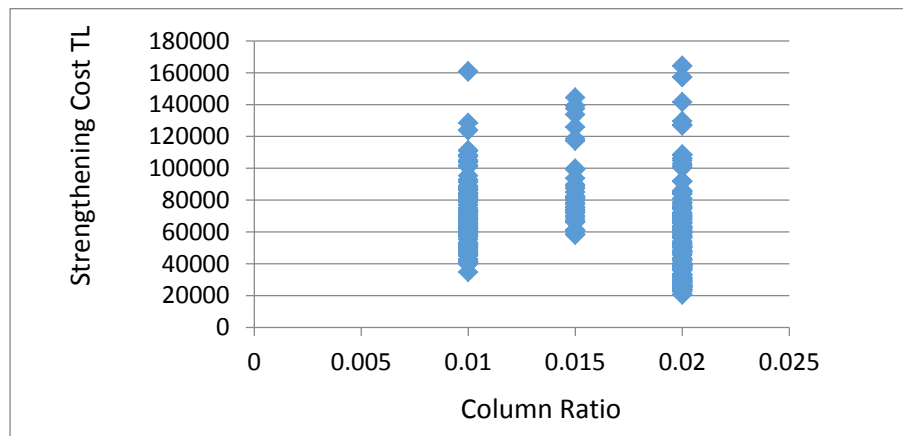
Figure 39: The effect of column ratio on strengthening cost
