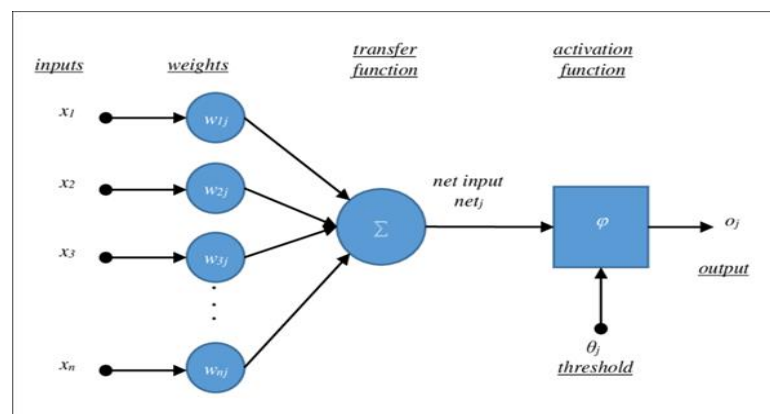
Figure 2: The Artificial Neural cell model [25]
