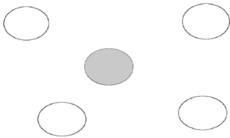
Figure 8 Centralized Algorithm
