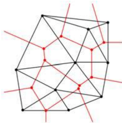
Figure 3 Delaunay triangulation
