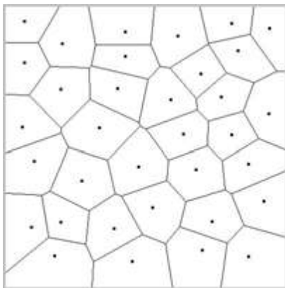
Figure 2 Voronoi diagram
