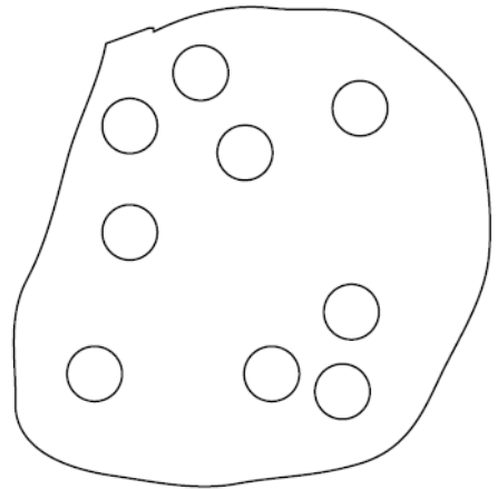
Figure 5 Random Placement
