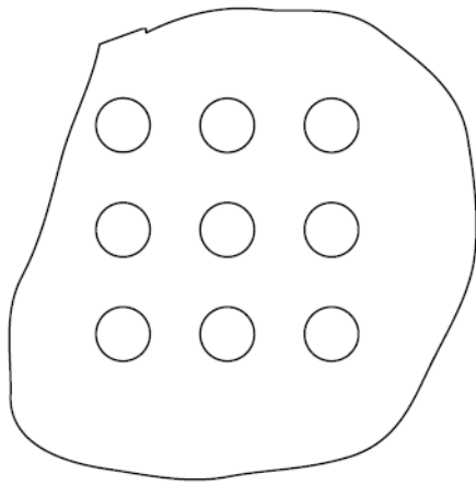
Figure 4 Deterministic Placement
