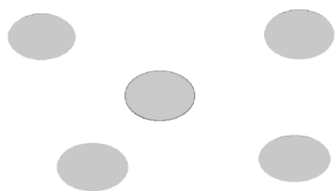
Figure 9 Distributed Algorithm
