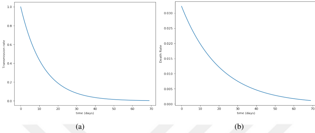
Figure 5.12: Estimation of the (a) transmission rate and (b) death rate for Spain.
