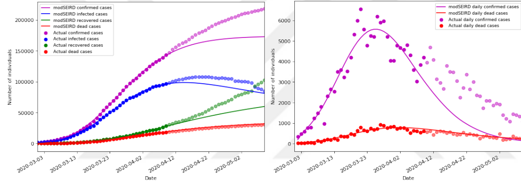
(c) Simulations for confirmed, infected, recovered and dead cases using 40 days training data. (d) Simulations for daily confirmed and dead cases using 40 days training data.
