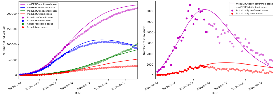
(a) Simulations for confirmed, infected, recovered and dead cases using 30 days training data. (b) Simulations for daily confirmed and dead cases using 30 days training data.
