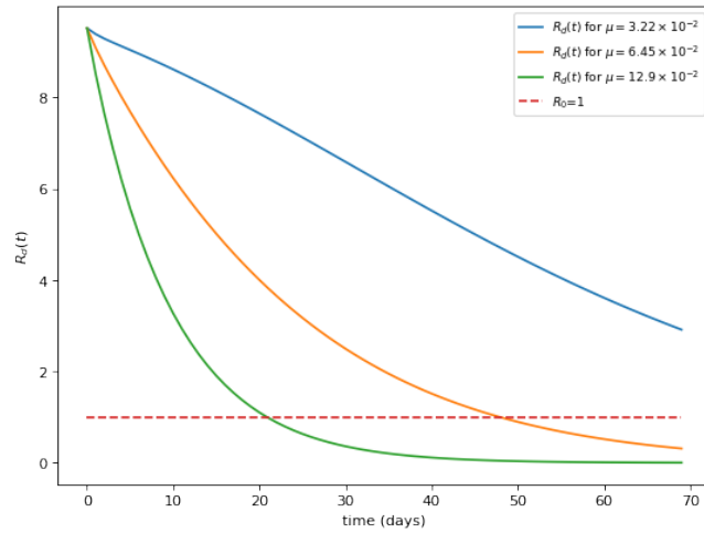
Figure 5.5: \mathcal{R}_d(t) estimation for different values of \mu in Italy by taking other parameter values of the model to be optimal.
