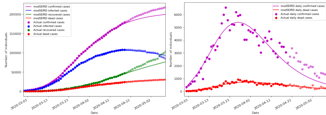
(e) Simulations for confirmed, infected, recovered and dead cases using 50 days training data. (f) Simulations for daily confirmed and dead cases using 50 days training data.
