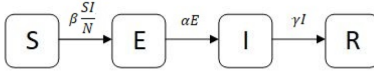
Figure 2.2: The SEIR Model.
