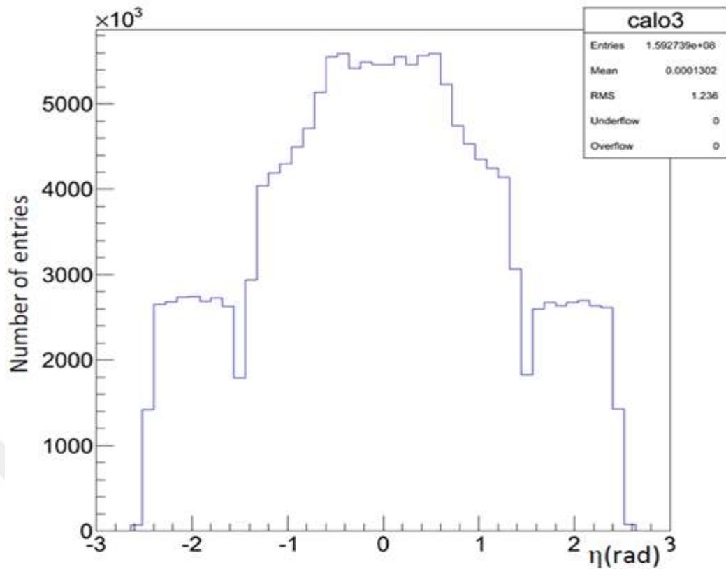
Figure 5.2 Eta ( \eta ) value distribution of photon reconstructed form electron and positron pairs for conversions vector
