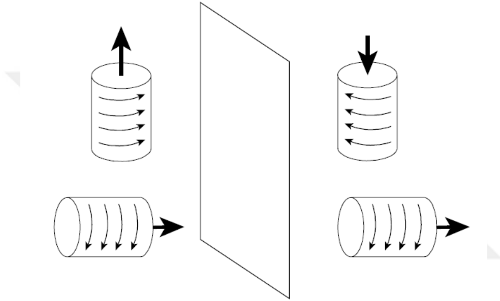
Figure 2.1 Mirror reflection of axial vectors
