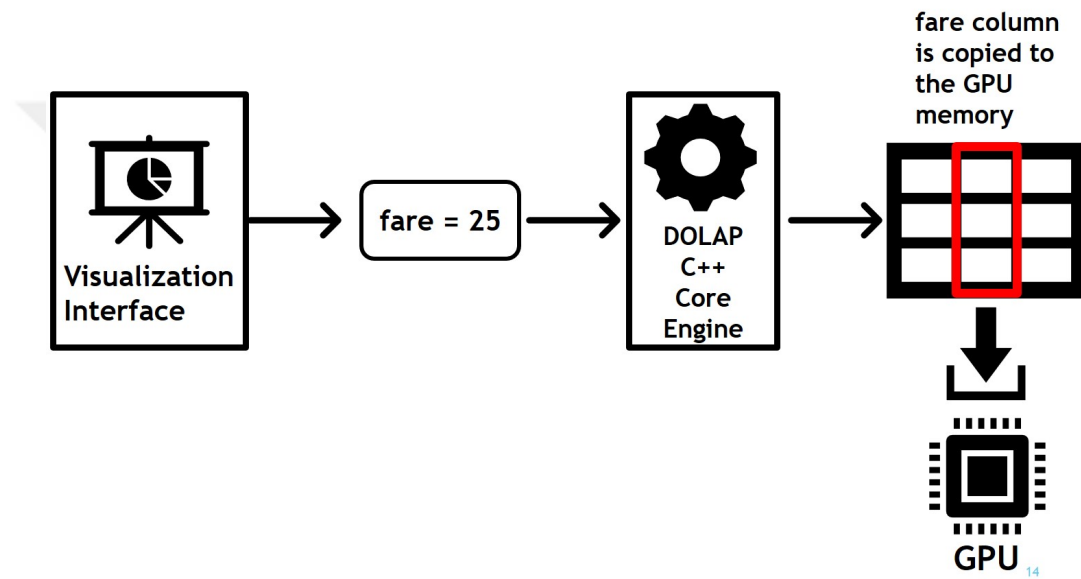
Figure 5.8 Answering Query Type 2 on GPU
