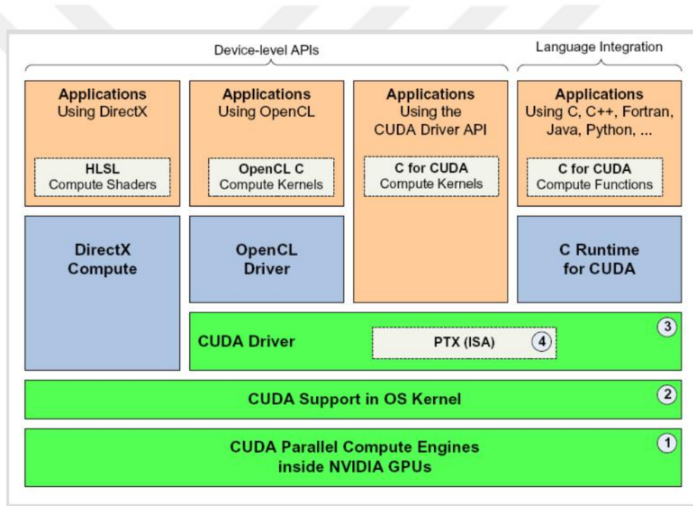
Figure 4.9 CUDA Software Architecture
