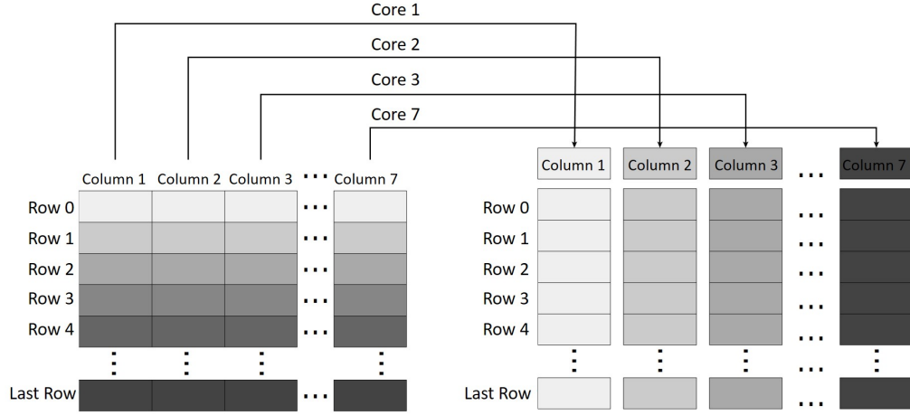
Figure 5.3 DOLAP data loading in column format
