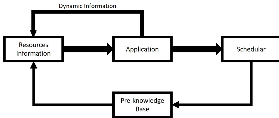
Figure 4.17 Dynamic Load Balancing
