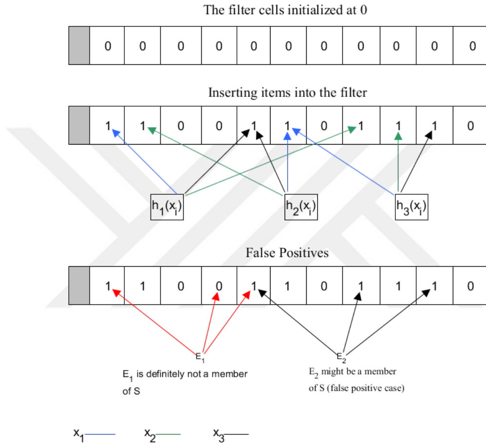
Figure 5.5 Bloom Filter
