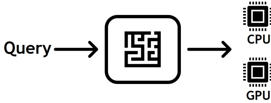
Figure 6.3 Algorithm-Based Method
