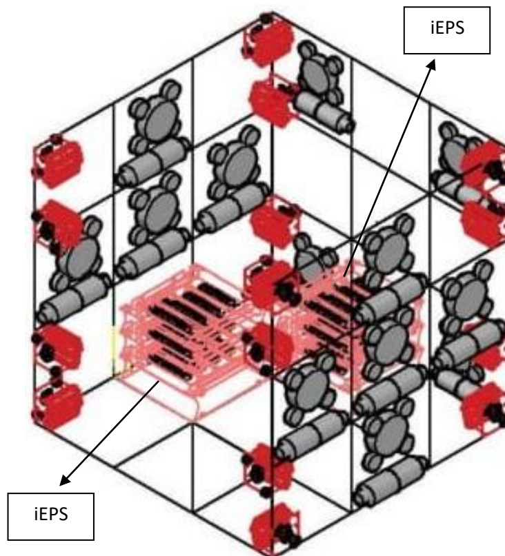
FIGURE 13. 56 iEPS CONFIGURATION OF THE WIDESAT-2
