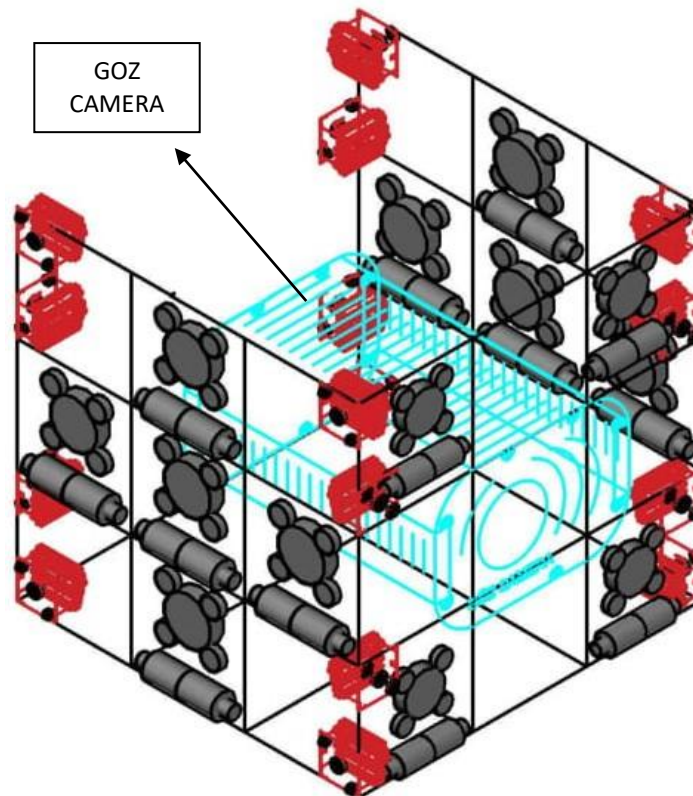
FIGURE 13. 53 GOZ CAMERA CONFIGURATION OF THE WIDESAT-3
