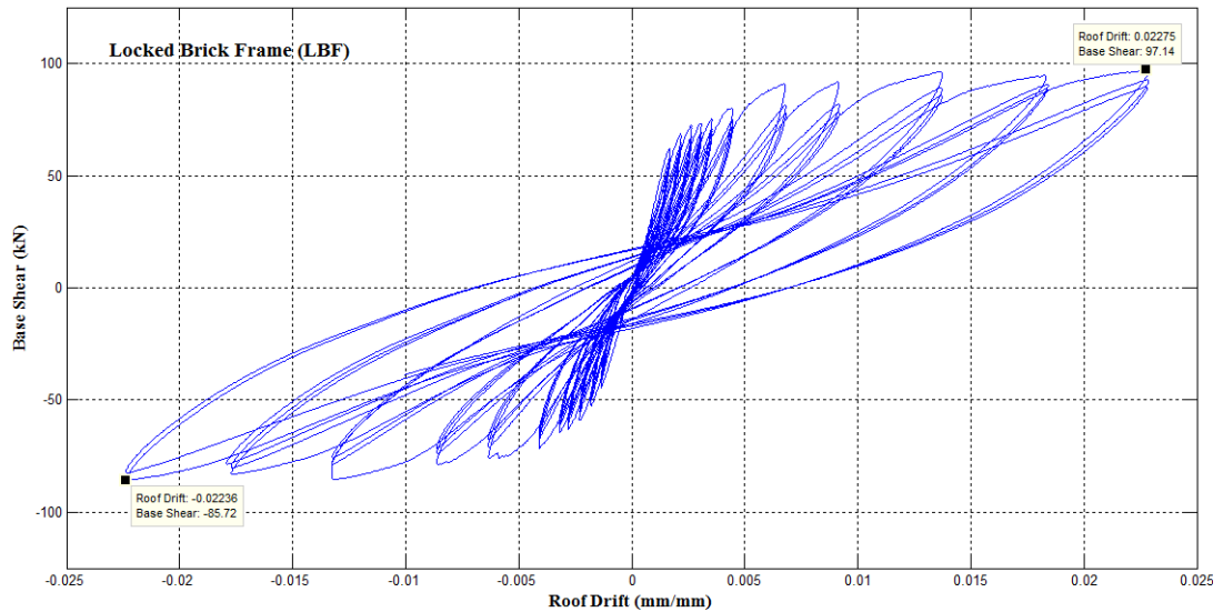
Figure 4.5 Base shear – top drift diagram for locked brick infilled frame
