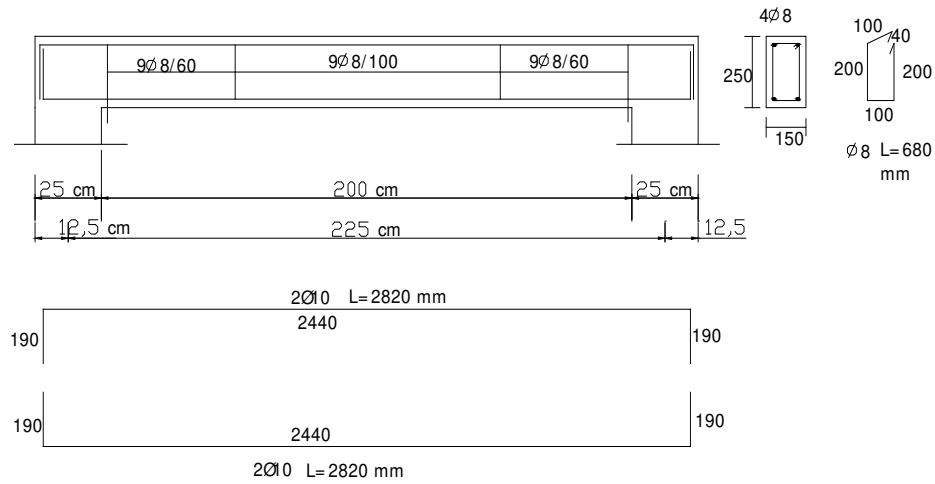
Figure 3.5 Detailing of beam reinforcements
