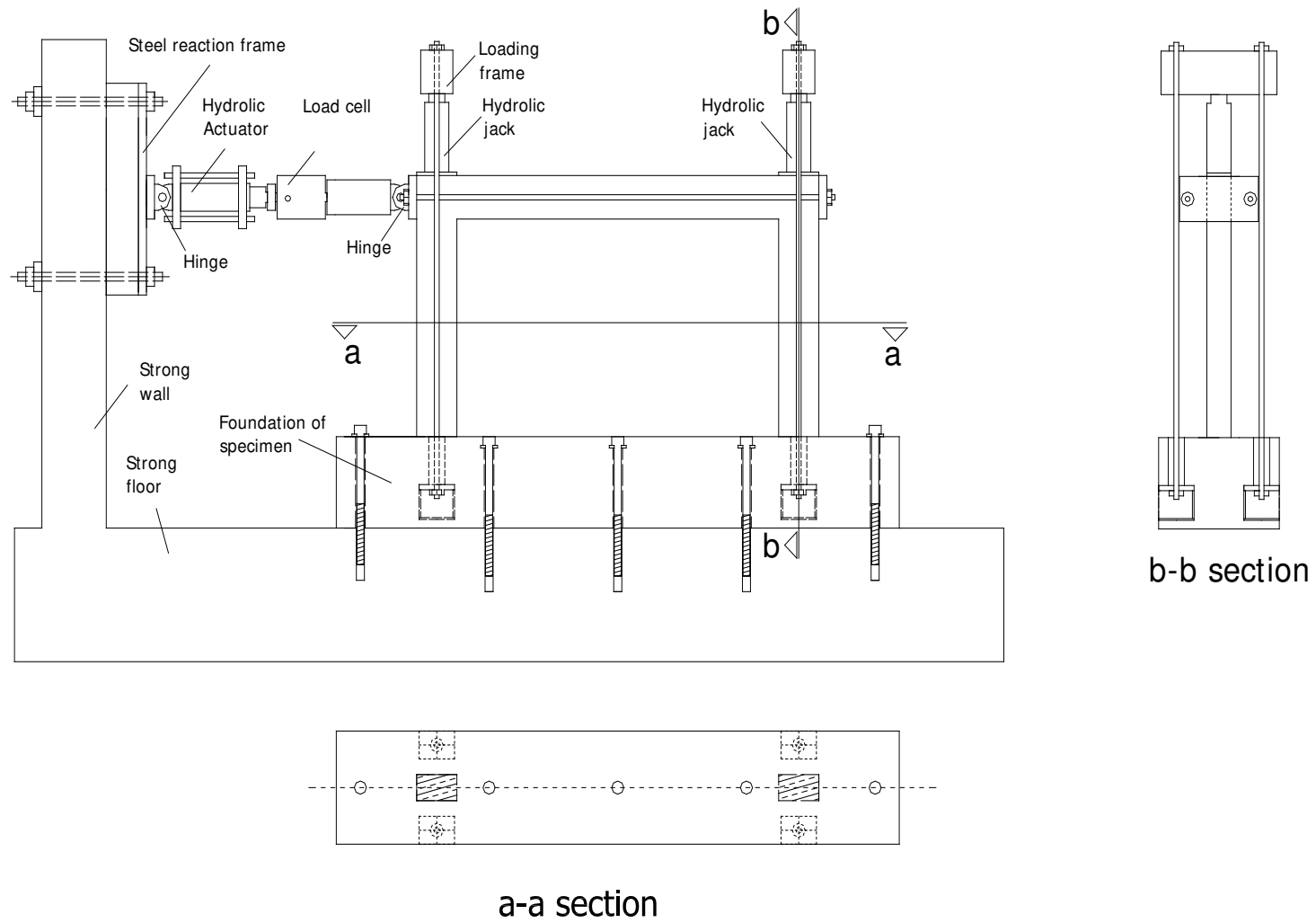
Figure 3.1 Test set-up
