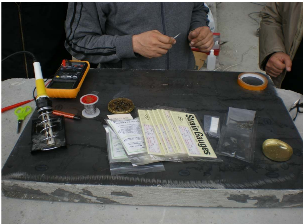
Figure 3.17 Soldering
