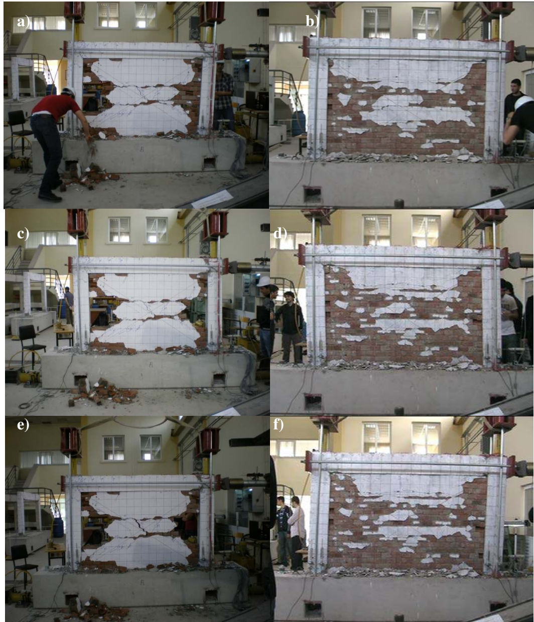
Figure 4.13 Observed damages at specific levels of drift ratio: a) Locked brick frame at -3% drift, b) Standard brick frame at -3% drift, c) Locked brick frame at 3.5% drift, d) Standard brick frame at 3.5% drift, e) Locked brick frame at -3.5% drift, f) Standard brick frame at -3.5% drift
