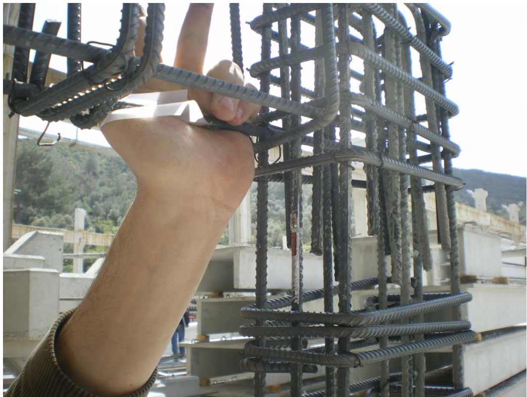
Figure 3.19 Application of pressure
