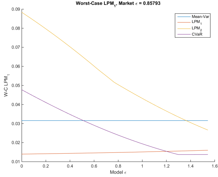
Figure 7.19: Worst-case LPM_1 measures. Low-risk Setting. H = 4.29 , r_{mv} = 0.45 , r = 0.35 , d = 0.40 .
