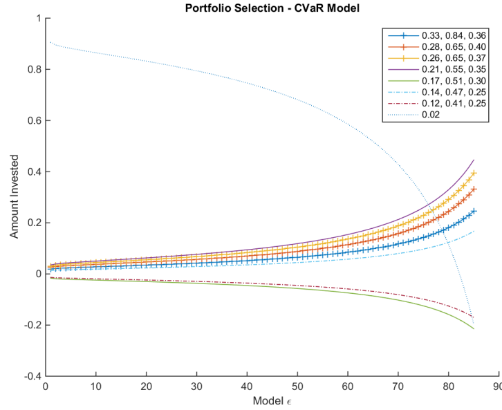
Figure 7.6: Portfolio Selection for the CVaR Model. High-risk Setting. Legend shows return mean, standard deviation and Sharpe-ratio for each single risky asset; return rate for the riskless asset. H = 0.493 , r_{mv} = 0.12 , r = 0.25 , d = 0.07 .
