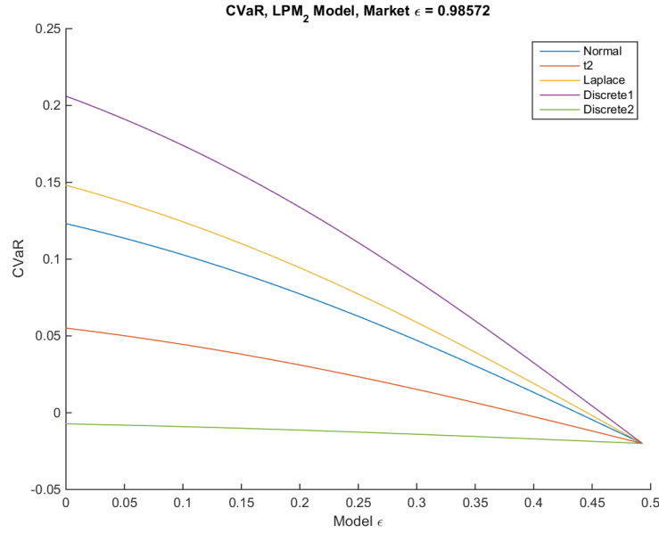
Figure 7.23: CVaR Risk Measures for Return Distributions Based on LPM 2 Model Solution and Different Distribution Types. High-risk Setting. H = 0.493 , r_{mv} = 0.12 , r = 0.25 , d = 0.07 .
