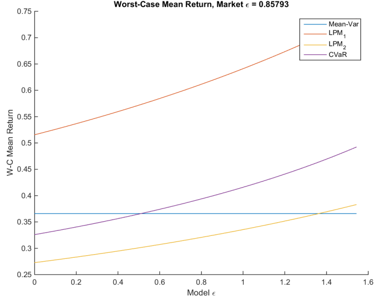
Figure 7.17: Worst-case Expected Portfolio Return. Low-risk Setting. H = 4.29 , r_{mv} = 0.45 , r = 0.35 , d = 0.40 .
