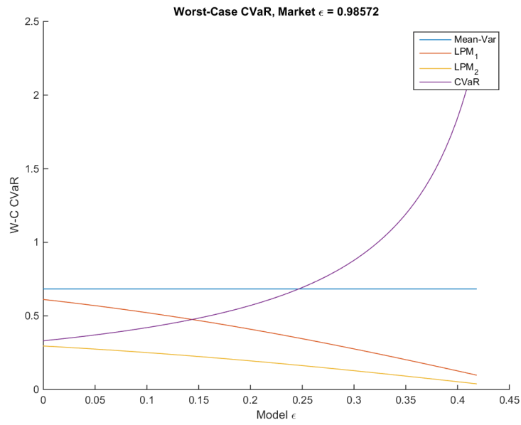
Figure 7.13: Worst-case CVaR measures. High-risk Setting. H = 0.493 , r_{mv} = 0.12 , r = 0.25 , d = 0.07 .
