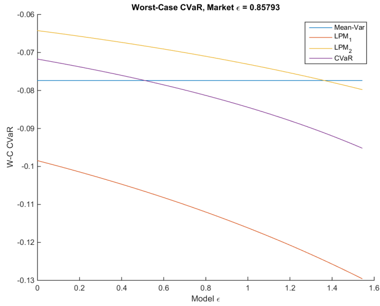
Figure 7.18: Worst-case CVaR measures. Low-risk Setting. H = 4.29 , r_{mv} = 0.45 , r = 0.35 , d = 0.40 .
