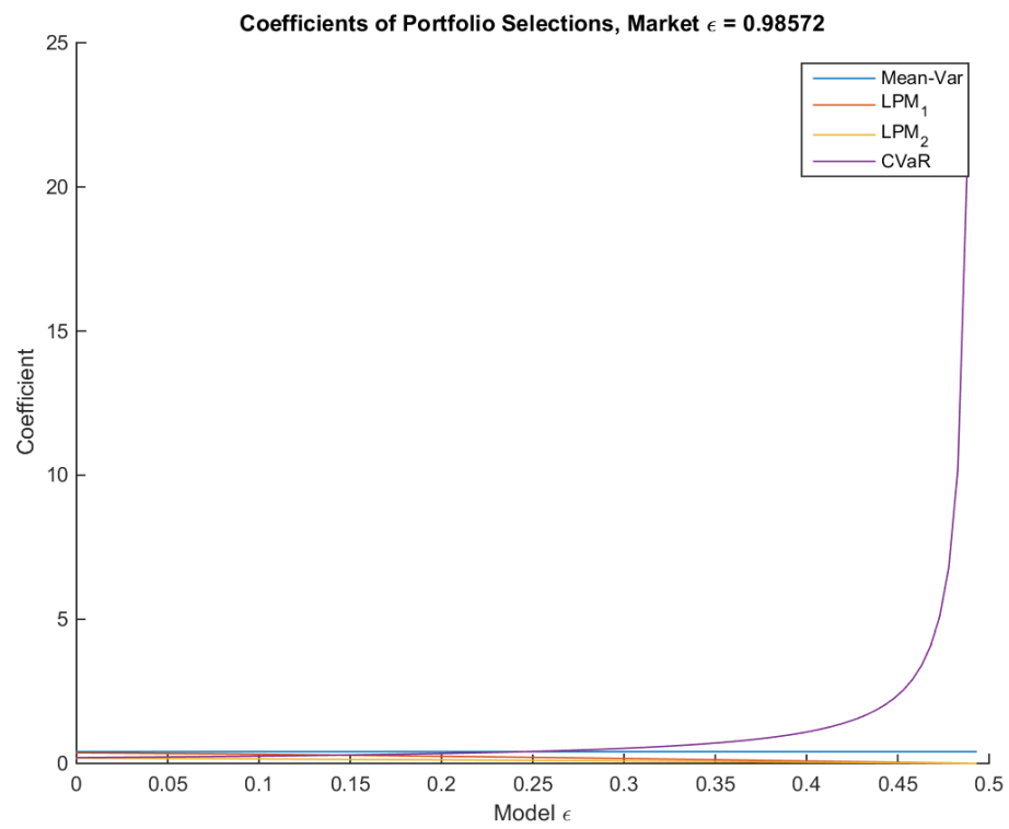
Figure 7.1: Change in Coefficients as Anticipated Mean Uncertainty Radius Increases. H = 0.493 , r_{mv} = 0.12 , r = 0.25 , d = 0.07 .
