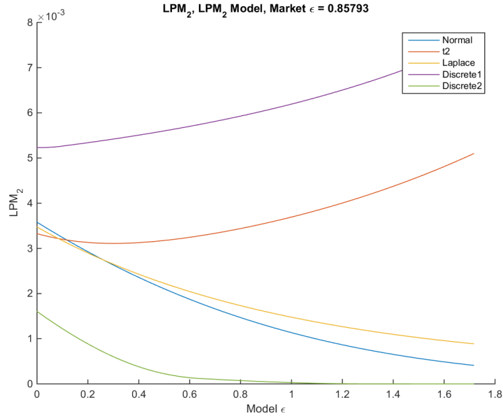
Figure 7.25: LPM_2 Risk Measures for Return Distributions Based on LPM_2 Model Solution and Different Distribution Types. Low-risk Setting. H = 4.29 , r_{mv} = 0.45 , r = 0.35 , d = 0.40 .
