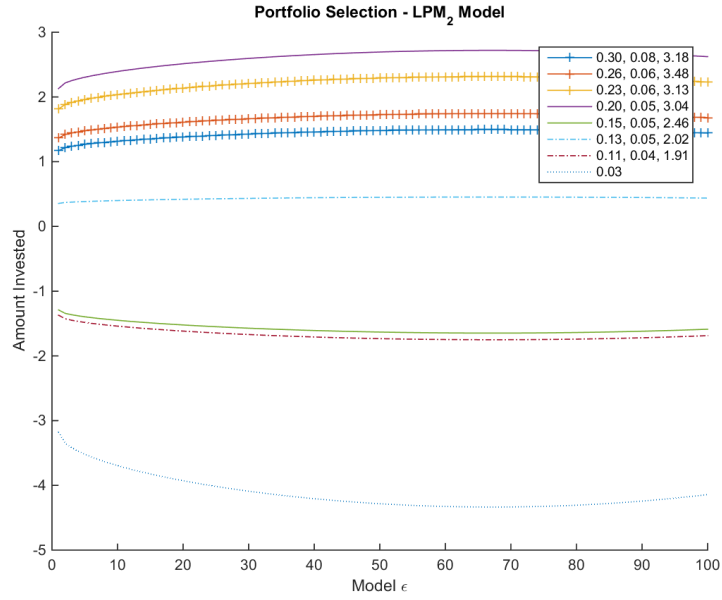
Figure 7.8: Portfolio Selection for the LPM_2 Model. Low-risk Setting. Legend shows return mean, standard deviation and Sharpe-ratio for each single risky asset; return rate for the riskless asset. H = 4.29 , r_{mv} = 0.45 , r = 0.35 , d = 0.40 .
