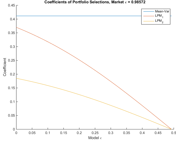
Figure 7.2: Change in Coefficients as Anticipated Mean Uncertainty Radius Increases, without the CVaR model. H = 0.493 , r_{mv} = 0.12 , r = 0.25 , d = 0.07 .
