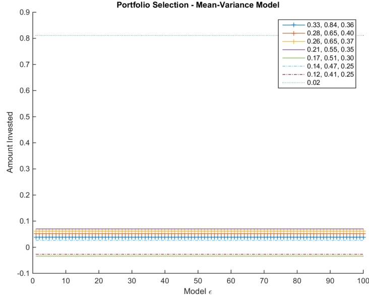
Figure 7.3: Portfolio Selection for the Mean-Variance Model. High-risk Setting. Constant over x-axis since the model does not involve mean return vector uncertainty. Legend shows return mean, standard deviation and Sharpe-ratio for each single risky asset; return rate for the riskless asset. H = 0.493 , r_{mv} = 0.12 , r = 0.25 , d = 0.07 .
