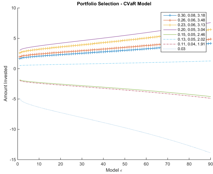
Figure 7.9: Portfolio Selection for the CVaR Model. Low-risk Setting. Legend shows return mean, standard deviation and Sharpe-ratio for each single risky asset; return rate for the riskless asset. H = 4.29 , r_{mv} = 0.45 , r = 0.35 , d = 0.40 .
