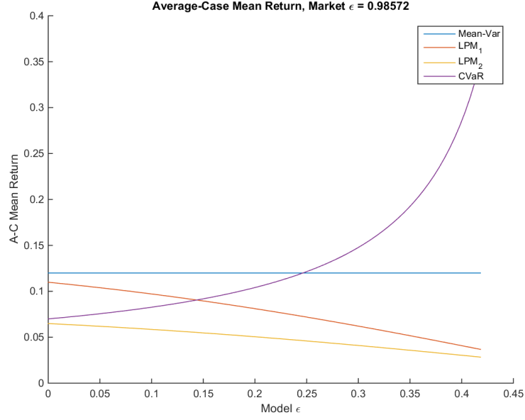
Figure 7.10: Expected Return Rate on Portfolio on an Average-Case. High-risk Setting. H = 0.493 , r_{mv} = 0.12 , r = 0.25 , d = 0.07 .
