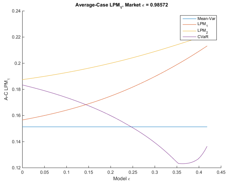
Figure 7.15: Average-case LPM_1 measures. High-risk Setting. H = 0.493 , r_{mv} = 0.12 , r = 0.25 , d = 0.07 .
