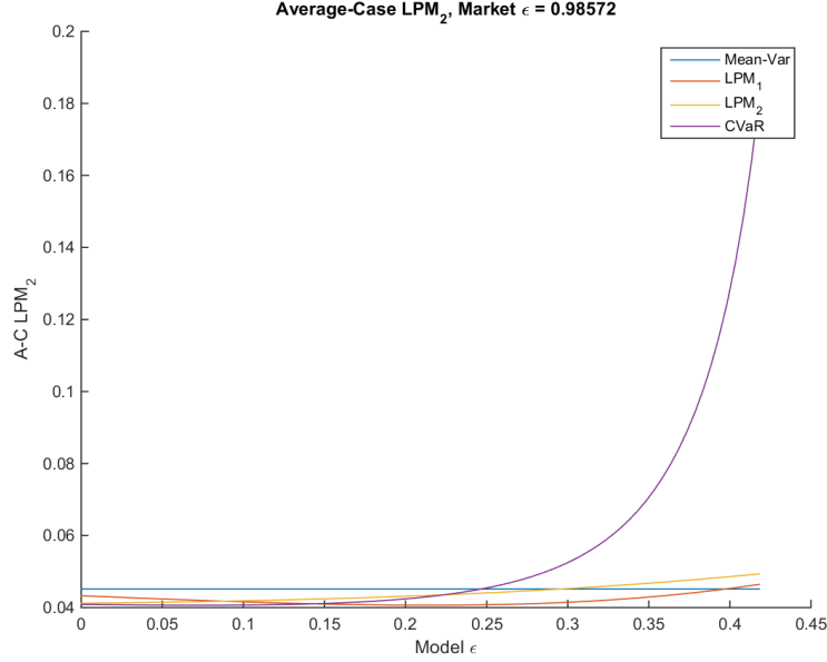
Figure 7.16: Average-case LPM_2 measures. High-risk Setting. H = 0.493 , r_{mv} = 0.12 , r = 0.25 , d = 0.07 .
