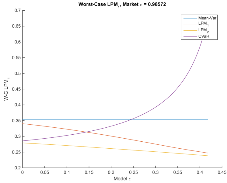
Figure 7.11: Worst-case LPM_1 measures. High-risk Setting. H = 0.493 , r_{mv} = 0.12 , r = 0.25 , d = 0.07 .
